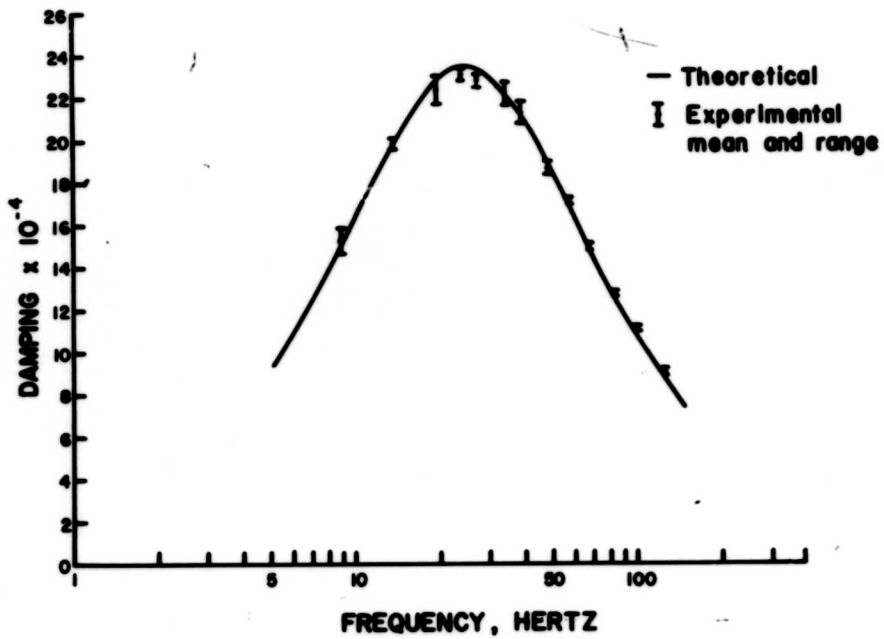
Figure 4. Damping Versus Frequency for 2024-T4 Aluminum; Theoretical and Experimental.
