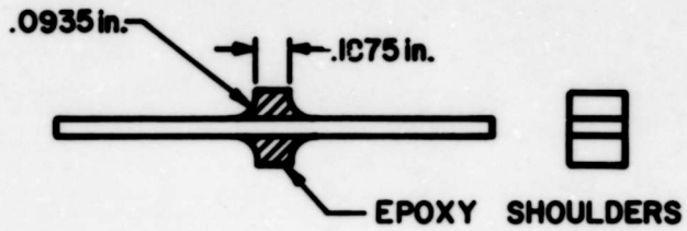
Figure 1. Forced Vibration, FRP Test Specimen Geometry.
