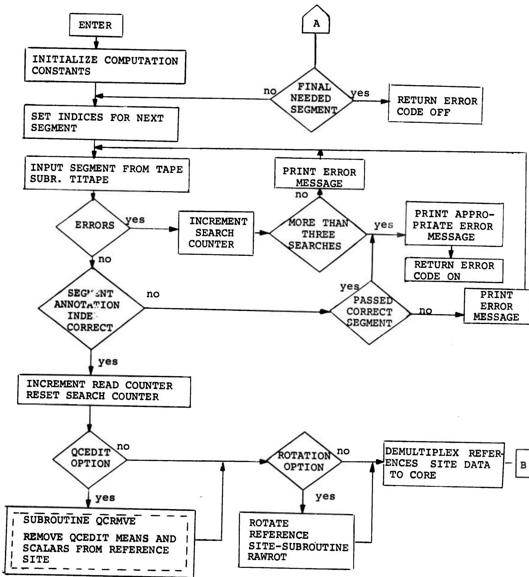
FIGURE III-16 PREPAR
