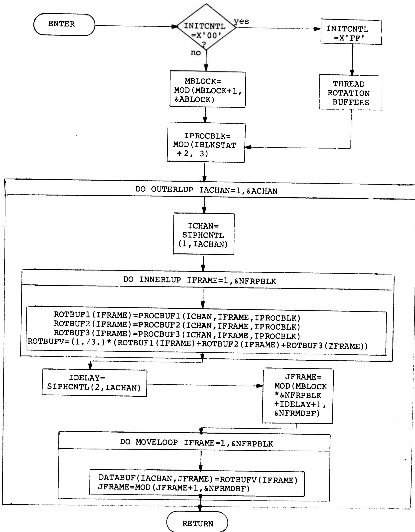
FIGURE II-2 SUBROUTINE SIPHON
