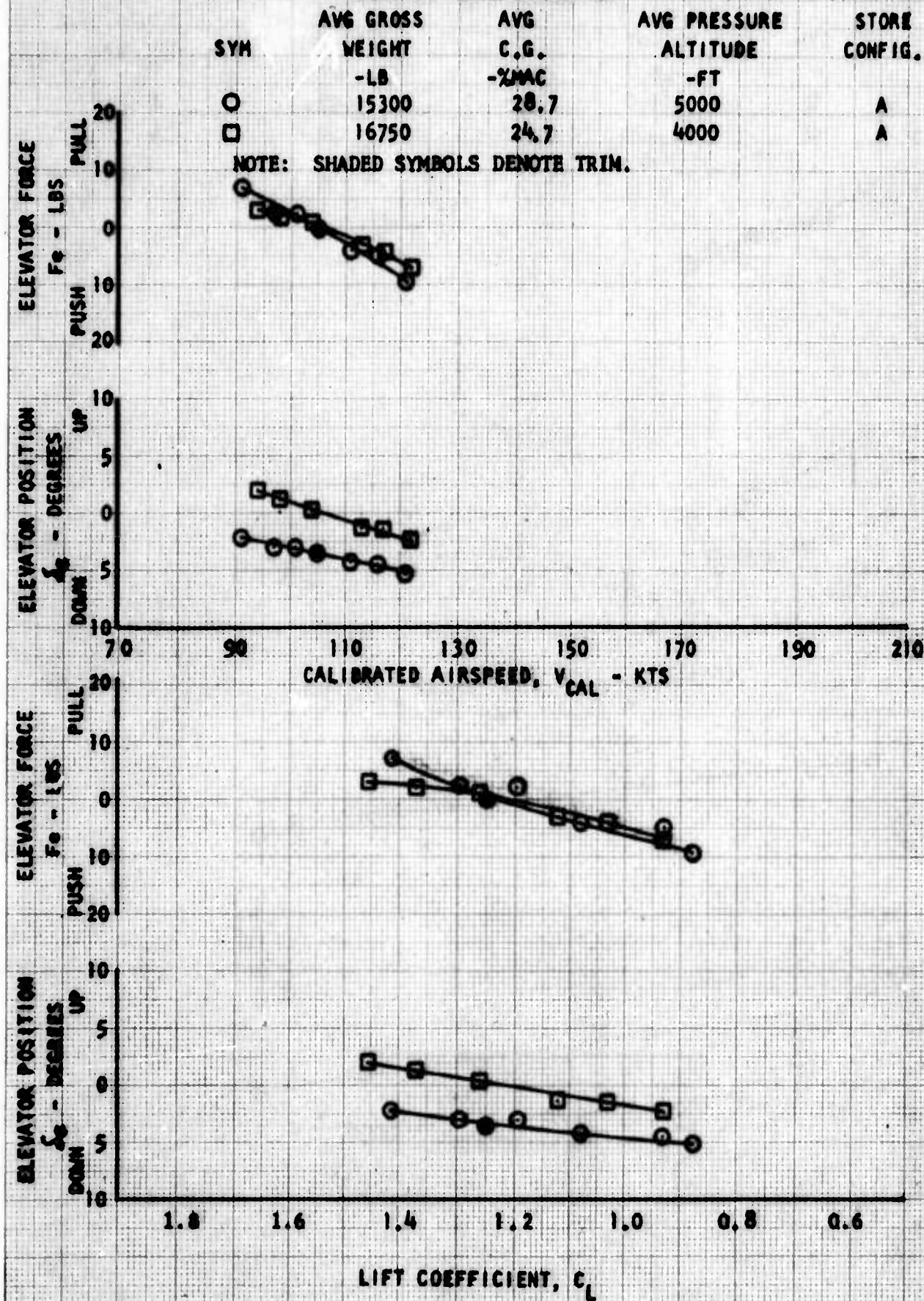
FIGURE No. 33 STATIC LONGITUDINAL STABILITY (STICK FIXED & FREE) OV-10 (PRE-PRODUCTION) USA S/N 67-18899 WAVE-OFF CONFIGURATION
