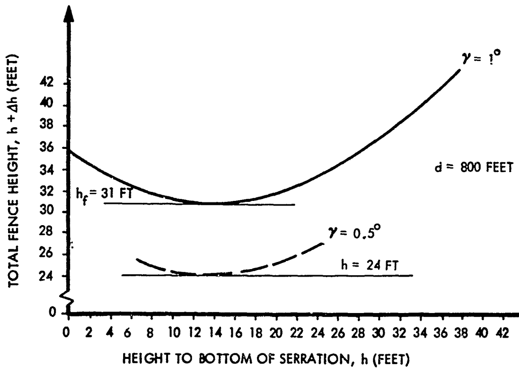
793 - 3A 1EV 1 Figure 6-3. Complex Fence Height Versus Slot Location, (Serrated Edge Type) (Refer to Figure 6-2 for Fence Geometry)
