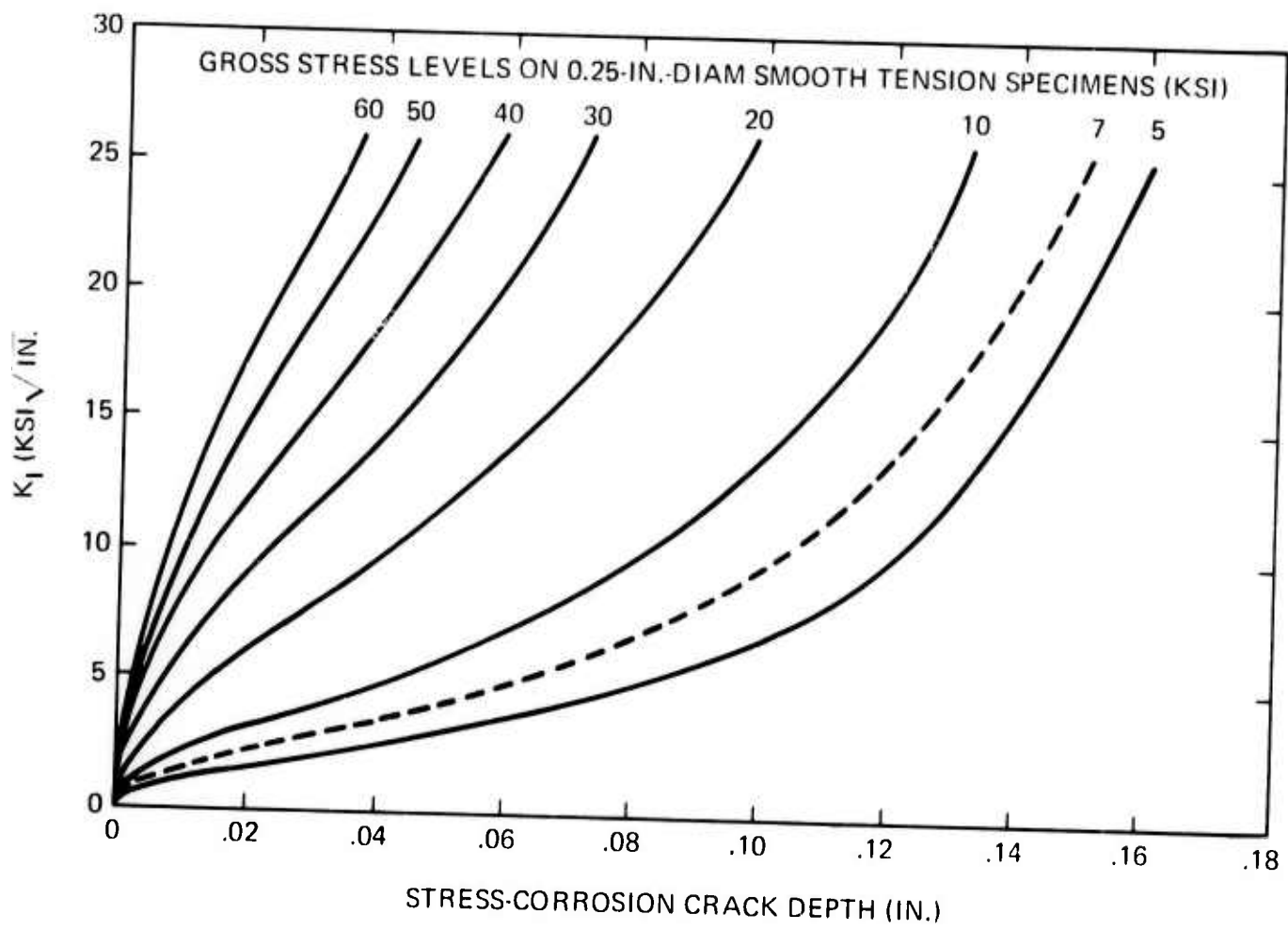
Figure 70. Approximate Stress Intensity Versus Crack Depth Curves for Single-Edge Notched Tension Specimens Loaded to Different Gross Stress Levels (From Ref. 26)
