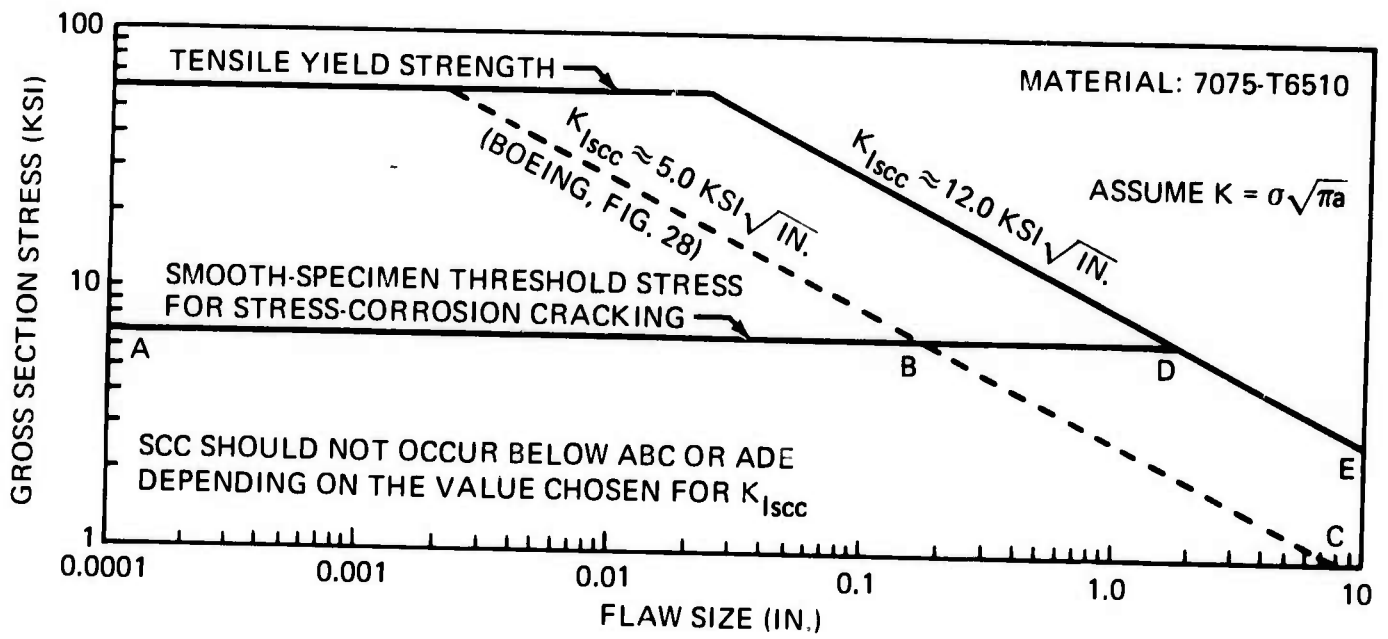
Figure 69. Suggested Method for Combining Stress-Corrosion Data on Smooth and Pre-cracked Specimens for Predicting When Stress-Corrosion Cracking Will Occur (From Ref. 44)
