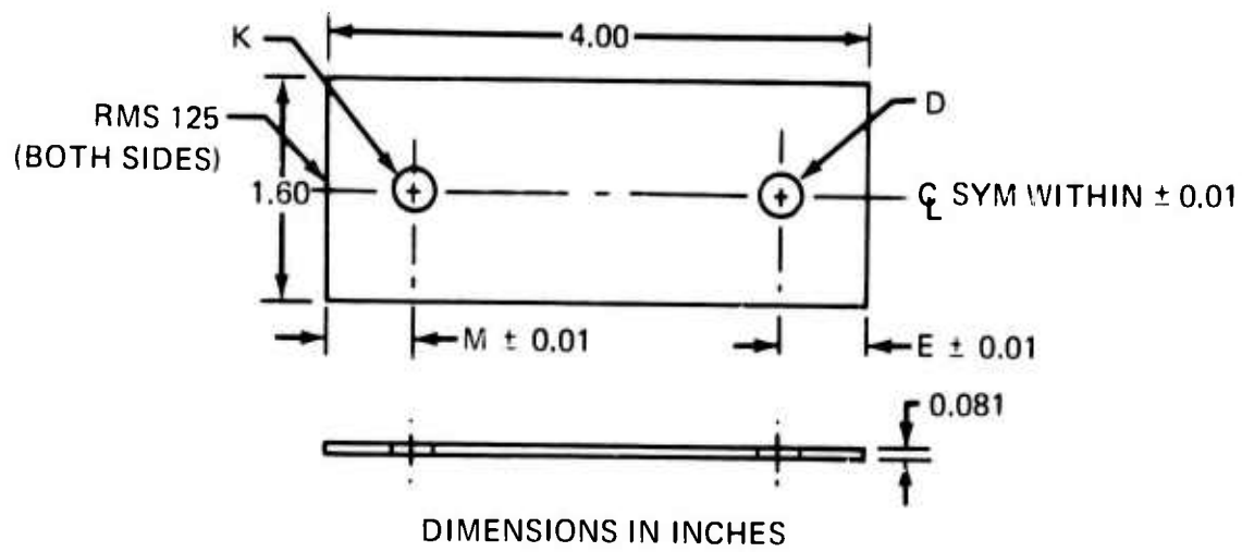
Figure 75. Bearing Specimen
