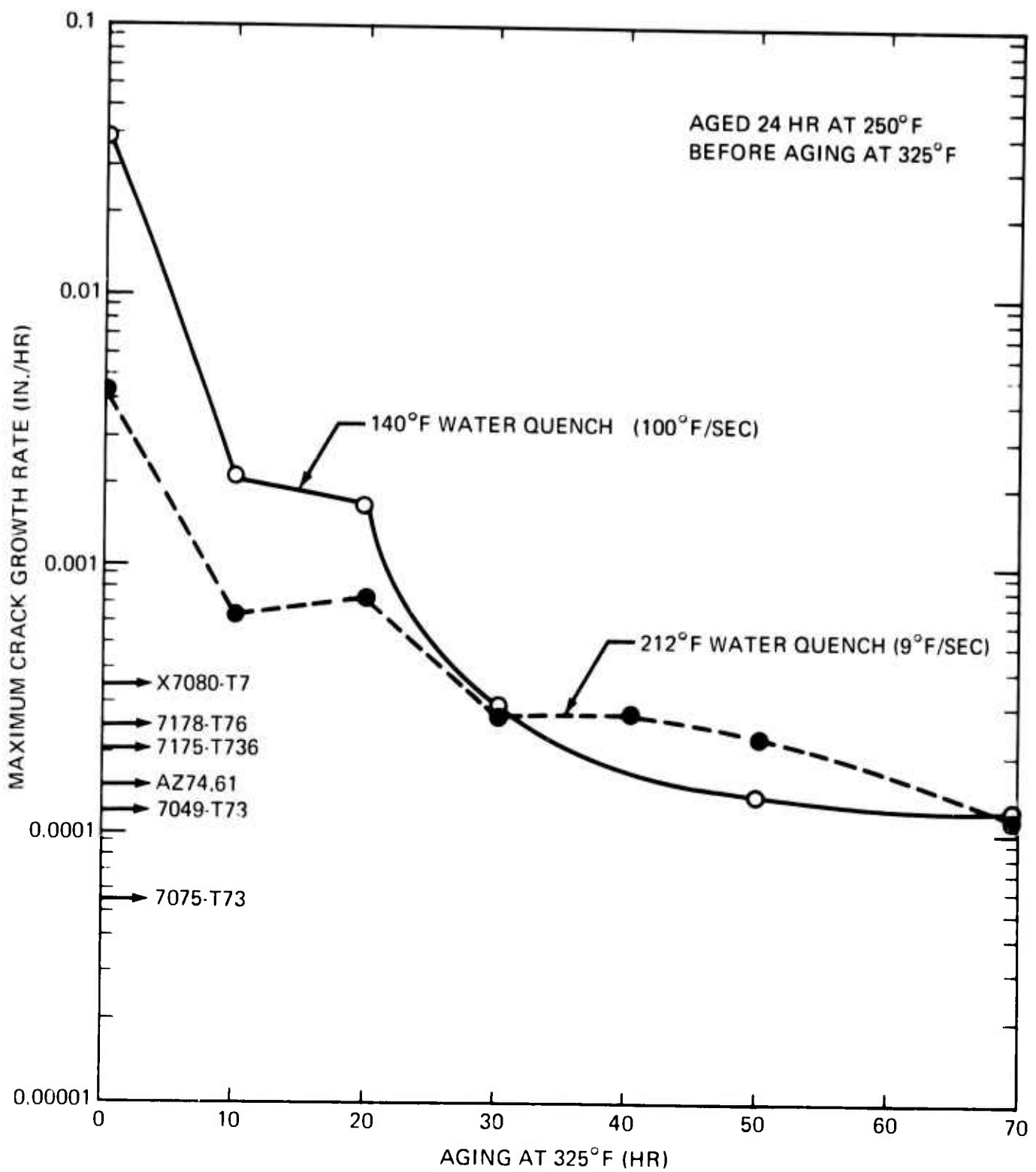
Figure 3.3 Effect of Aging Time at 325°F on the Maximum Stress-Corrosion Crack Growth Rates of Alloy 21. Maximum Crack Growth Rates for the Commercial Alloys Are from Ref. 26.
