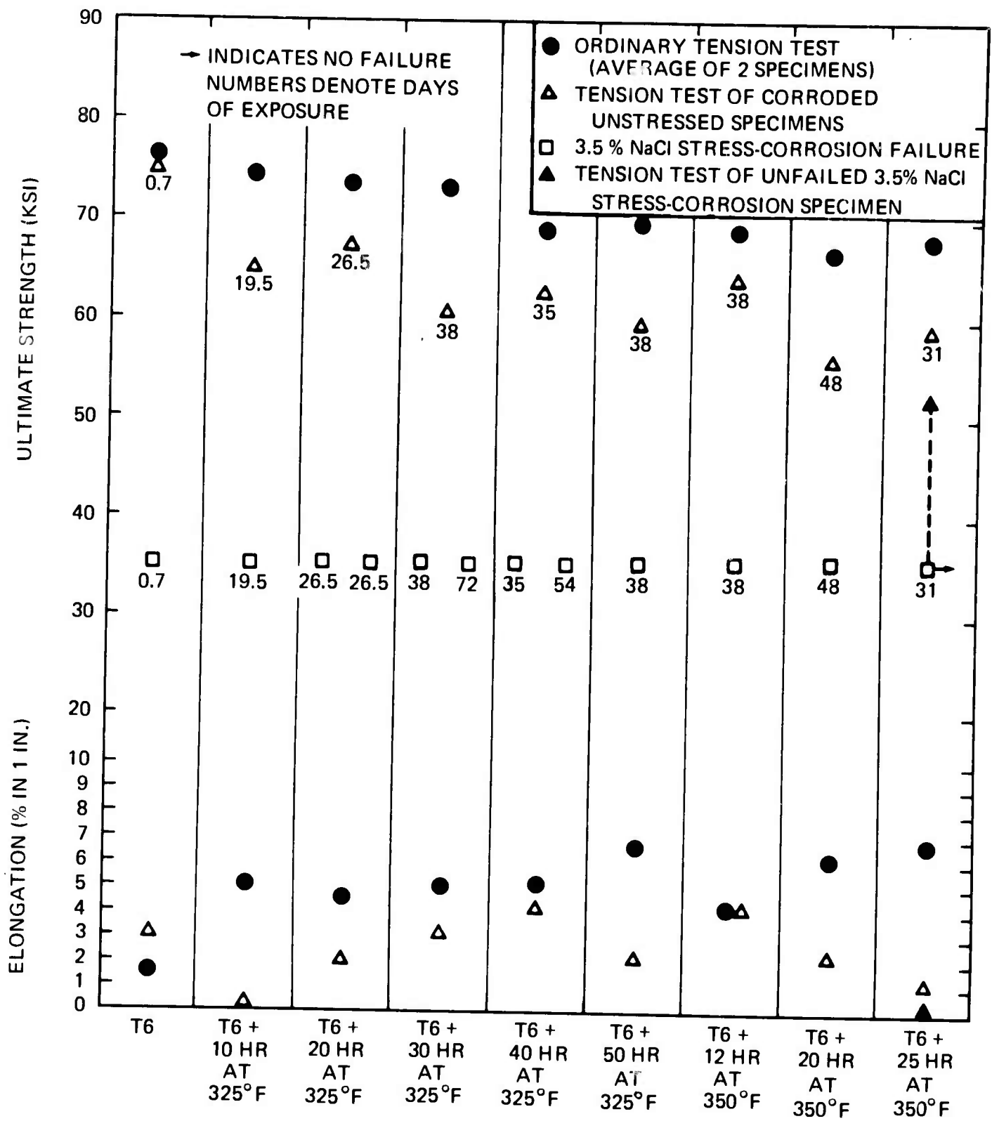
Figure 41. Effect of Corrosion and Stress-Accelerated Corrosion on Mechanical Properties of Alloy 21 in Various Heat-Treatment Conditions. Specimen Blanks Were Quenched in 212°F Water.
