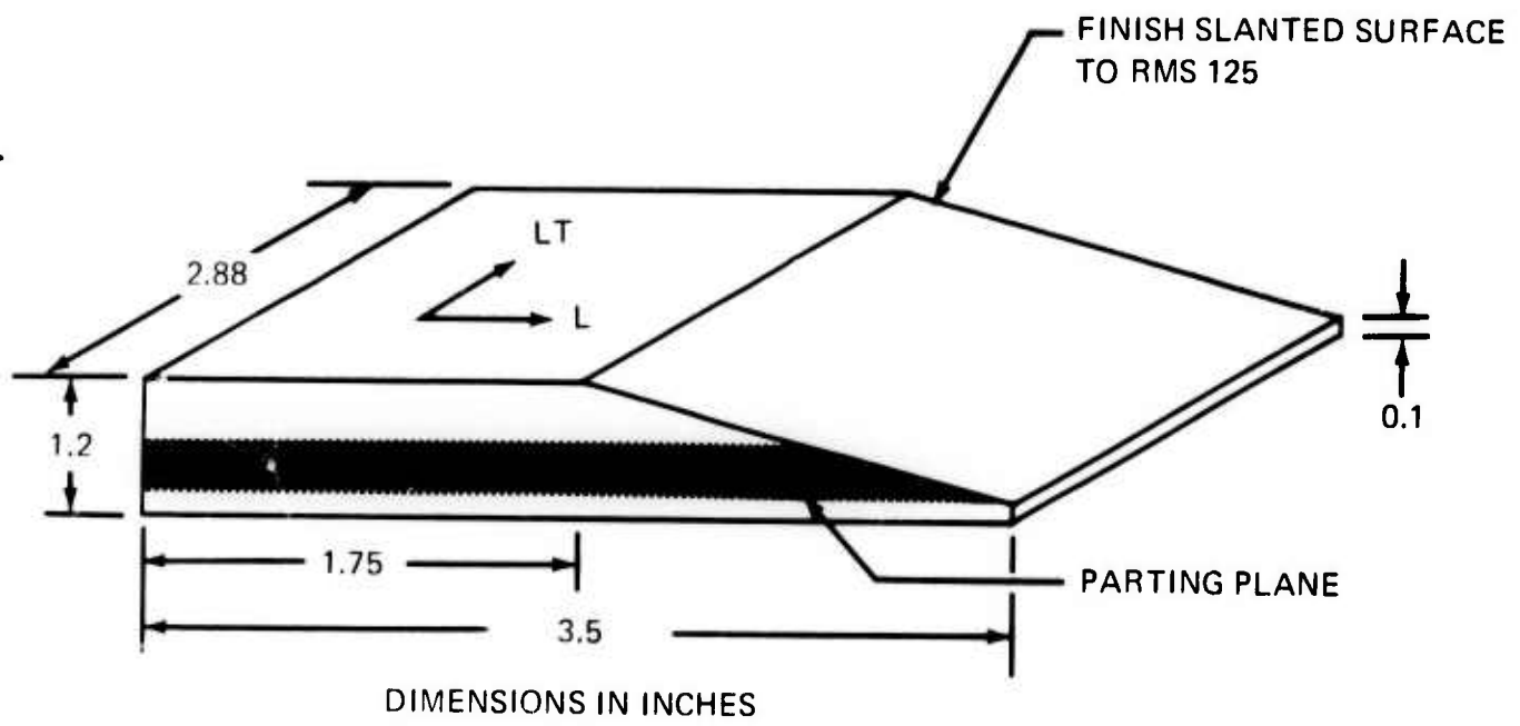
Figure S1. Exfoliation Corrosion Specimen
