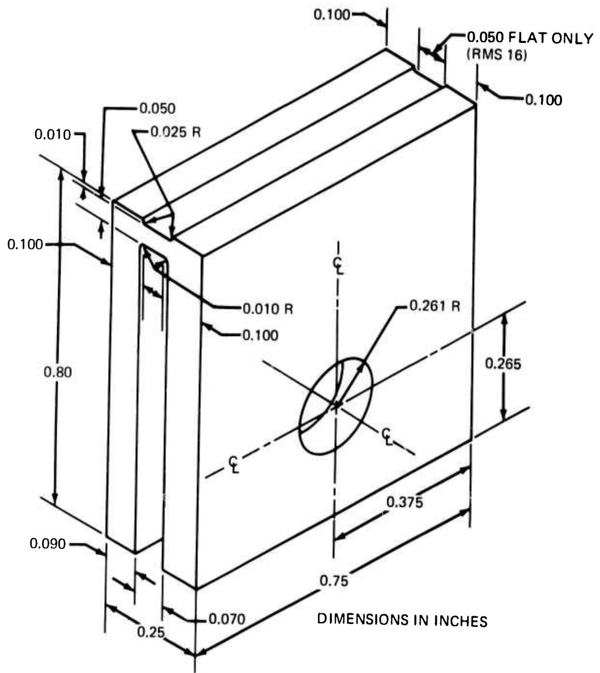
Figure 79. Battelle Tuning-Fork Type Stress-Corrosion Specimen (Ref. 45 )
