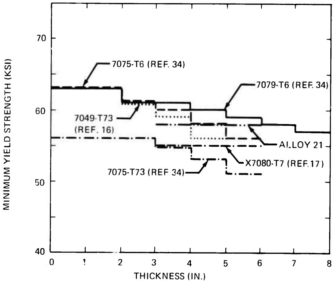
Figure 54. Minimum Longitudinal Ultimate and Yield Strength Values for Hand Forgings of Several Commercial Alloys and Alloy 21
