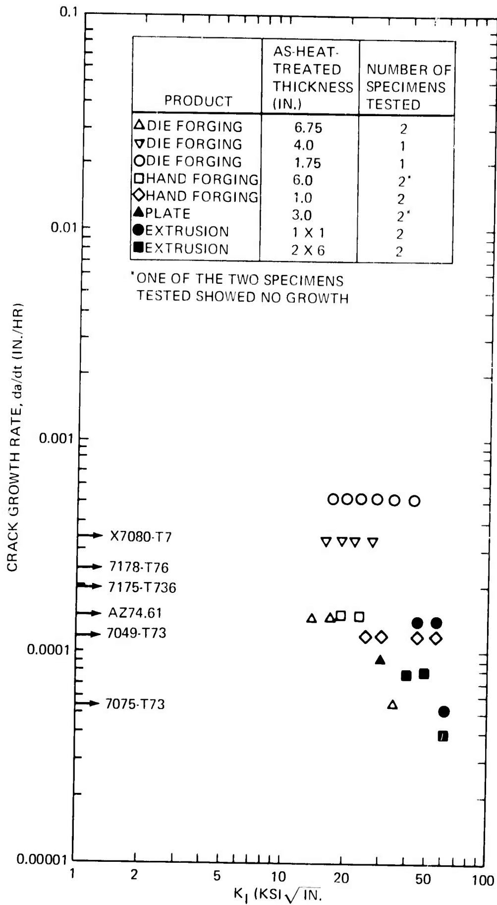
Figure 64. Stress-Corrosion Cracking Behavior of Alloy 21 Wrought Products Measured on Pre-cracked DCB Specimens Intermittently Wetted with 3.5% NaCl. All Specimens Were Machined to Test the Material in the Transverse or Short-Transverse Direction. Maximum Crack Growth Rates for the Commercial Alloys Are from Ref. 26.
