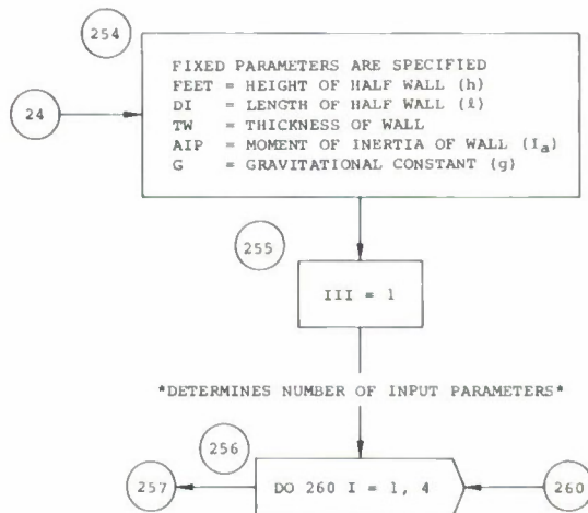
VI. OFFICE BUILDING (HALF WALL WITH WINDOWS) ANALYSIS SUBROUTINE - OHAFW
