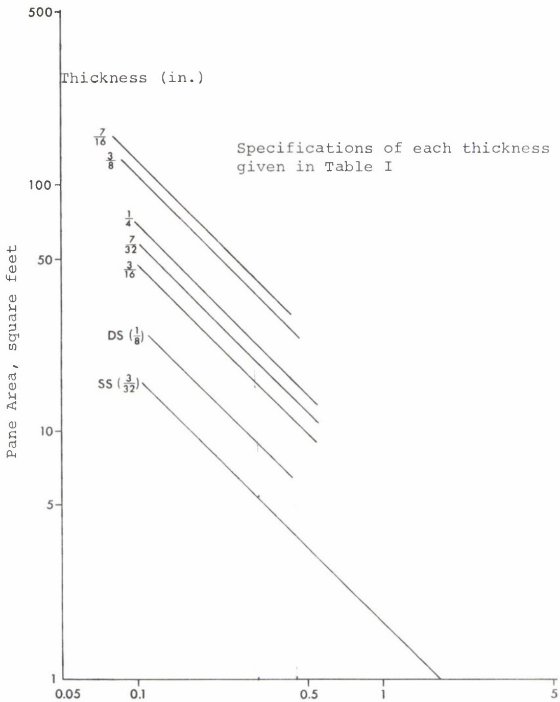
Figure 3. Sheet Glass Incipient Failure Pressures for Front-Face Loading as a Function of Pane Area and Thickness
