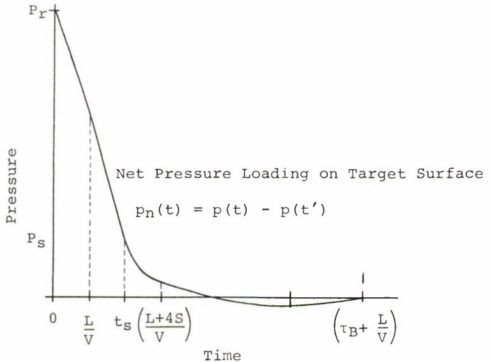
Figure 13. Net Pressure Loading Function.
