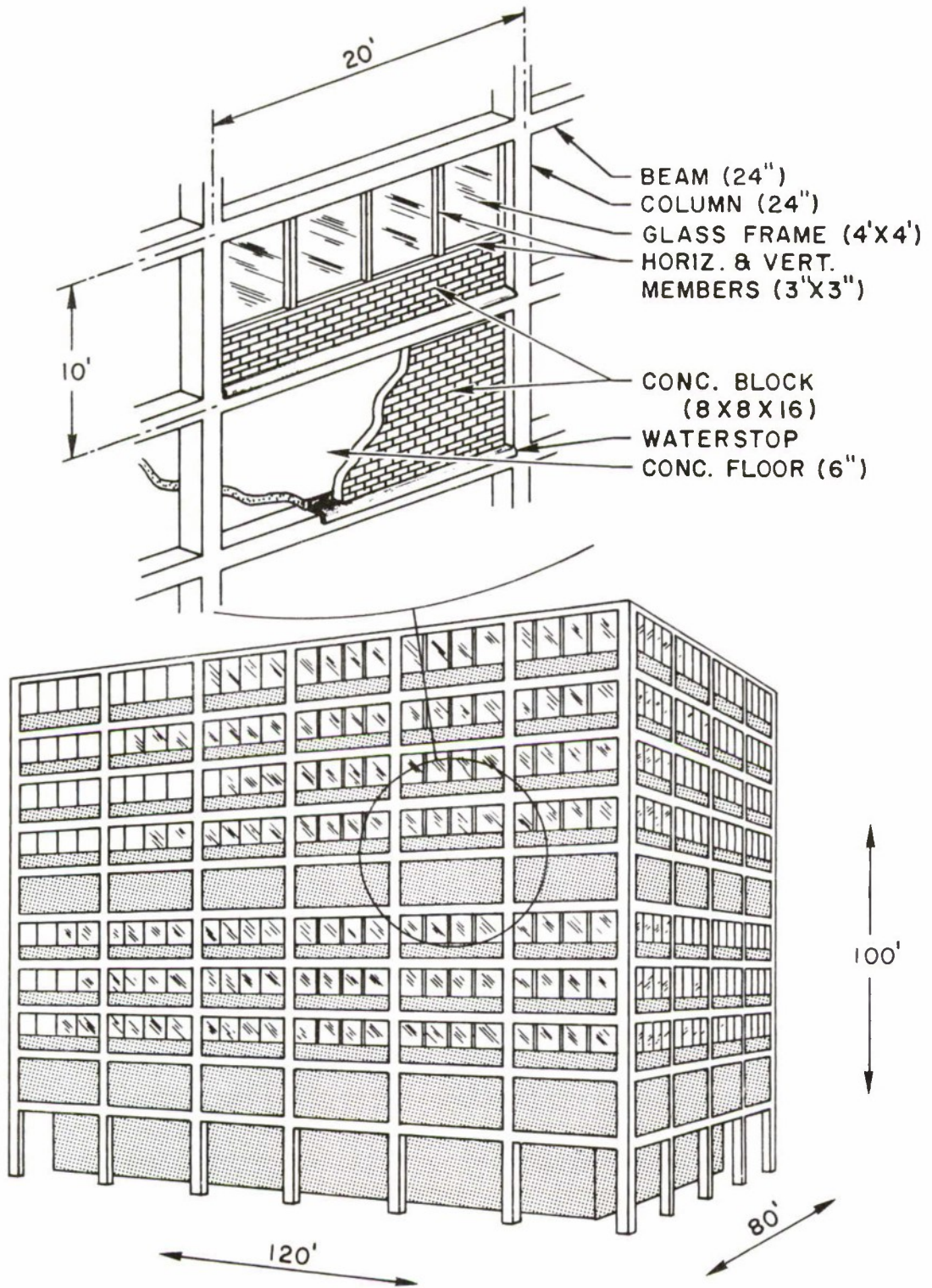
Figure 17. Multi-Story Building
