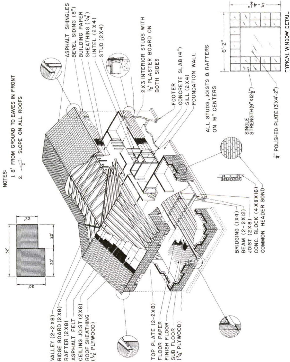
Figure 11. Split-Level House
