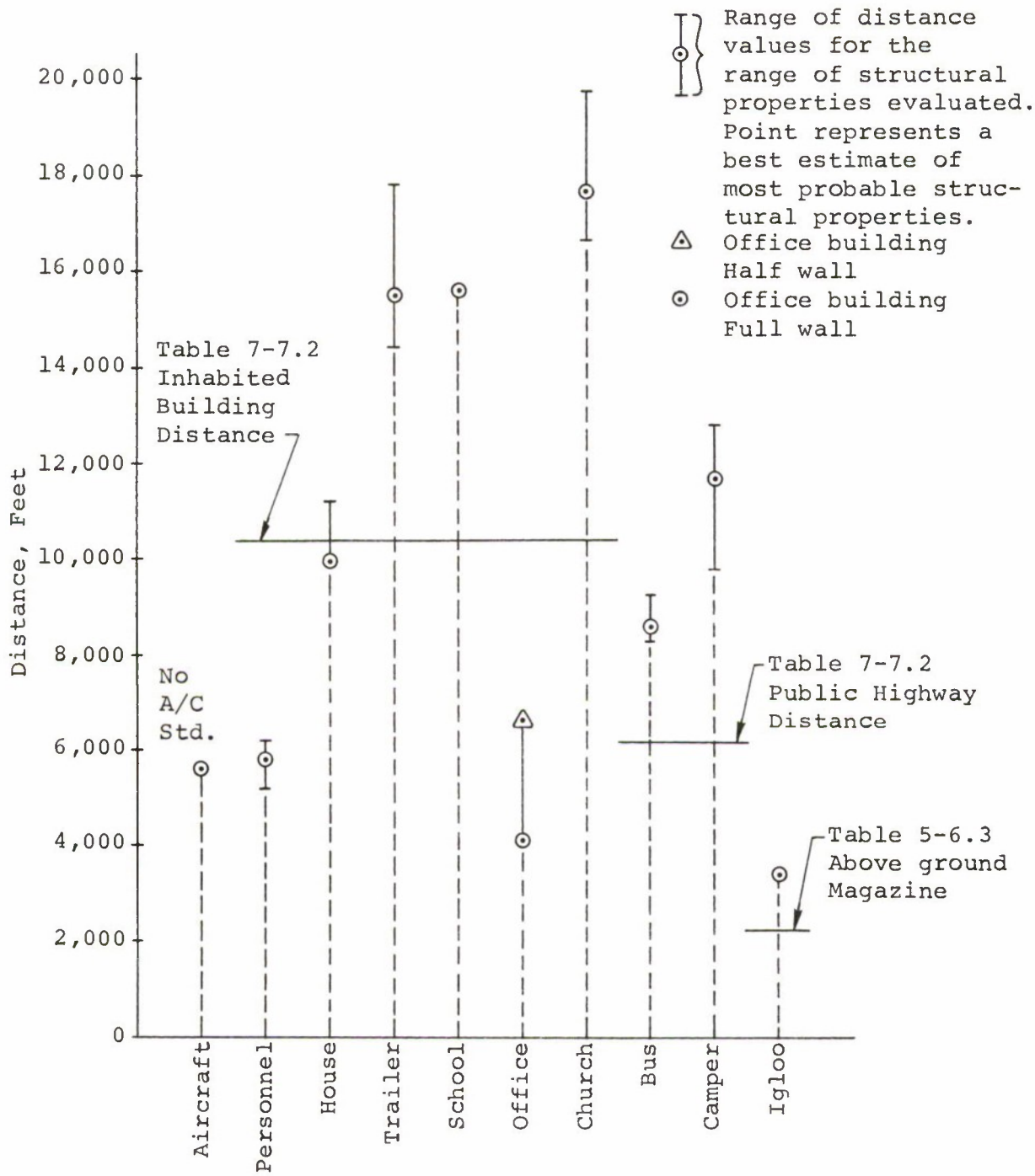
Figure 35. Computed Distance Requirements for Acceptable Damage to Targets Exposed to the Blast From 9 Million Pounds of TNT
