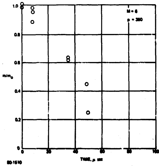
Figure 18 DROP MASS HISTORY; M=6 , p=350
