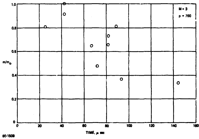
Figure 17 DROP MASS HISTORY; M=3 , p=760
