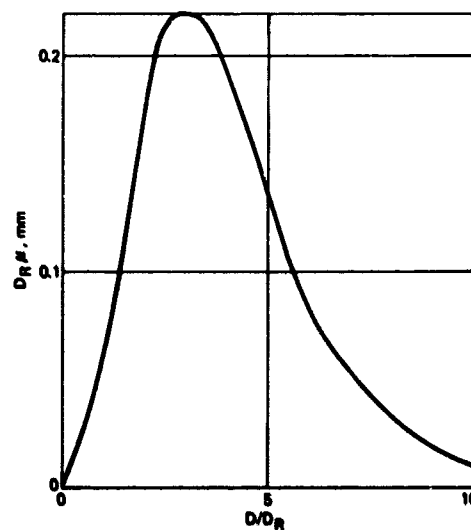
80-1530 Figure 35 RAINSTORM MASS DISTRIBUTION FUNCTION
