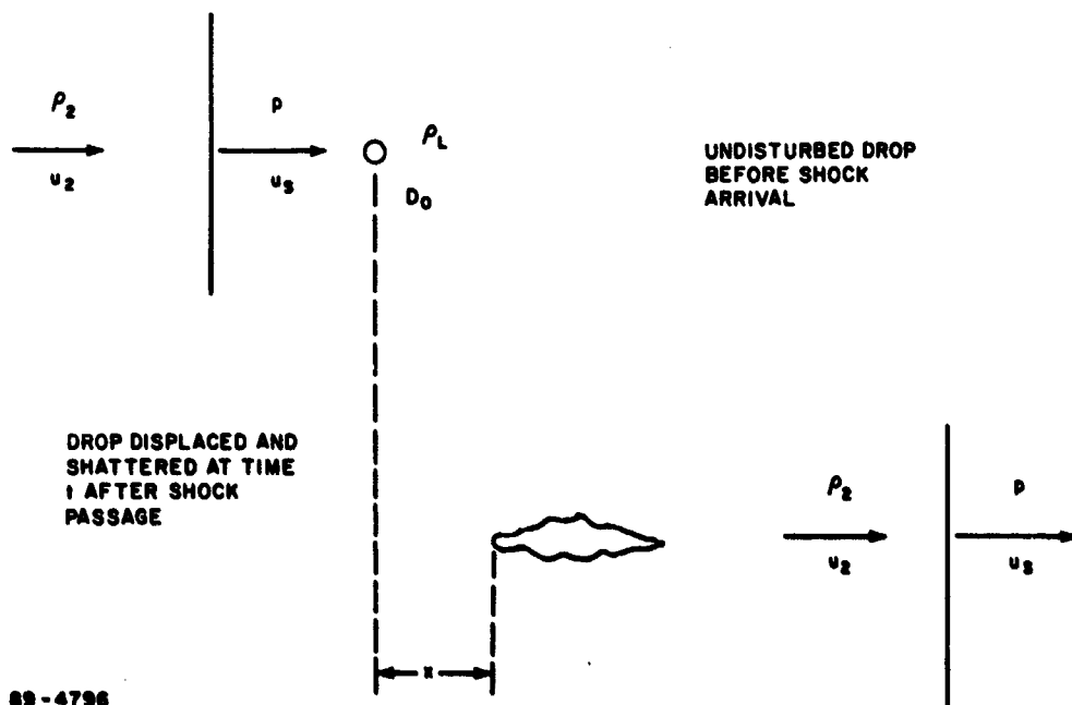
Figure 8 SCHEMATIC OF EXPERIMENT
