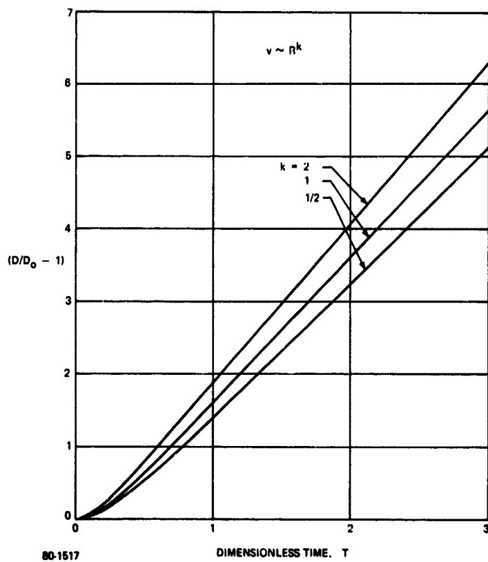
Figure 22 DISK-SHAPED DROP DEFORMATION
