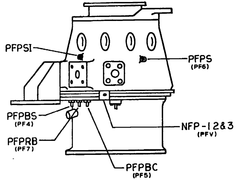
b. Fuel Turbopump Sensor Locations Fig. III-1 Continued
