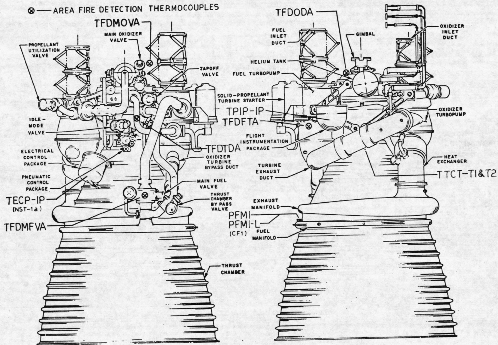
a. General Arrangement Fig. III-1 Selected Sensor Locations
