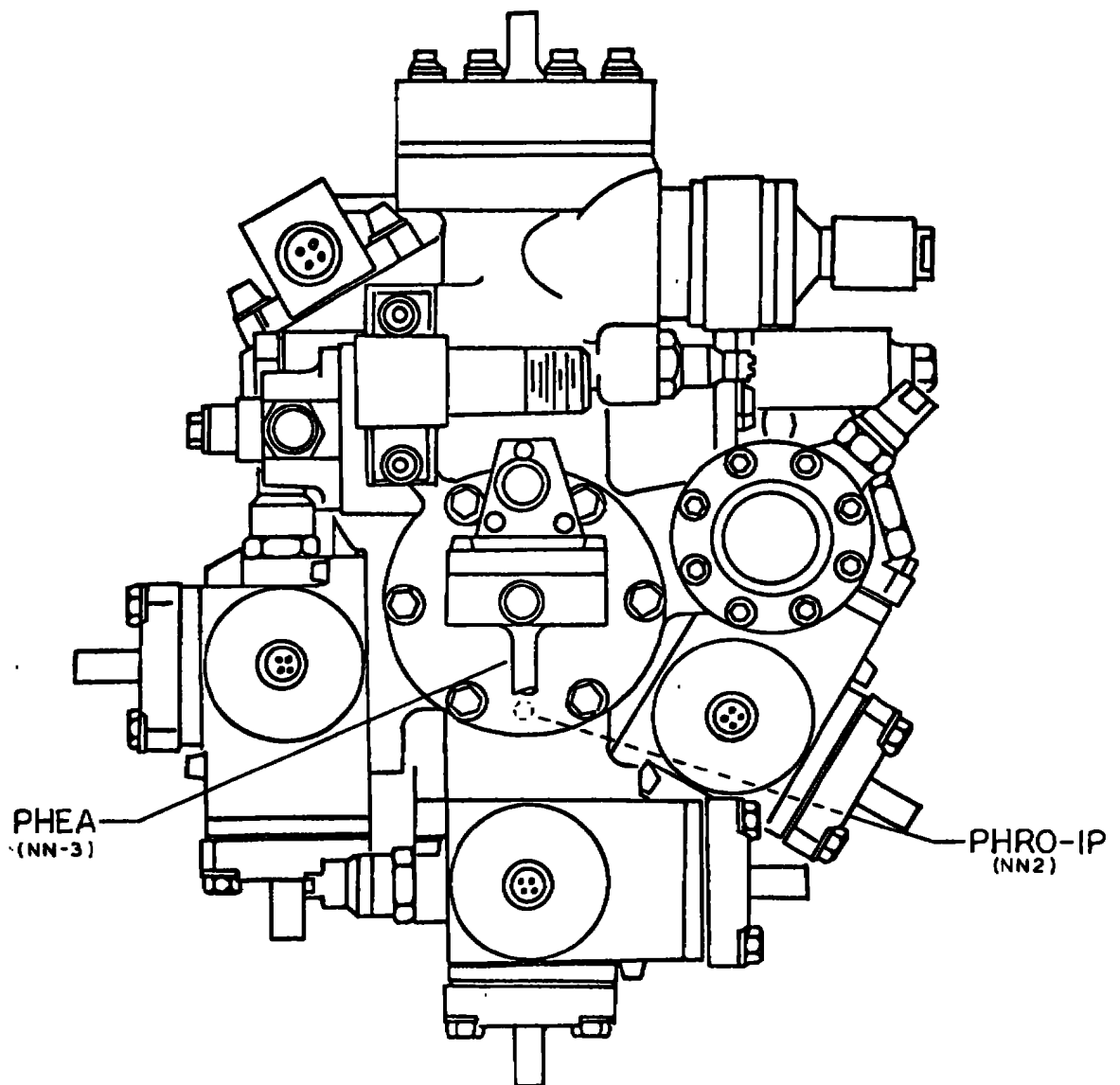
i. Pneumatic Control Package Sensor Locations Fig. III-1 Continued
