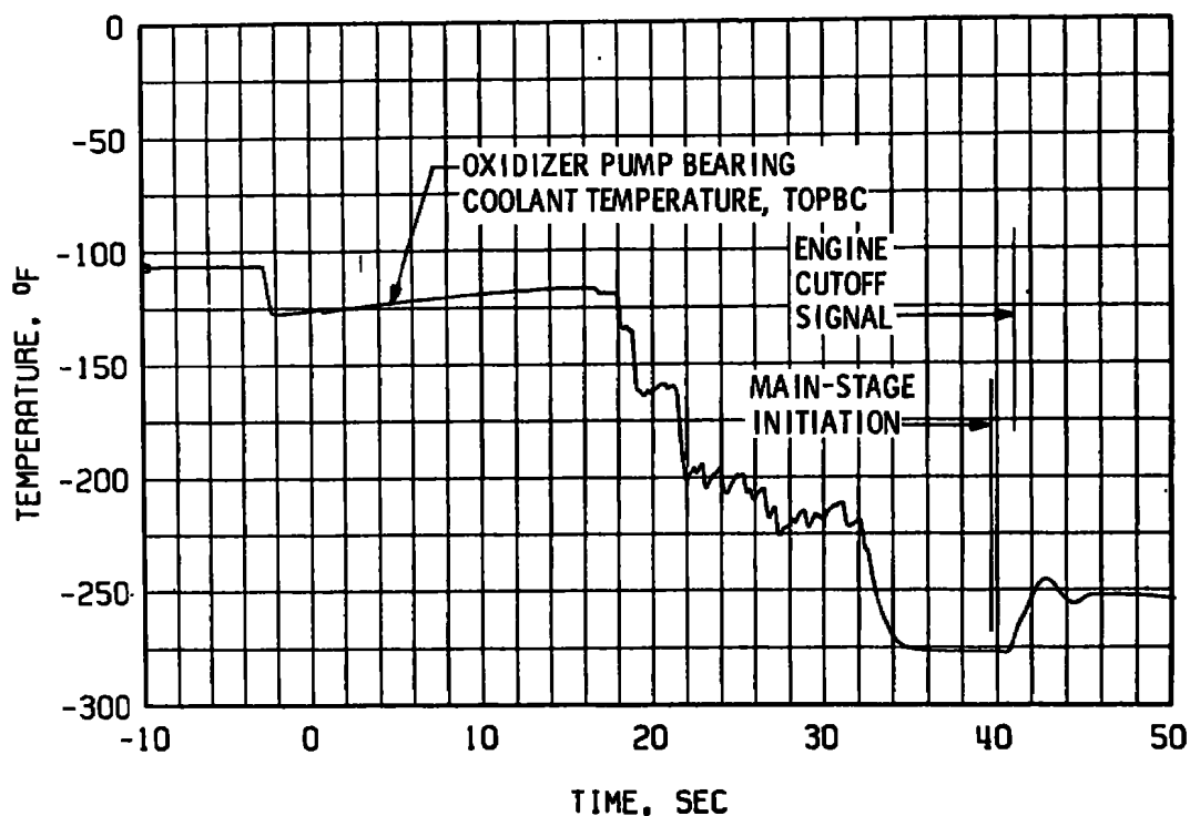
Fig. 35 Oxidizer Pump Bearing Coolant Temperature, Firing 04B
