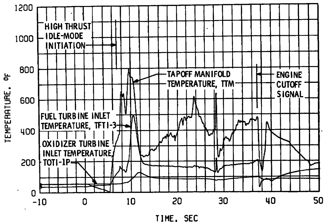
Fig. 34 Turbine System Temperatures, Firing 05C
