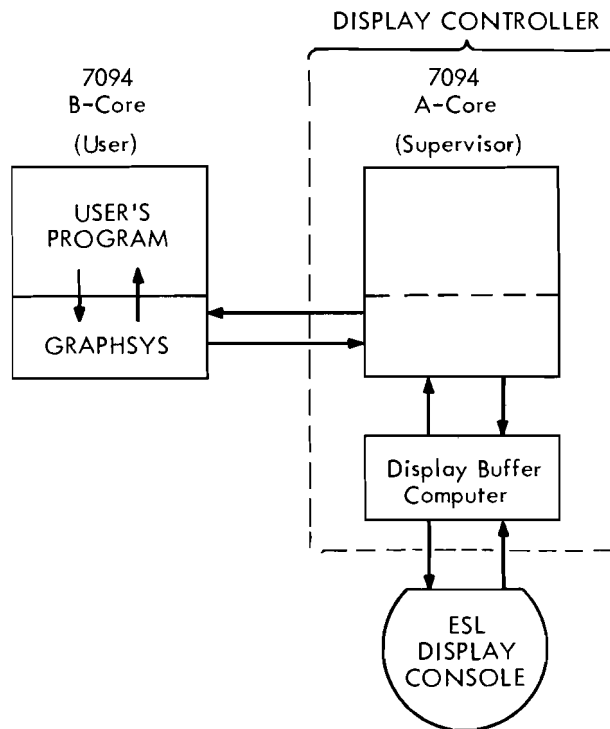
Fig. 17 Information Flow in Display System
