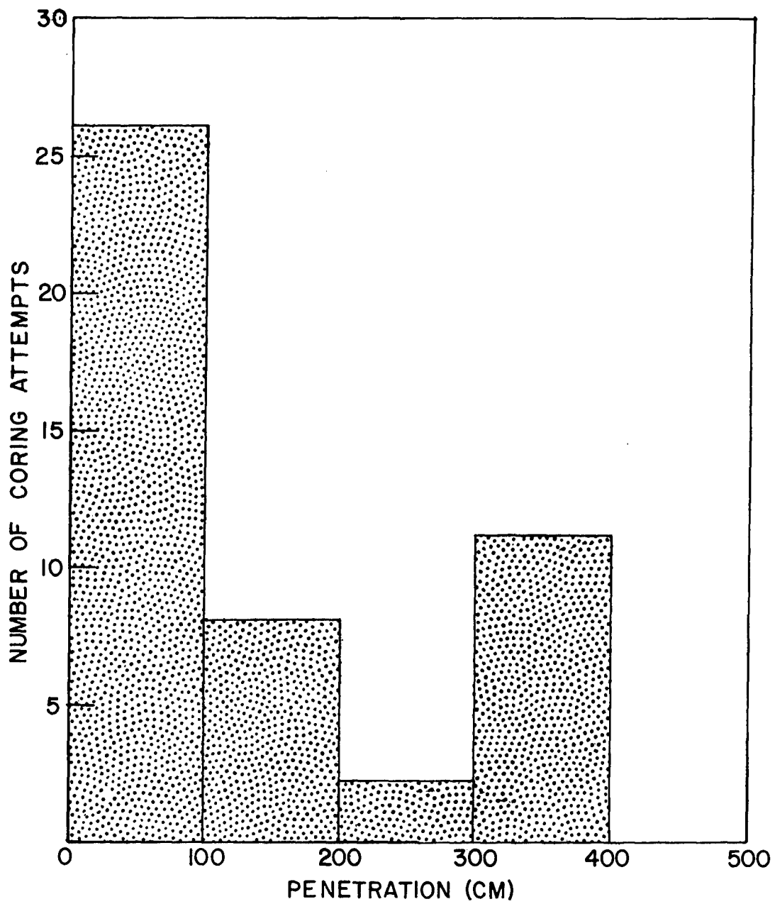
Figure 2. Histogram Depicting Corer Penetration
