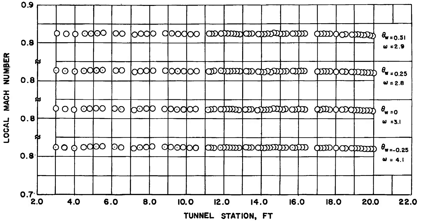
d. M = 0.825, \lambda = 1.140 Fig. 10 Continued
