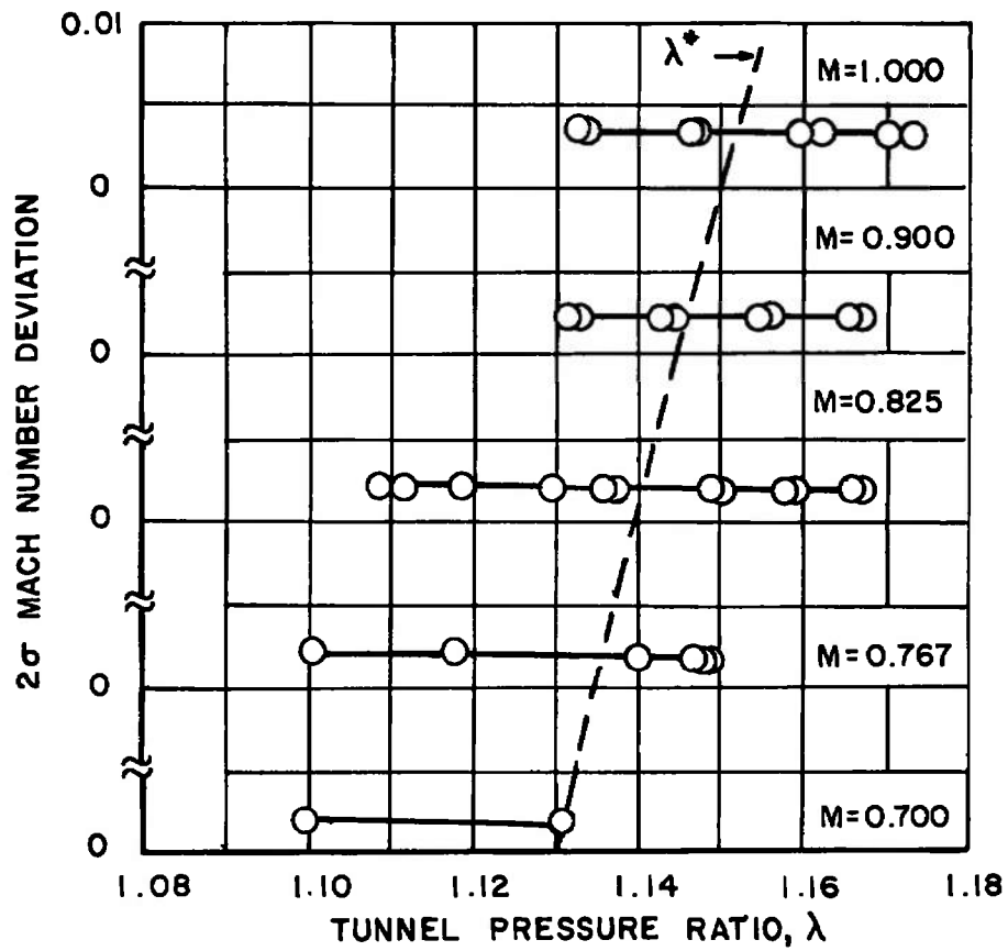
a. Tunnel Station 7.83 to 13.17
