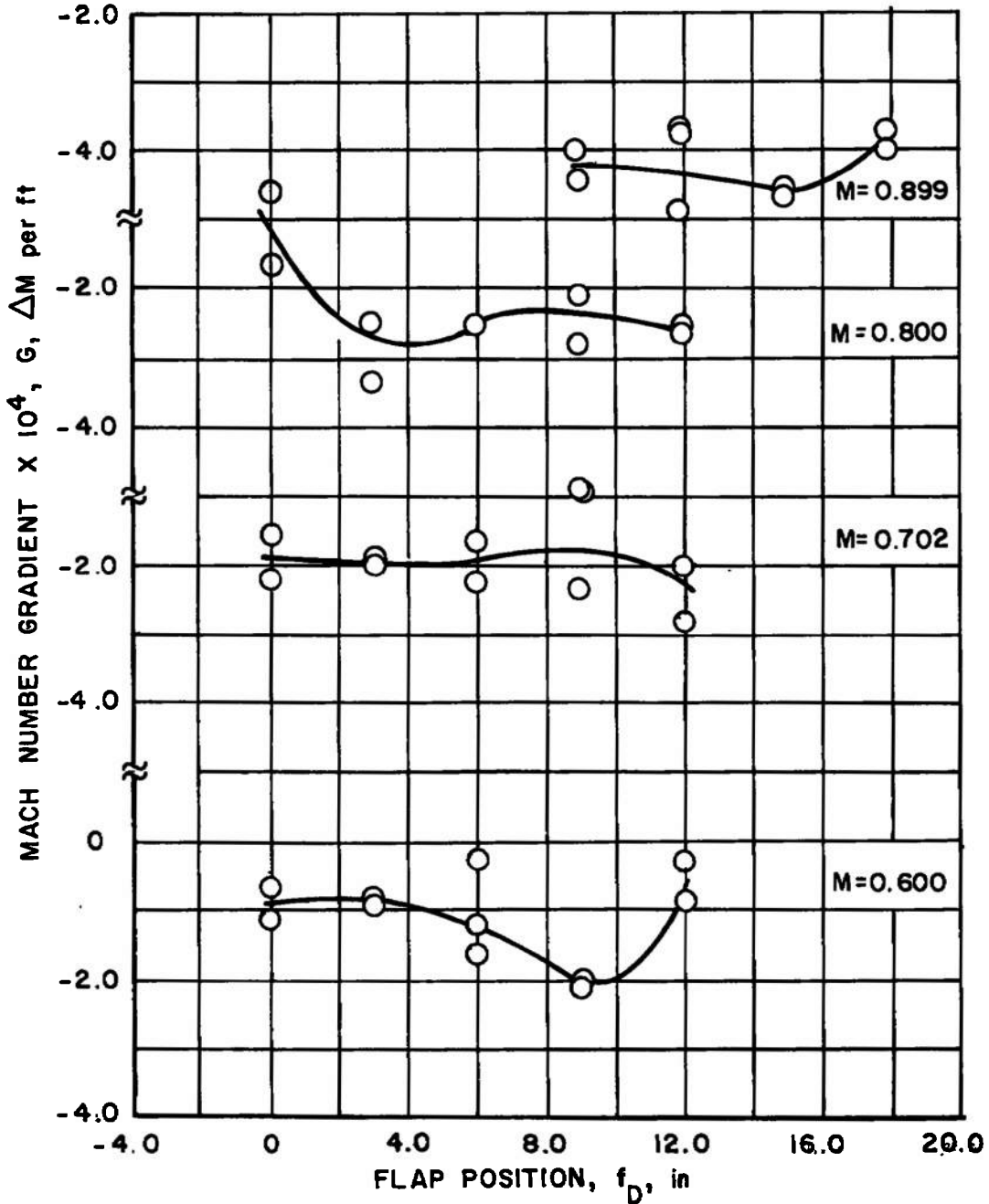
a. Tunnel Station 7.83 to 13.17
