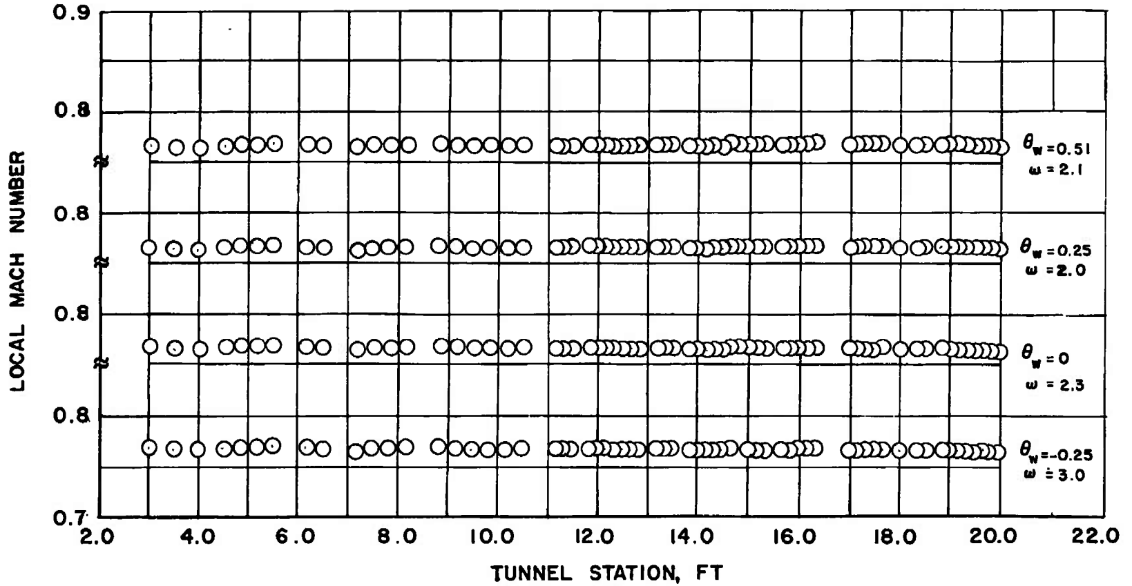
c. M = 0.767, \lambda = 1.135 Fig.10 Continued
