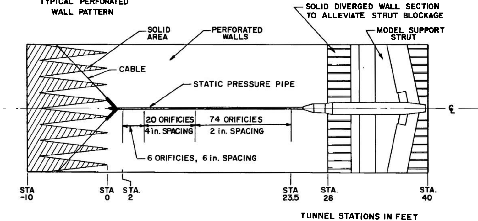
Fig. 1 Schematic of the Test Section and Centerline Pipe Installation
