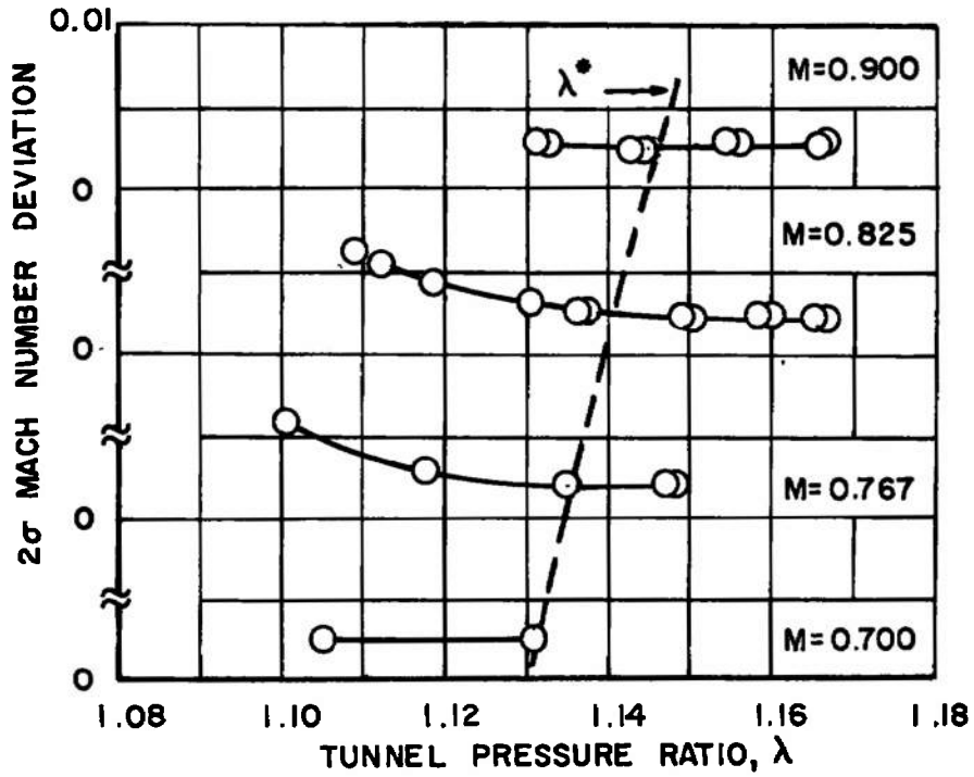
b. Tunnel Station 3.00 to 19.00 Fig. 8 Concluded
