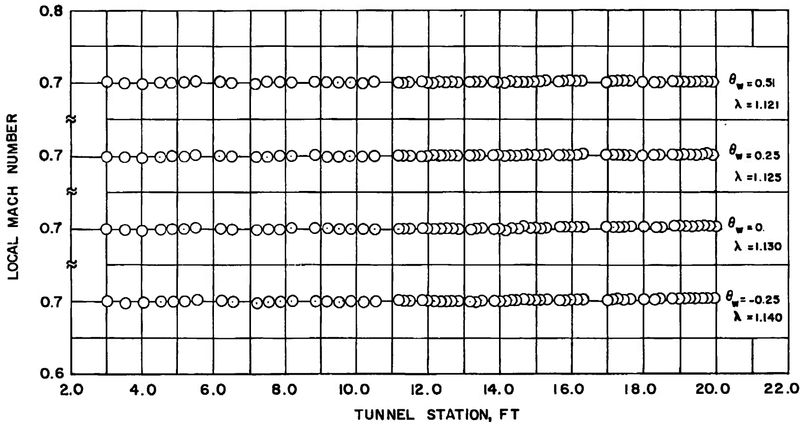
b. M = 0.700 , \omega = 0 Fig. 10 Continued
