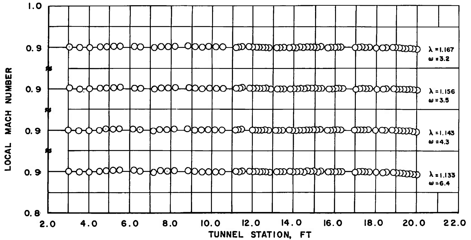
d. M = 0.900 Fig. 7 Continued
