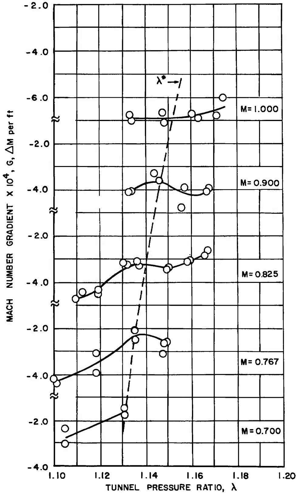
a. Tunnel Station 7.83 to 13.17
