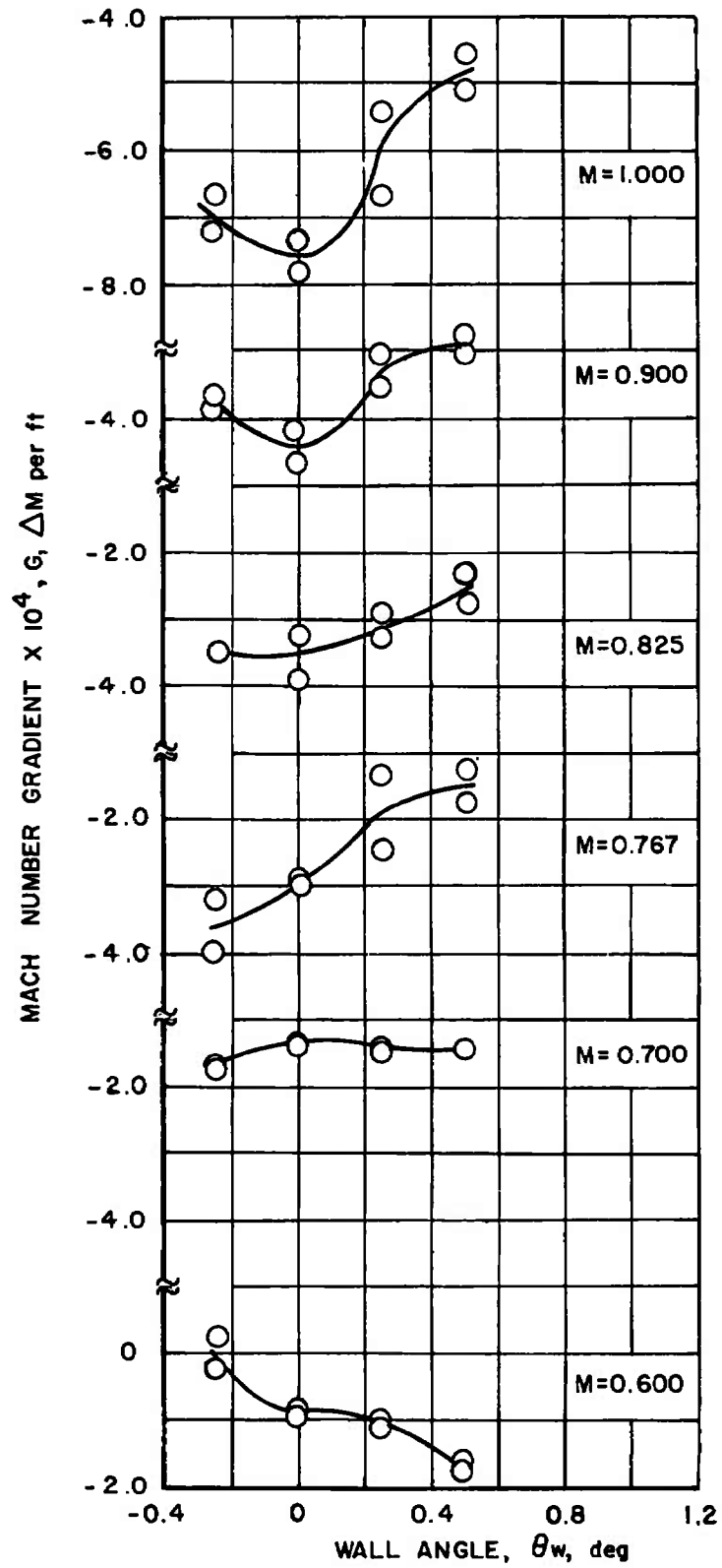
a. Tunnel Station 7.83 to 13.17
