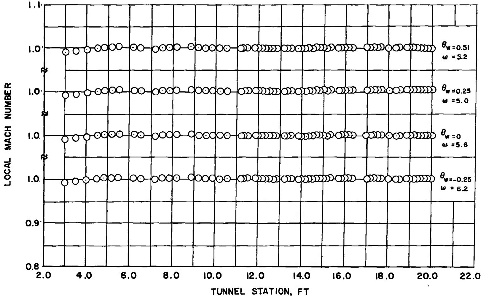
f. M = 1.000 , \lambda = 1.152 Fig. 10 Concluded
