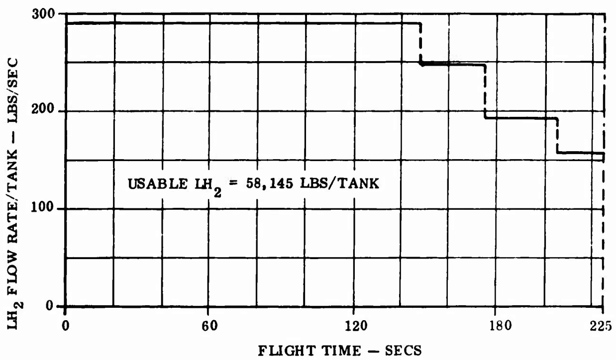
Figure 55. Propellant Outflow Rates
