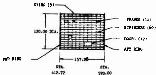
CENTAUR INTERSTAGE ADAPTER
