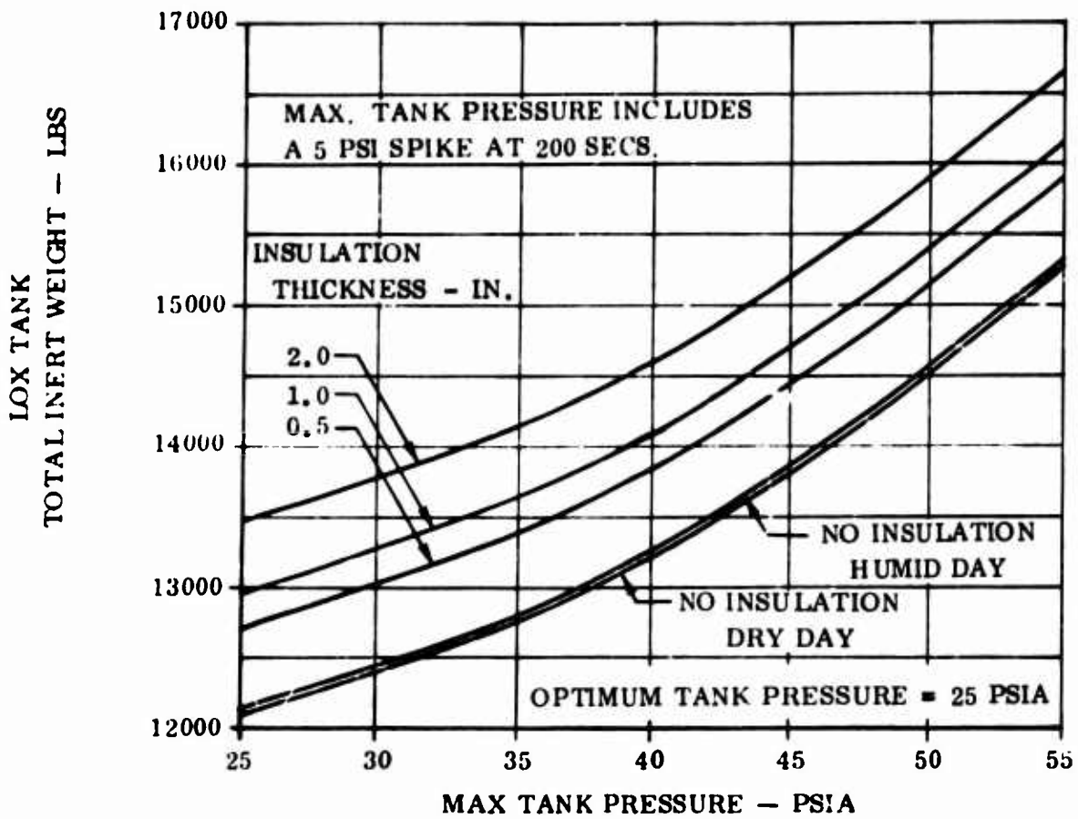
Figure 63. Total LOX Tank Inert Weight vs. Max. Tank Pressure - MPO With Pressure Spike
