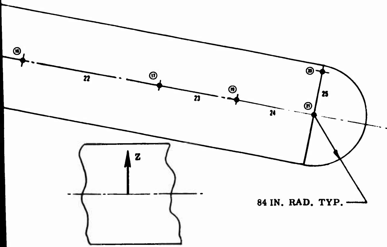
Figure 3. Structural Model for Internal Loads and Geometry - Intertank Adapter and LH 2 Tanks
