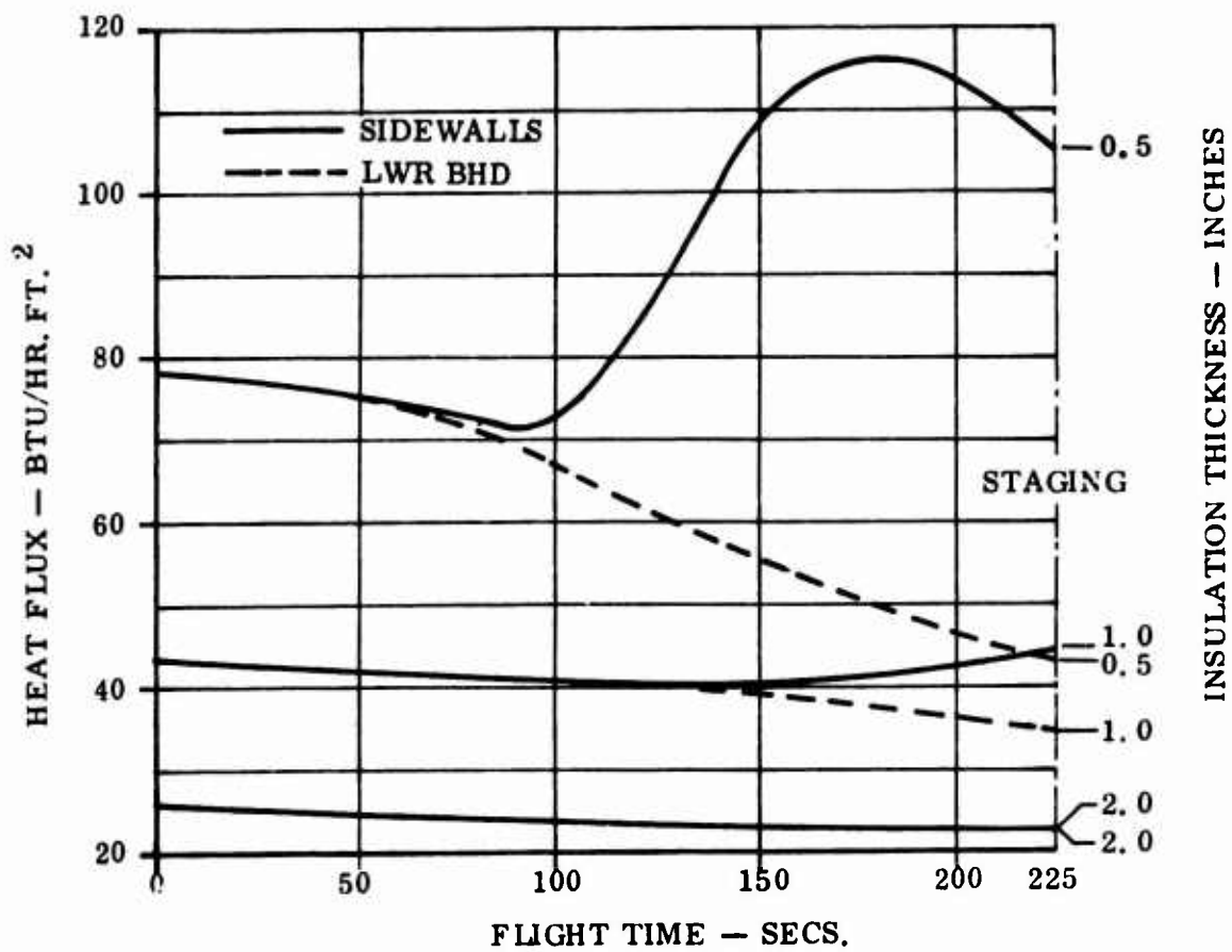
Figure 54. Propellant Heating During Flight - LOX Tank
