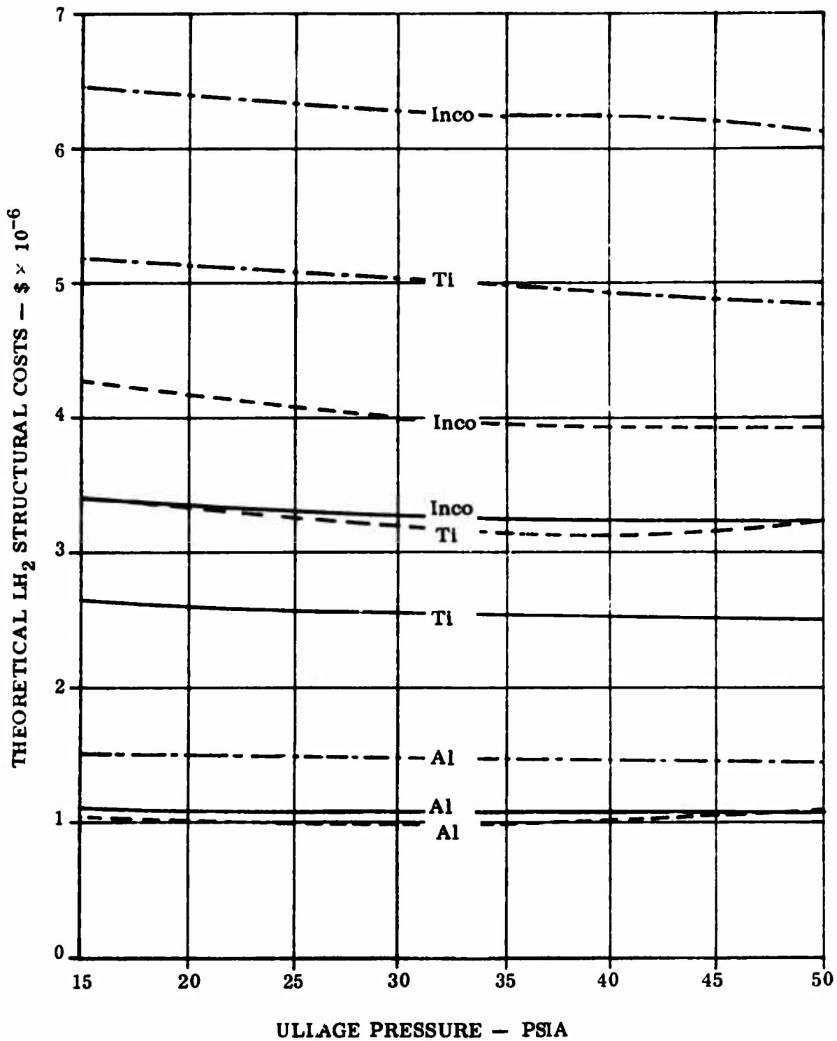
Figure 33 Theoretical LH 2 Tank Structure Costs versus Ullage Pressure
