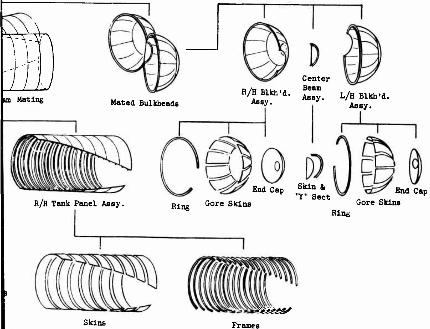
Figure 91. LOX Tank Manufacturing Breakdown and Assembly Sequence
