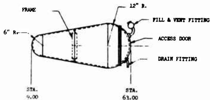
HYPERSONIC MODEL LH 2 TANK
