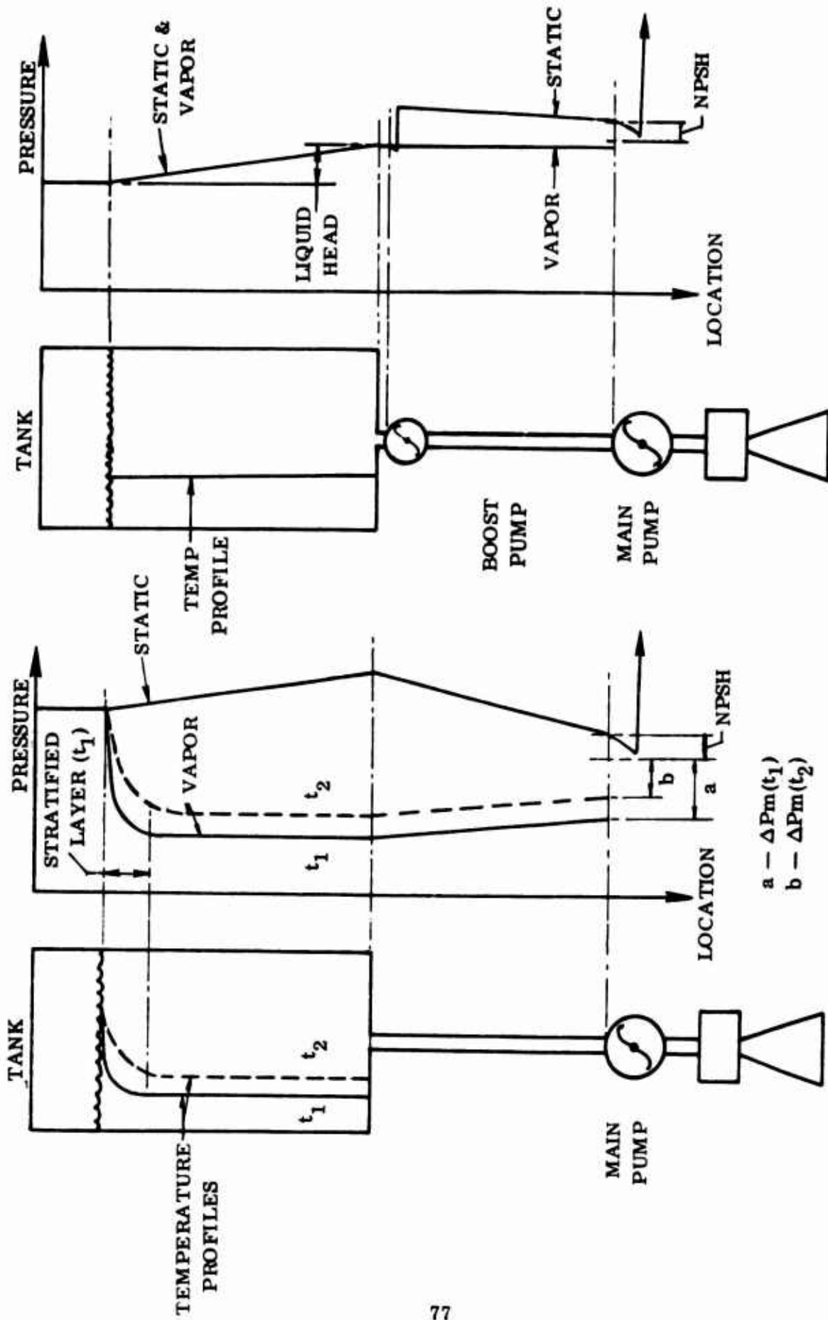
Figure 43. Boost Pump System
