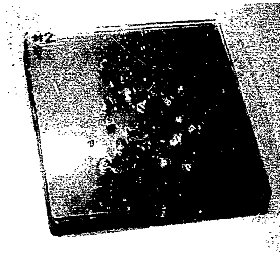
(b) Ballistically Tested Unbonded Multiple Ply Polycarbonate Plates Demonstrating Multiple Hit Capability.
