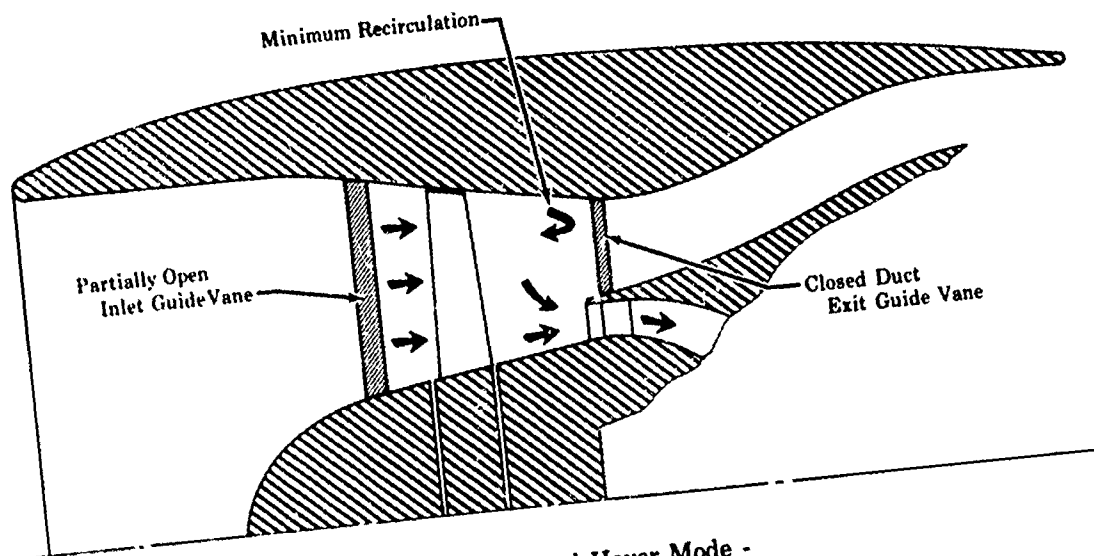
Figure 1. Variable Geometry Fan for Efficient Fan-to-Shaft Power Transfer.
