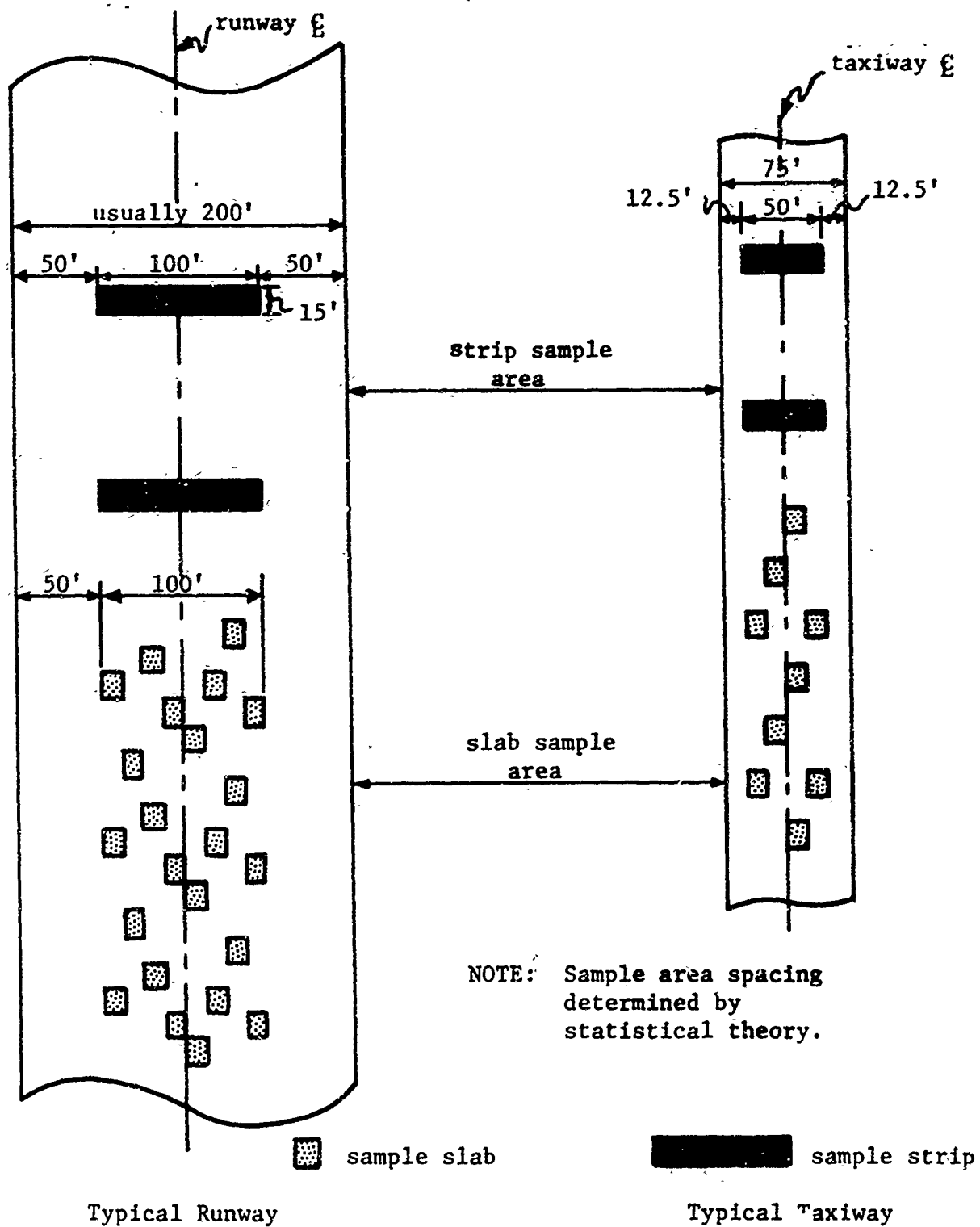
Figure 3. Portland cement concrete sample areas.
