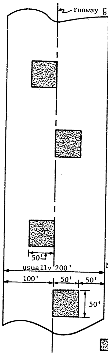
Typical Runway
