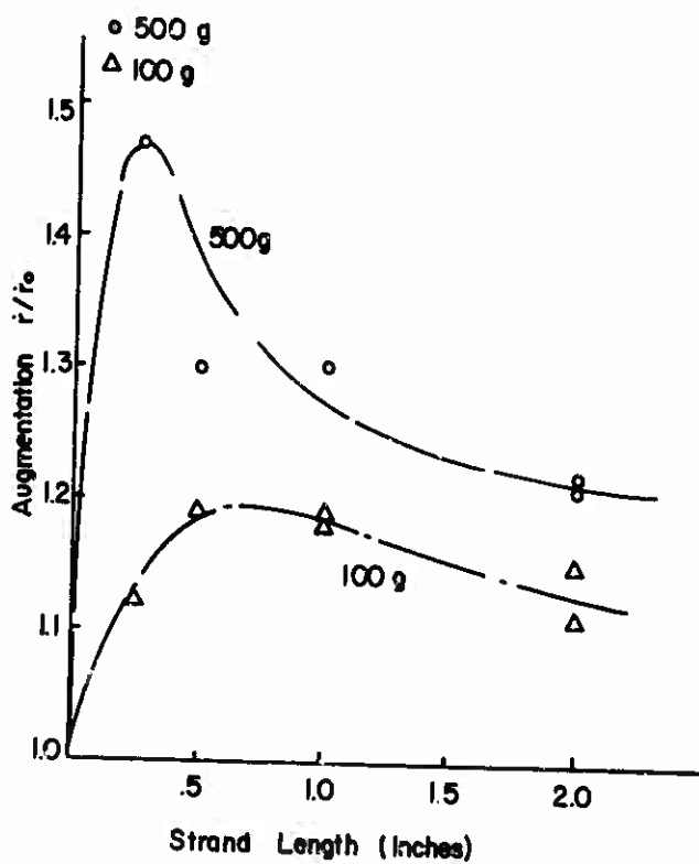
FIGURE 10. EFFECT OF STRAND LENGTH ON AUGMENTATION
