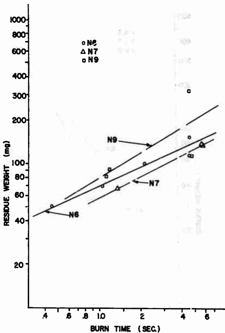
FIGURE 20. EFFECT OF BURN TIME ON RESIDUE WEIGHT OF N6, N7, N9, AT 500 g.
