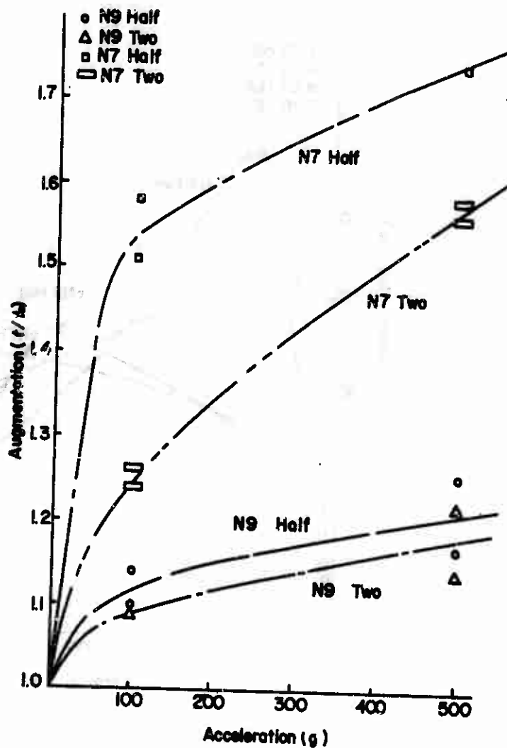
FIGURE 17. EFFECT OF BASE BURNING RATE ON AUGMENTATION
