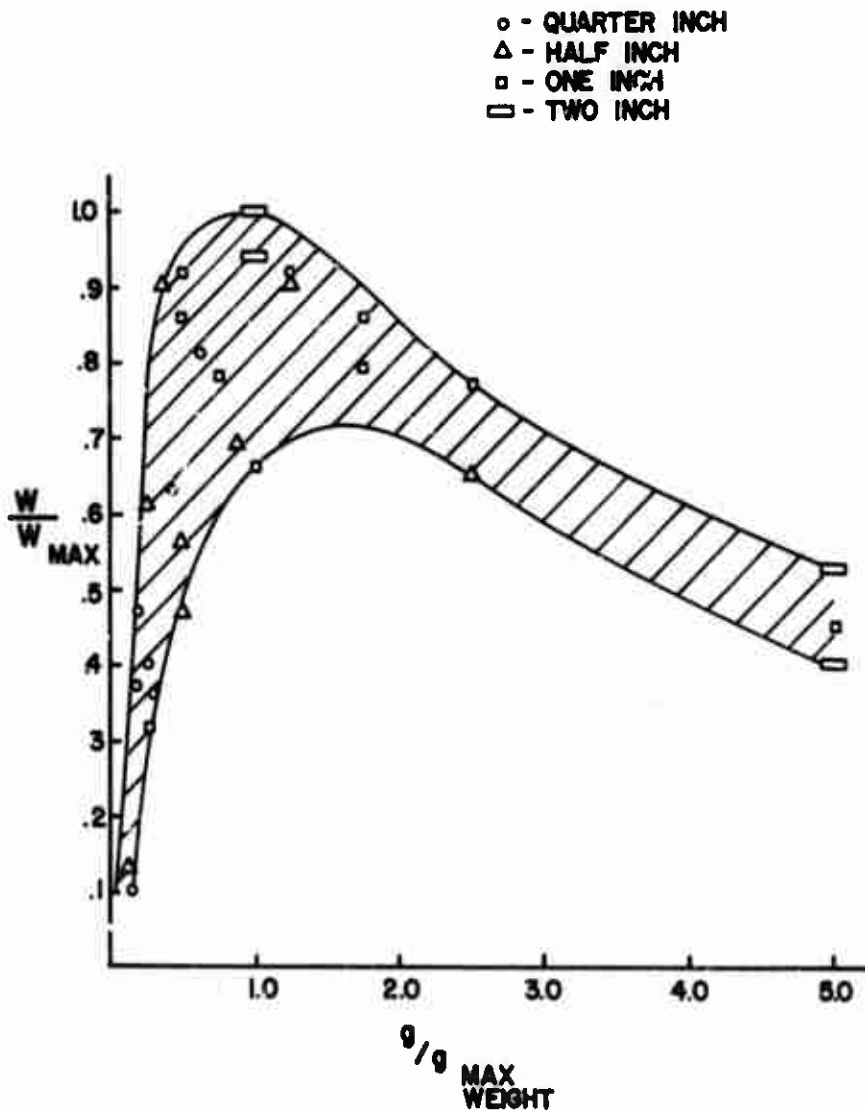
FIGURE 9. EFFECT OF ACCELERATION ON RESIDUE WEIGHT FOR PROPELLANT N6 (NORMALIZED FORM)
