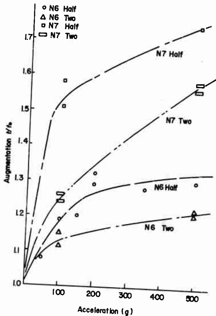
FIGURE 12. EFFECT OF BASE BURNING RATE AND AP SIZE ON AUGMENTATION
