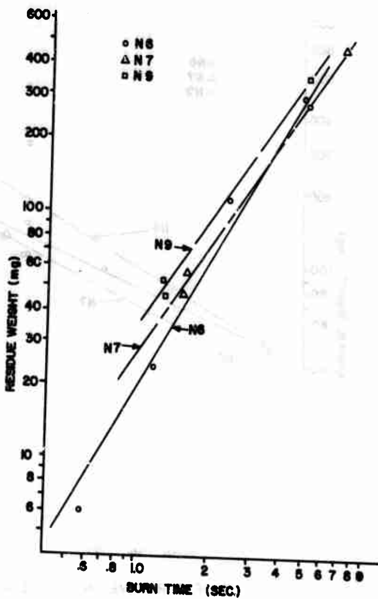
FIGURE 19. EFFECT OF BURN TIME ON RESIDUE WEIGHT OF N6, N7, N9, AT 100g.
