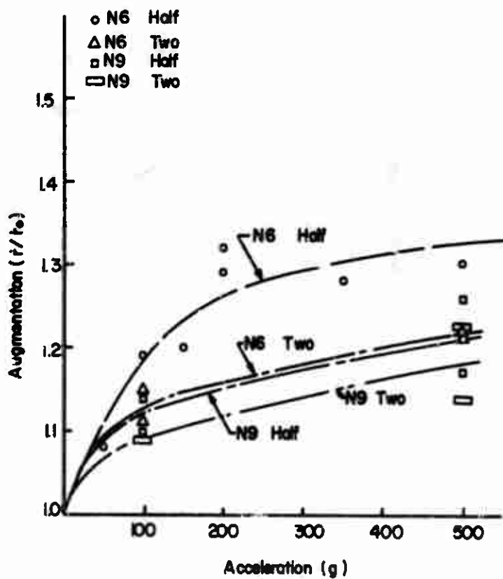
FIGURE 15. EFFECT OF AP SIZE ON AUGMENTATION
