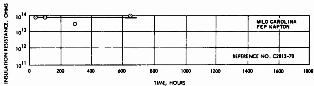
Figure 40. Insulation resistance as a function of thermal aging in air at 550°F – Wire type VI
