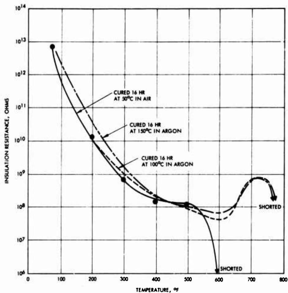
Figure 3. Insulation resistance measurements on perfluoroalkylenetriazine coated wires - 2.6 percent terephthalonitrile N, N' -dioxide
