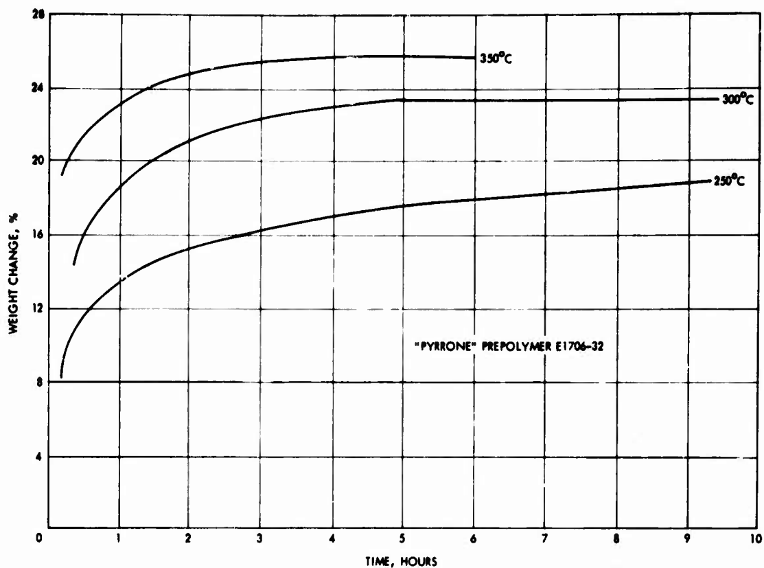
Figure 4. "Pyrrone" prepolymer weight loss as a function of cure temperature
