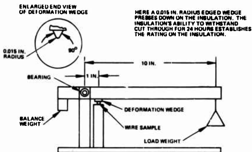
Figure 59. Insulation cut through tester
