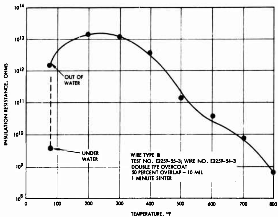
Figure 10. Insulation resistance of water-soaked Teflon TFE overcoated "pyrrone"-Kapton insulated wire - double overcoat - 1 minute sinter
