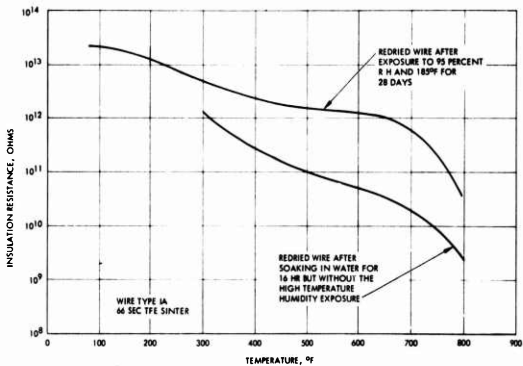
Figure 57. Insulation resistance of Teflon TFE overwrapped "pyrrone"-Kapton insulated wire before and after humidity test
