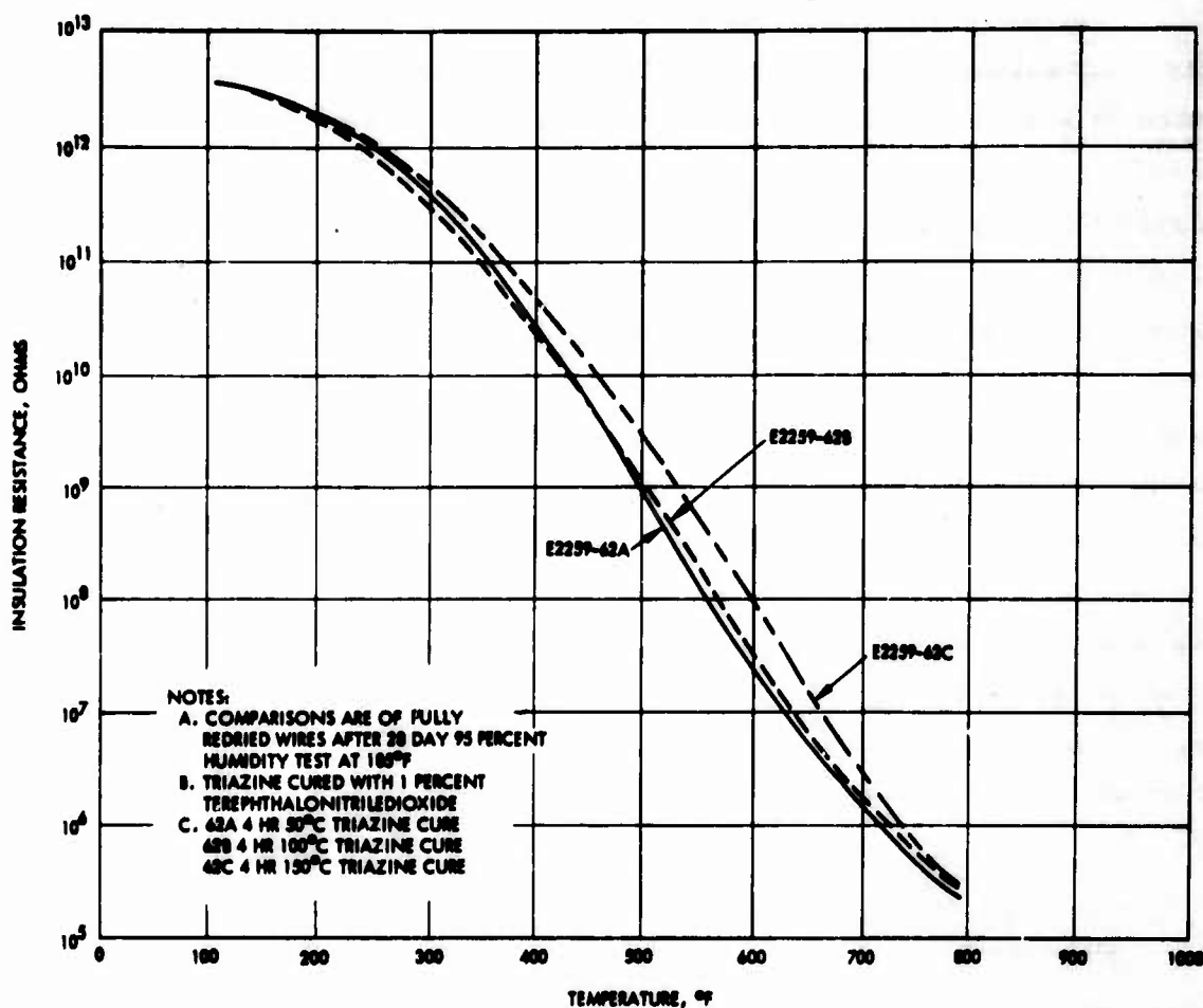
Figure 52. Insulation resistance as a function of temperature - perfluoroalkylenetriazine overcoated "pyrrone"-Kapton
