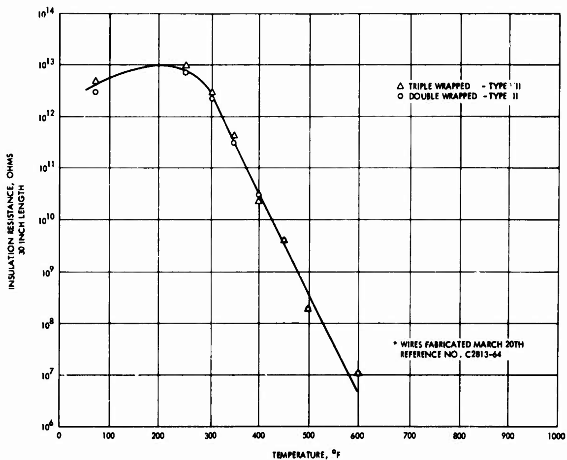
Figure 17. Insulation resistance of double and triple wrapped HR-100-Kapton wires as a function of temperature
