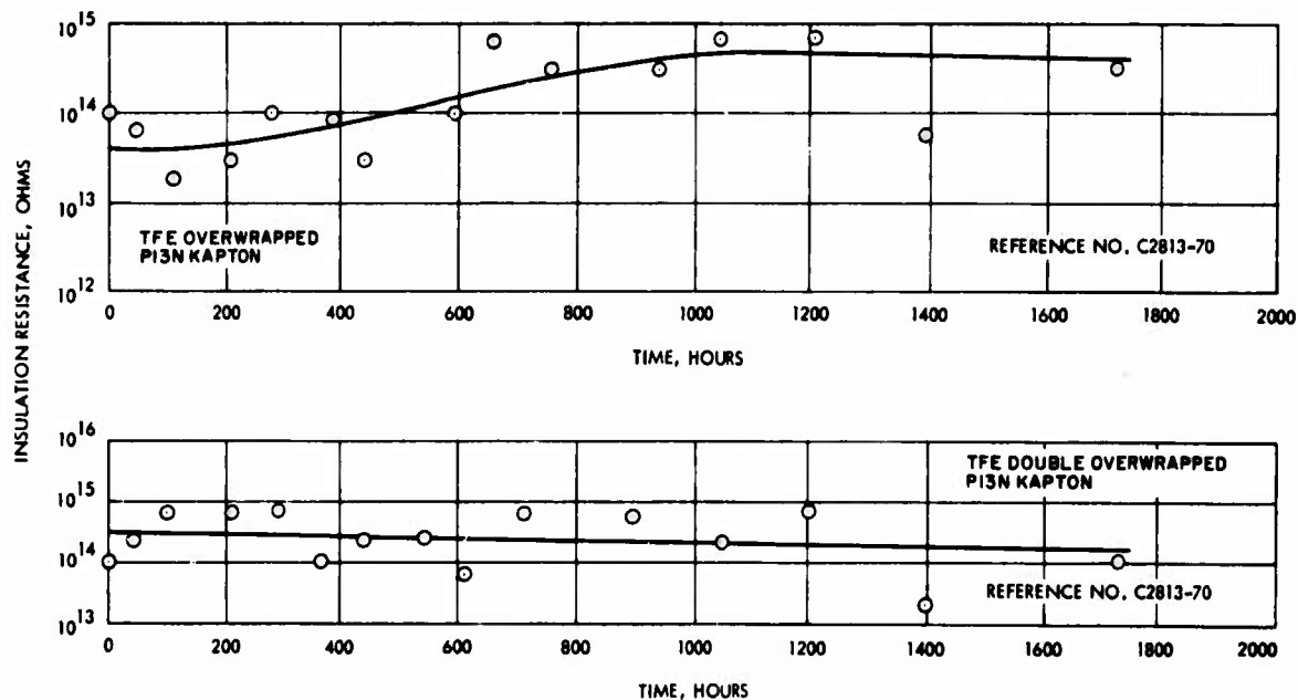
Figure 39. Insulation resistance as a function of thermal aging in air at 550°F - Wire type IVA (top) and IVB (bottom)
