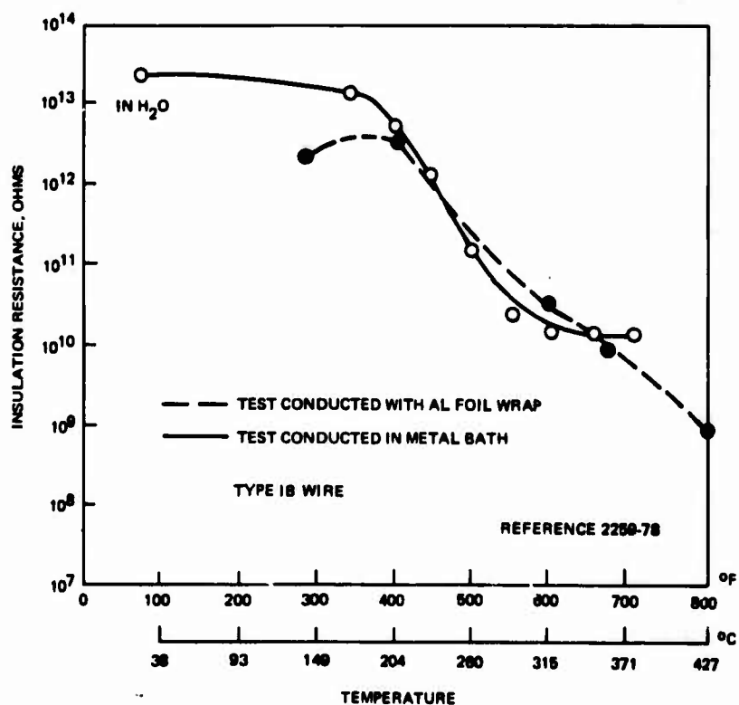
Figure 26. Insulation resistance of "pyrrone" - Kapton insulated wire with double Teflon over-coat (Wire Type IB)
