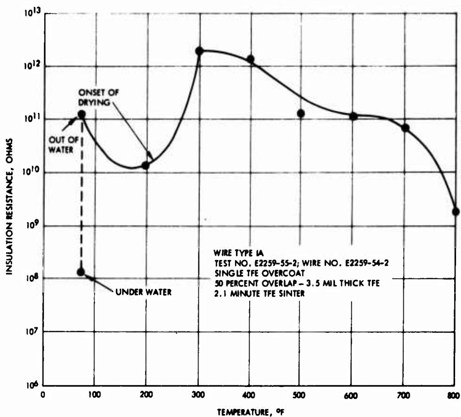
Figure 9. Insulation resistance of water-soaked Teflon TFE overcoated "pyrrone"-Kapton insulated wire - single overcoat - 2 minute sinter
