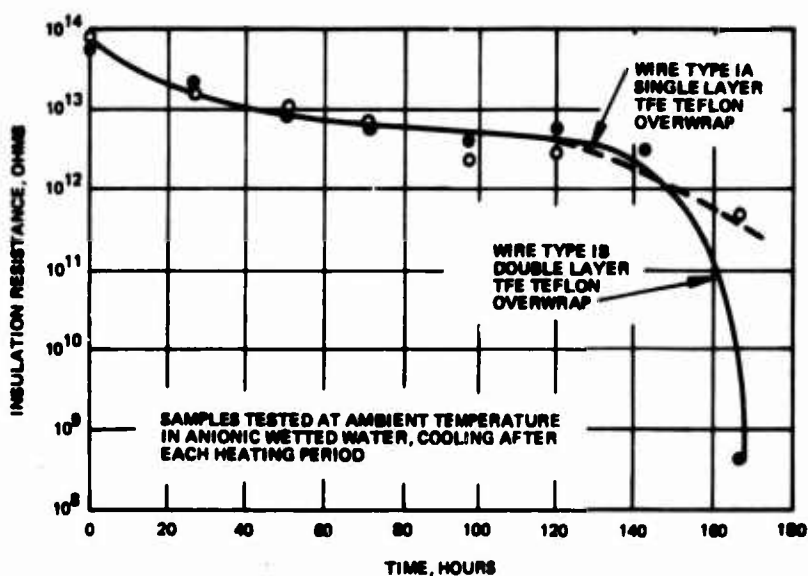
Figure 14. Insulation resistance of "pyrrone"-Kapton insulated wires as a function of thermal aging in air at 600°F
