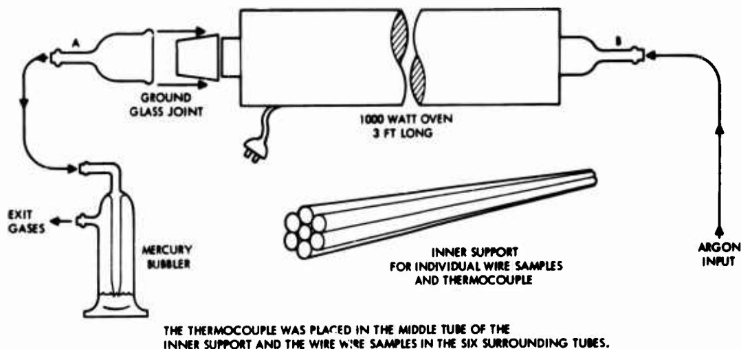
Figure 7. Wire postcure oven
