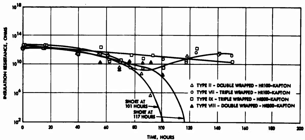
Figure 46. Insulation resistance as a function of thermal aging in air at 700°F – Wire types II, VII, VIII, and IX
