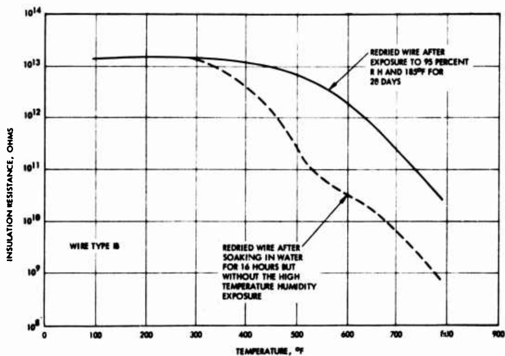
Figure 58. Insulation resistance of double overwrapped Teflon TFE on "pyrrone"-Kapton insulated wire before and after humidity test
