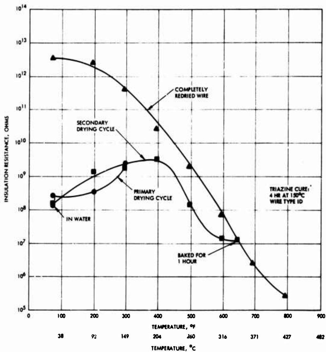
Figure 50. Insulation resistance as a function of temperature—perfluoroalkylenetriazine overcoated "pyrrone"-Kapton
