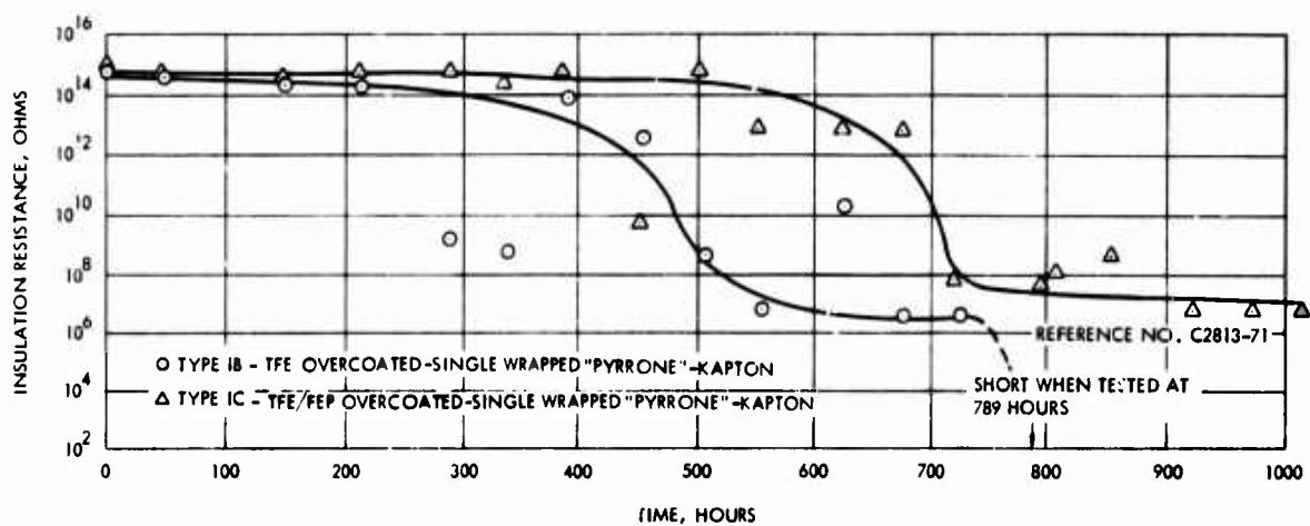
Figure 43. Insulation resistance as a function of thermal aging in air at 600°F – Wires type IB and IC
