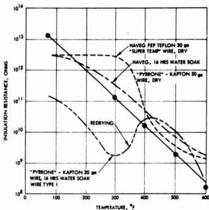
Figure 6. Effect of temperature on insulation resistance
