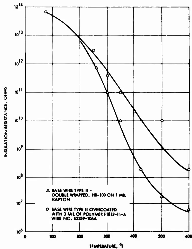
Figure 23. Insulation resistance versus temperature, Type II wire with 1,3-bis-(p-aminophenoxy) benzene based polyimide overcoat
