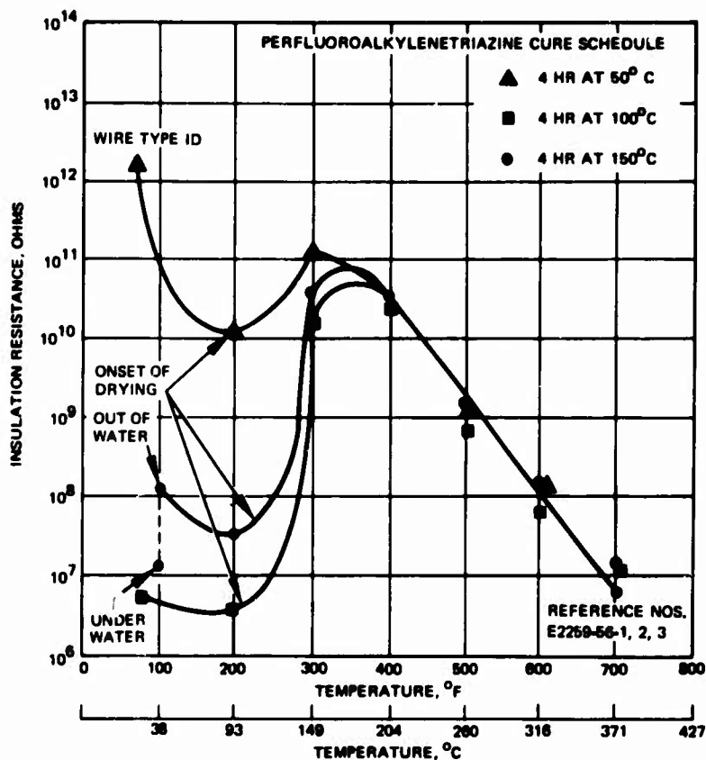
Figure 12. Insulation resistance of perfluoroalkylenetriazine coated "pyrrone"-Kapton insulated wire
