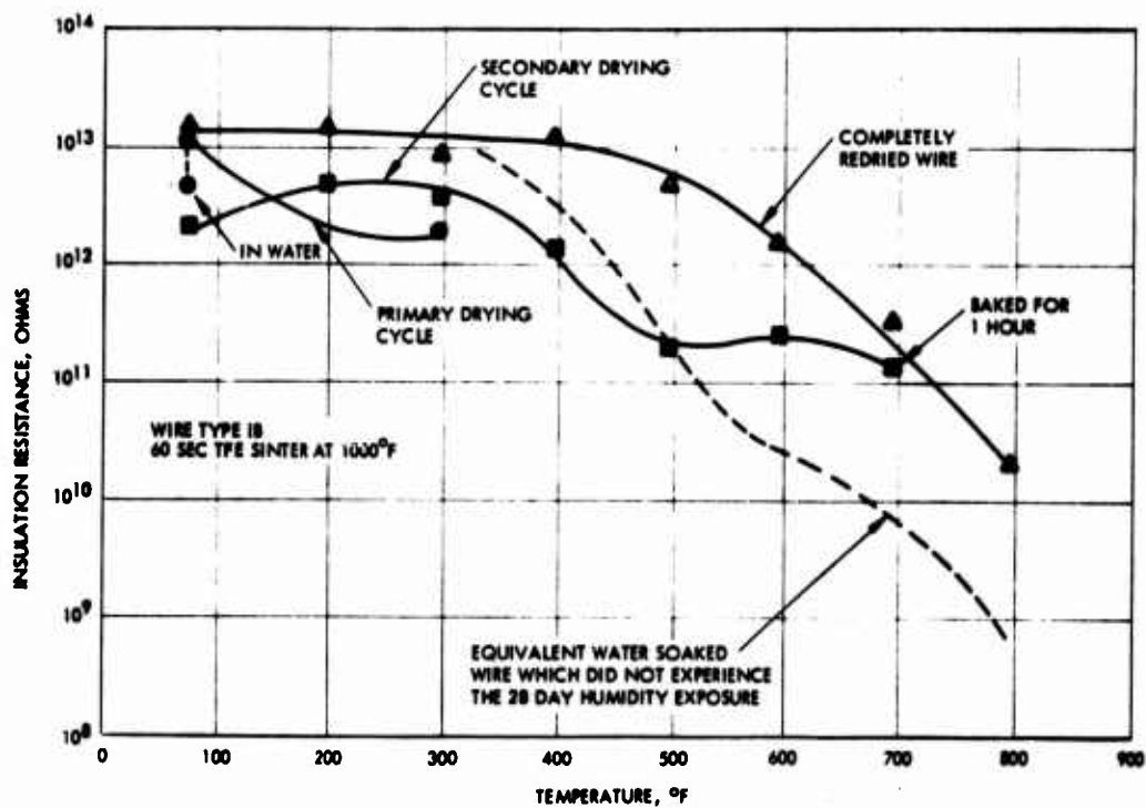
Figure 55. Insulation resistance of Teflon TFE overwrapped "pyrrone"-Kapton insulated wire after 28 days at 95 percent relative humidity (double wrap, 60 sec sinter)
