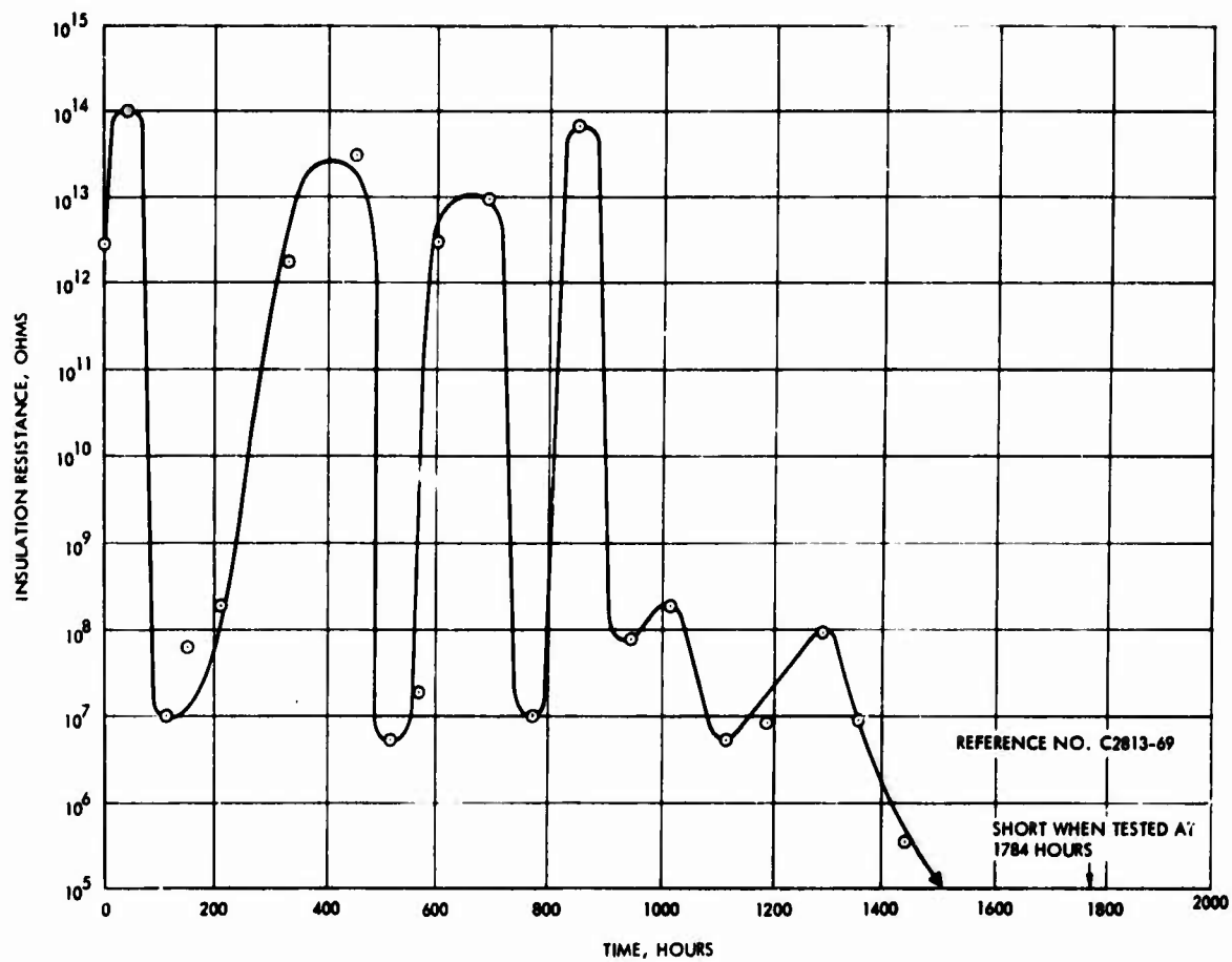
Figure 34. Insulation resistance as a function of thermal aging in air at 550°F — Wire type IA
