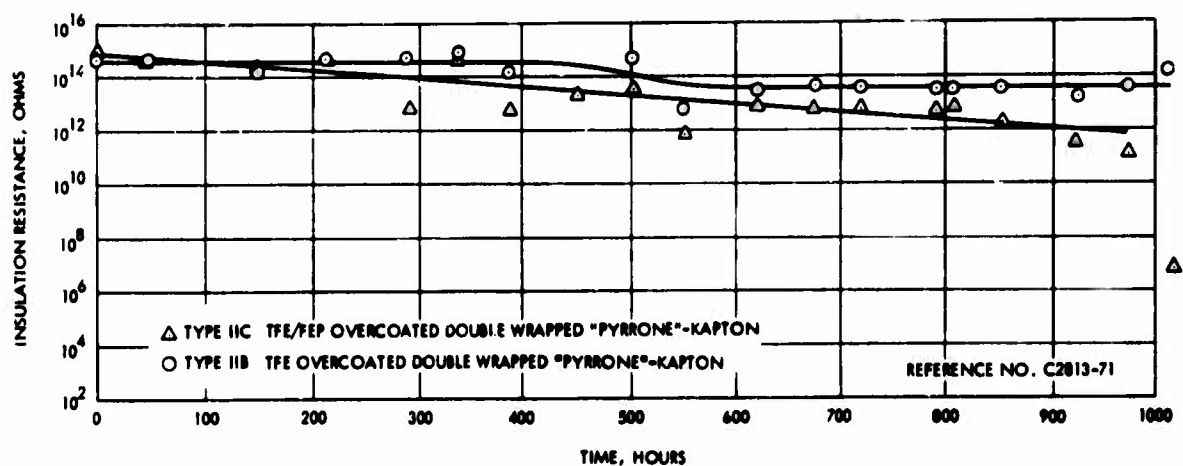
Figure 42. Insulation resistance as a function of thermal aging in air at 600°F – Wires type IIB and IIC
