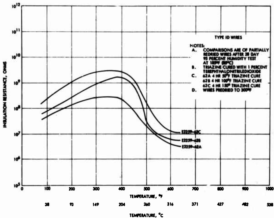
Figure 51. Insulation resistance as a function of temperature—perfluoroalkylenetriazine overcoated "pyrrone"-Kapton
