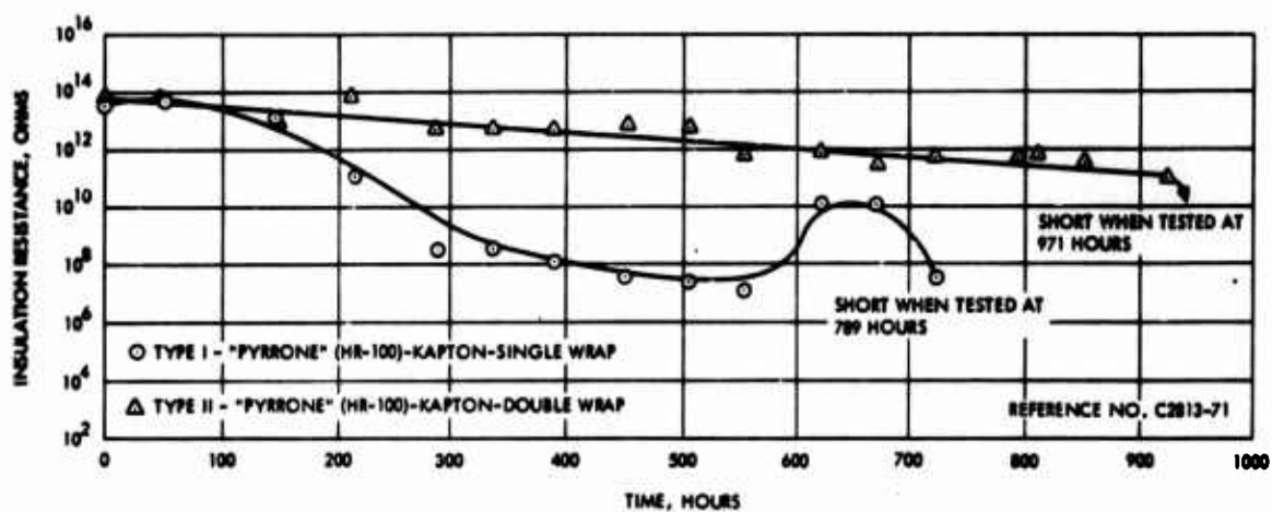
Figure 41. Insulation resistance as a function of thermal aging in air at 600°F – Wires type I and II
