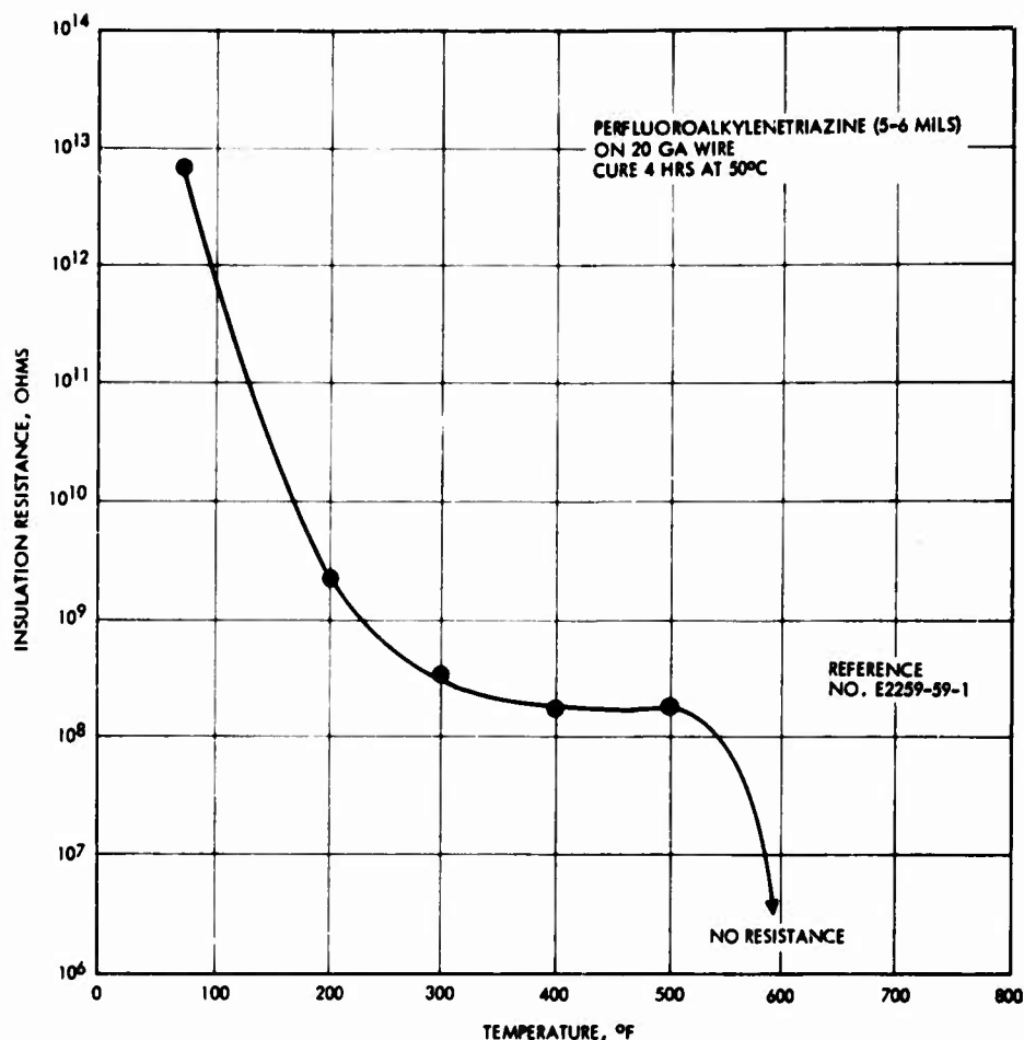
Figure 1. Insulation resistance of perfluoroalkylenetriazine insulated wire
