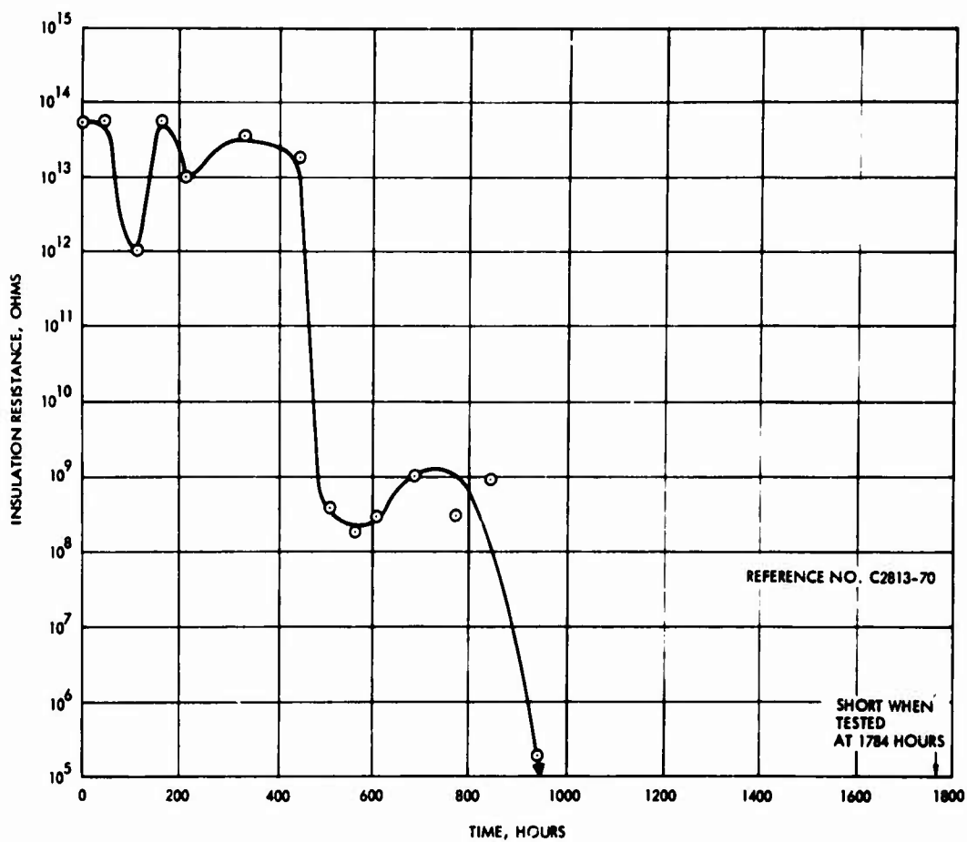
Figure 37. Insulation resistance as a function of thermal aging in air at 550°F – Wire type IV
