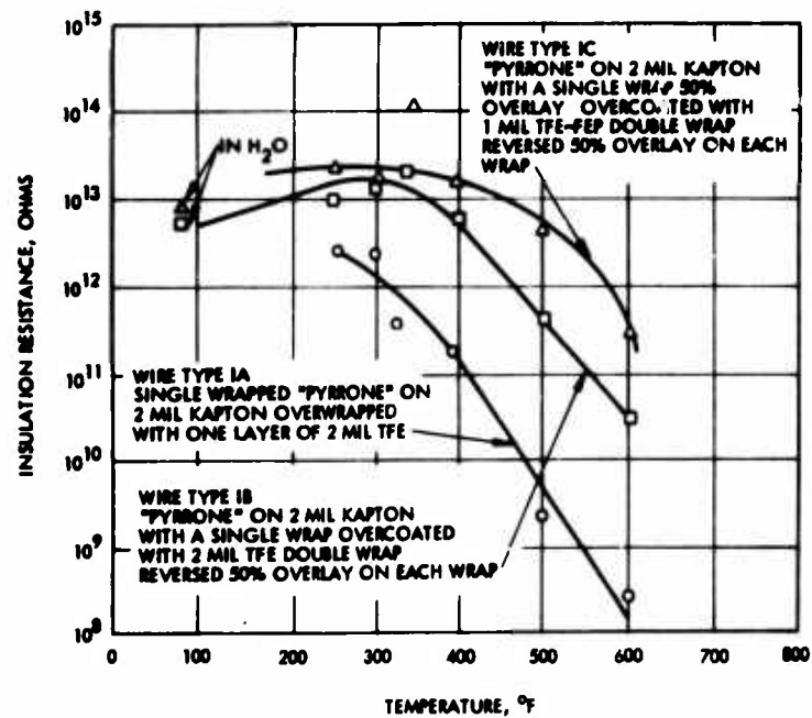
Figure 15. Insulation resistance of Teflon overcoated "pyrrone"-Kapton insulated wires as a function of temperature
