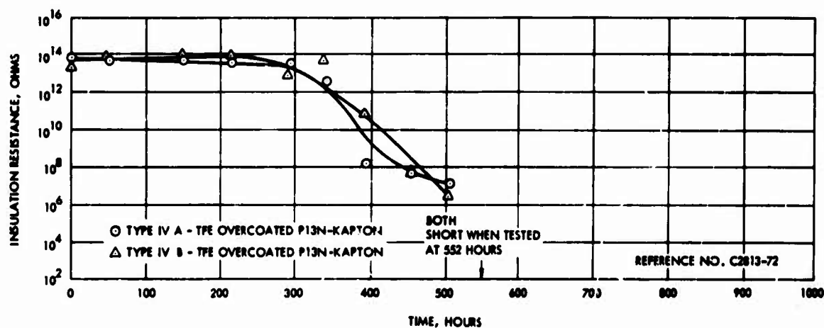
Figure 45. Insulation resistance as a function of thermal aging in air at 600°F – Wires type IVA and IVB
