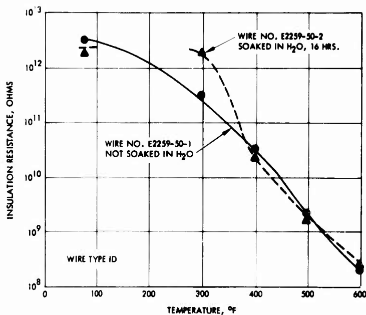
Figure 11. Insulation resistance of perfluoroalkylenetriazine overcoated "pyrrone"-Kapton insulated wire
