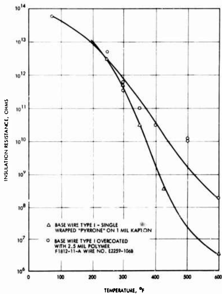
Figure 22. Insulation resistance versus temperature, Type I wire with 1,3-bis-(p-aminophenoxy) benzene based polyimide overcoat
