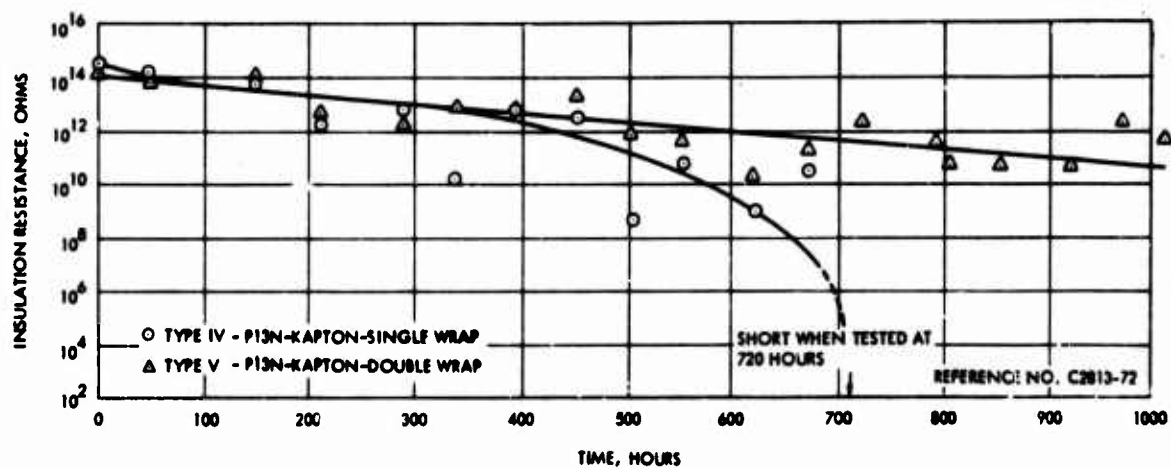
Figure 44. Insulation resistance as a function of thermal aging in air at 600°F – Wire types IV and V
