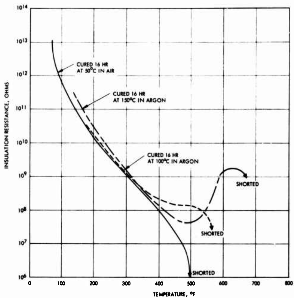
Figure 2. Insulation resistance measurements on perfluoroalkylenetriazine coated wires — 1.3 percent terephthalonitrile N, N'-dioxide
