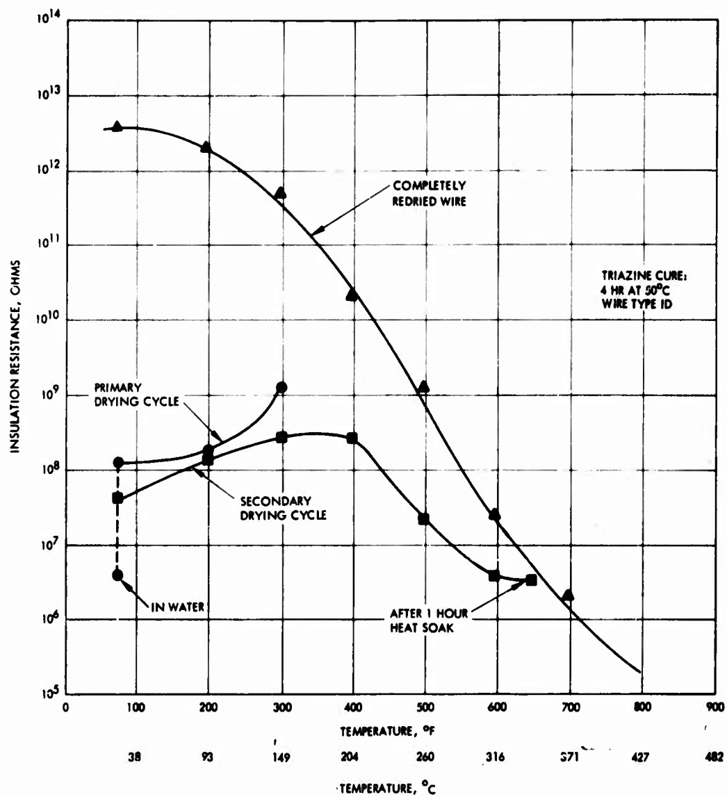
Figure 48. Insulation resistance as a function of temperature—perfluoroalkylenetriazine overcoated "pyrrone"-Kapton
