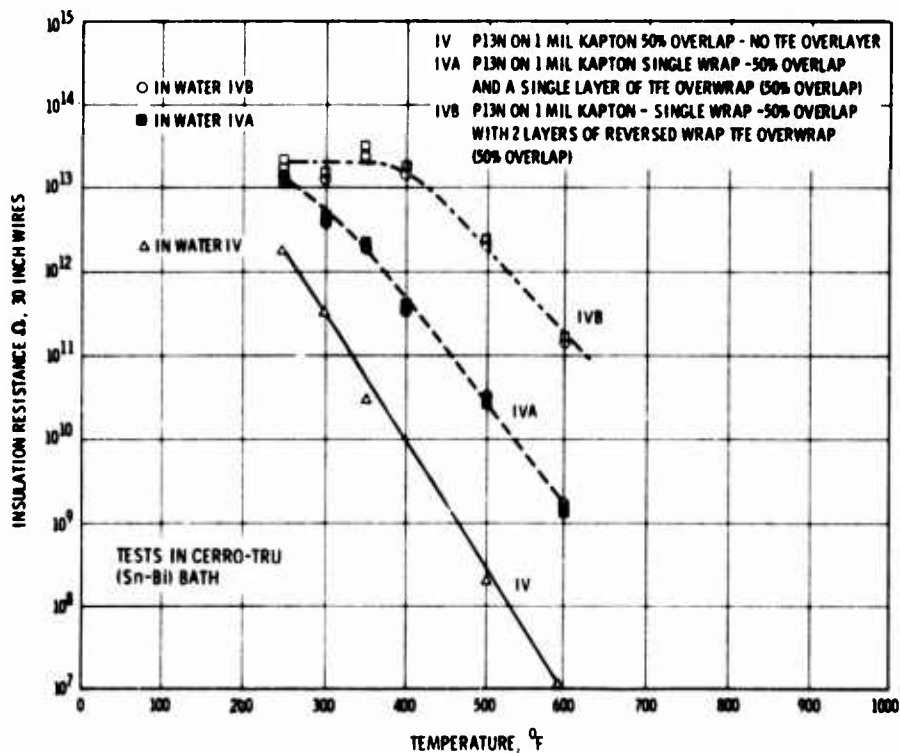
Figure 19. Insulation resistance as a function of temperature of P13N bonded Kapton insulated wires
