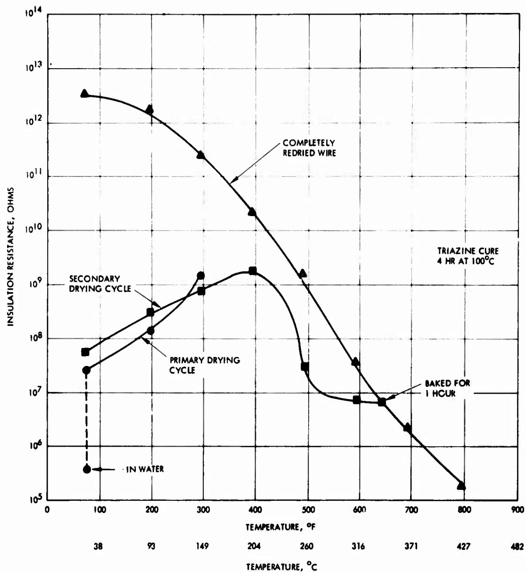
Figure 49. Insulation resistance as a function of temperature—perfluoroalkylenetriazine overcoated "pyrrone"-Kapton
