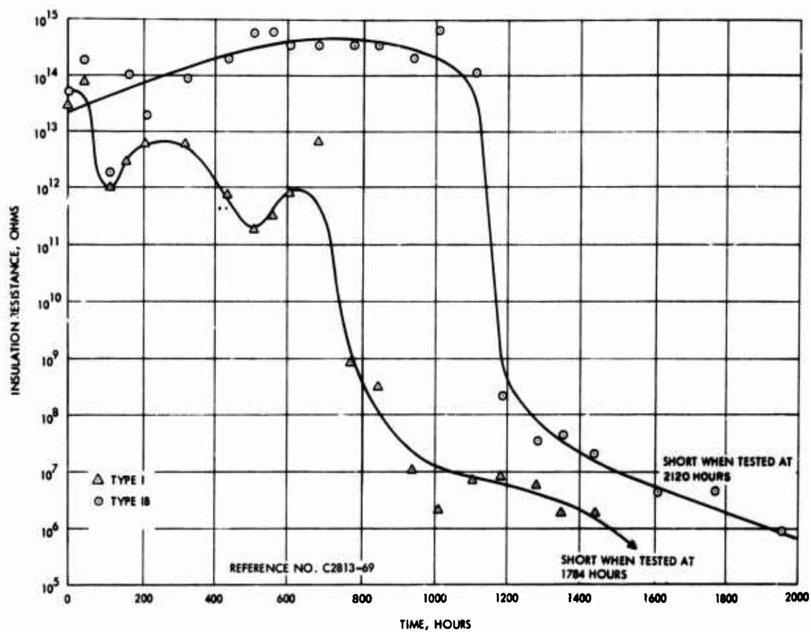
Figure 33. Insulation resistance as a function of thermal aging in air at 550°F — Wires type I and IB
