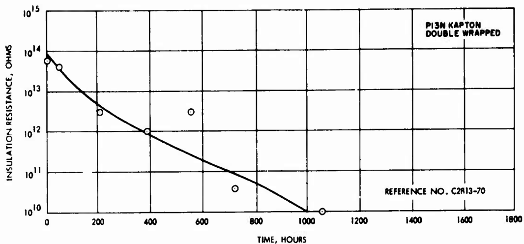
Figure 38. Insulation resistance as a function of thermal aging in air at 550°F - Wire type V
