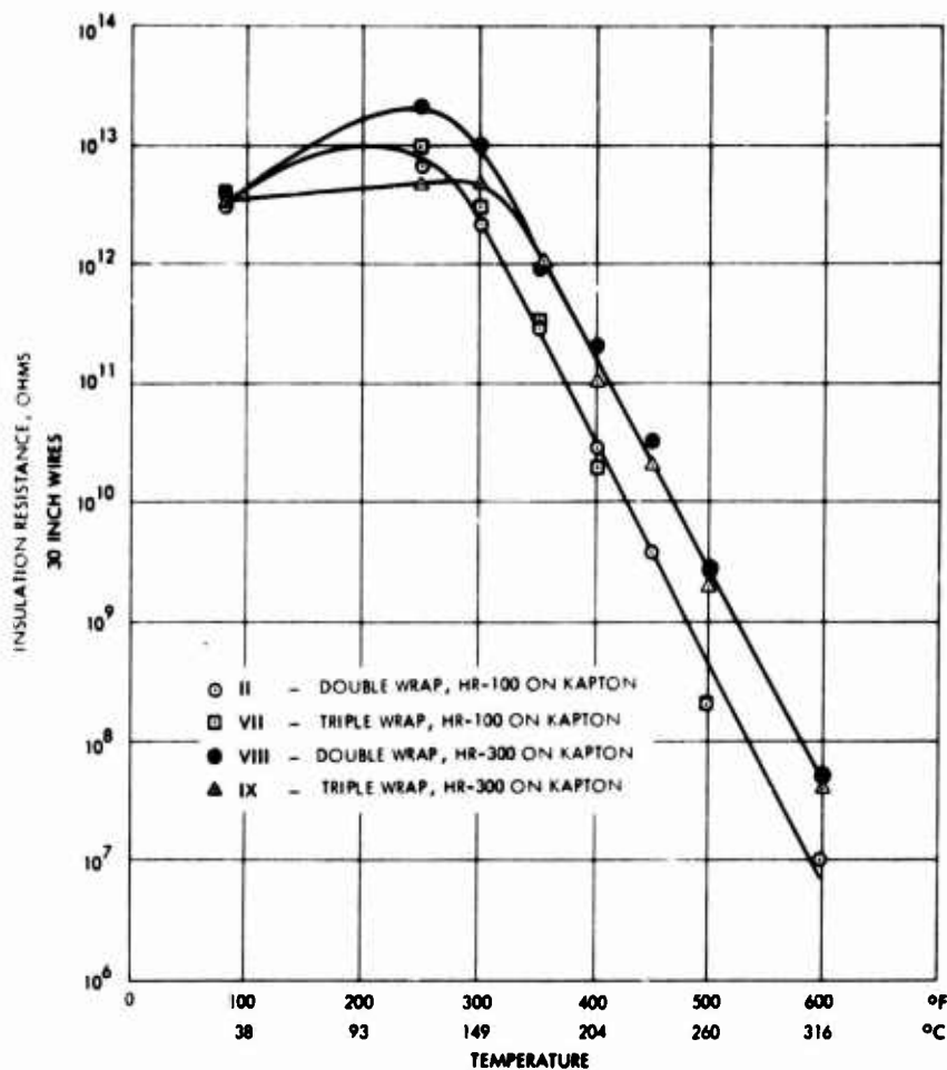
Figure 18. Insulation resistance as a function of temperature of HR-100 and HR-300 bonded Kapton insulated wires
