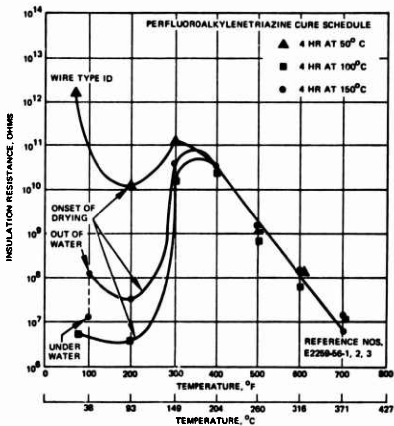
Figure 47. Insulation resistance of perfluoroalkylenetriazine overcoated "pyrrone"-Kapton wire as a function of temperature
