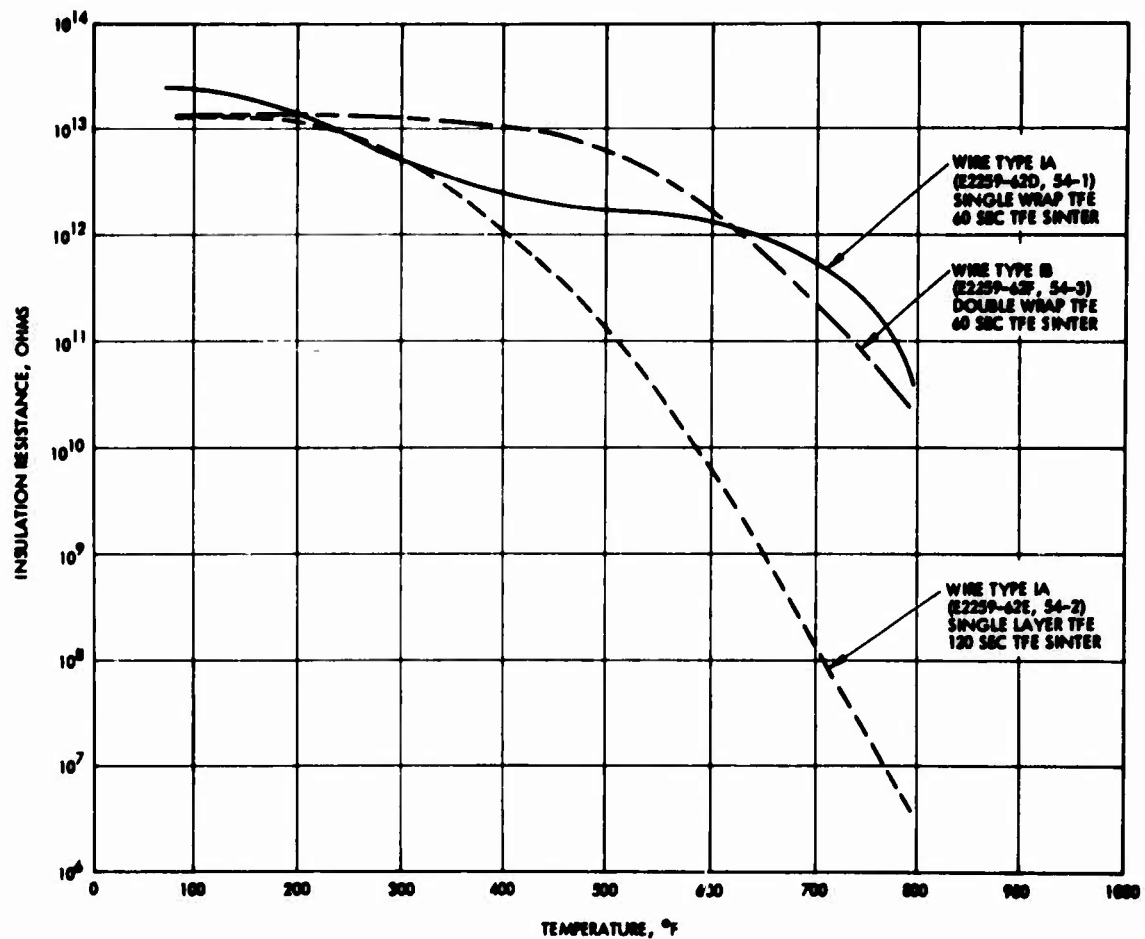
Figure 56. Insulation resistance of redried Teflon TFE overwrapped "pyrrone"-Kapton insulated wire after the 28-day exposure at 95 percent relative humidity
