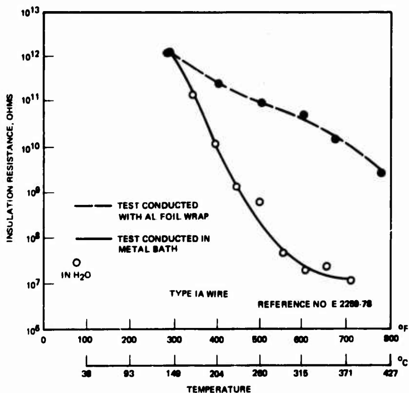
Figure 25. Insulation resistance of "pyrrone" - Kapton insulated wire with single Teflon over-coat (Wire Type IA)
