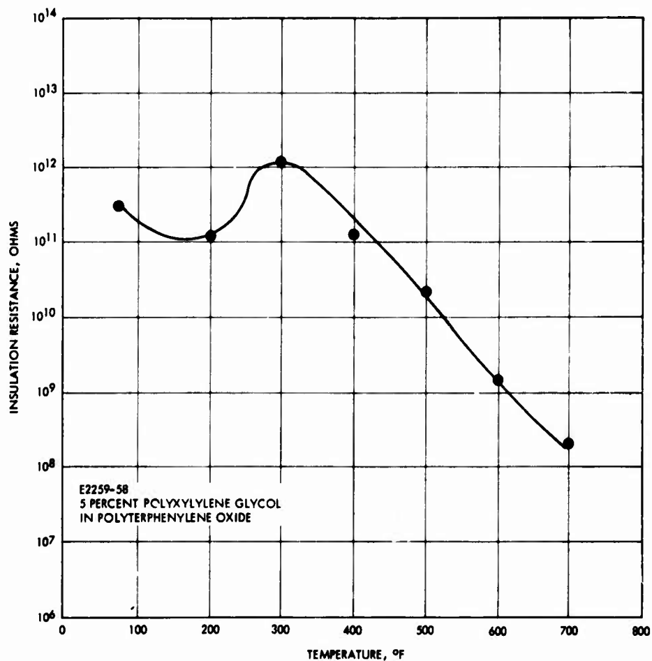
Figure 21. Insulation resistance of polyterphenyleneoxide coated wire as a function of temperature
