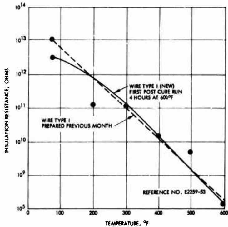
Figure 5. Insulation resistance of "pyrrone"-Kapton insulated wire
