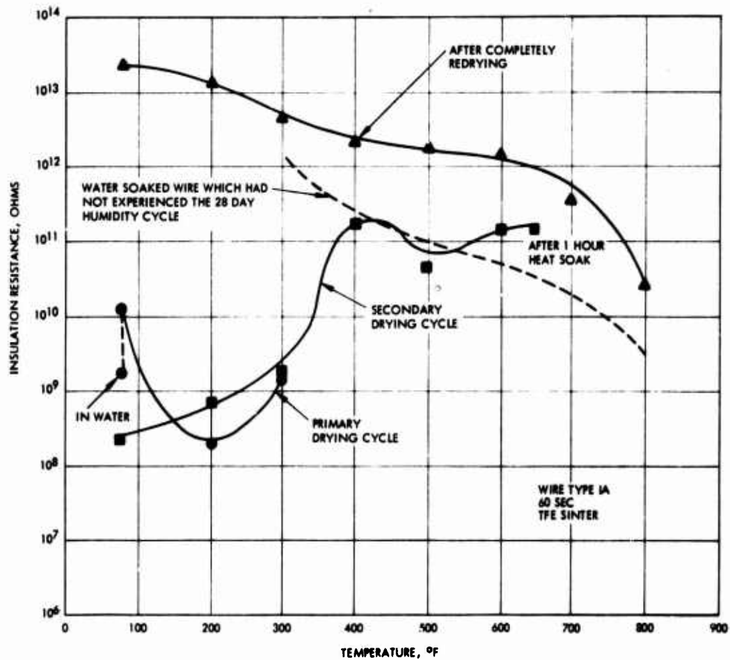
Figure 53. Insulation resistance of Teflon TFE overwrapped "pyrrone"-Kapton insulated wire after 28 days at 95 percent relative humidity (single wrap, 60 sec sinter)
