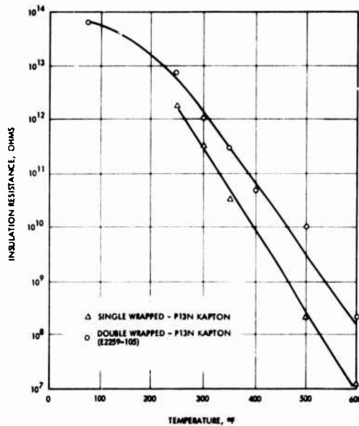
Figure 20. Insulation resistance of P13N-Kapton insulated wire as a function of temperature
