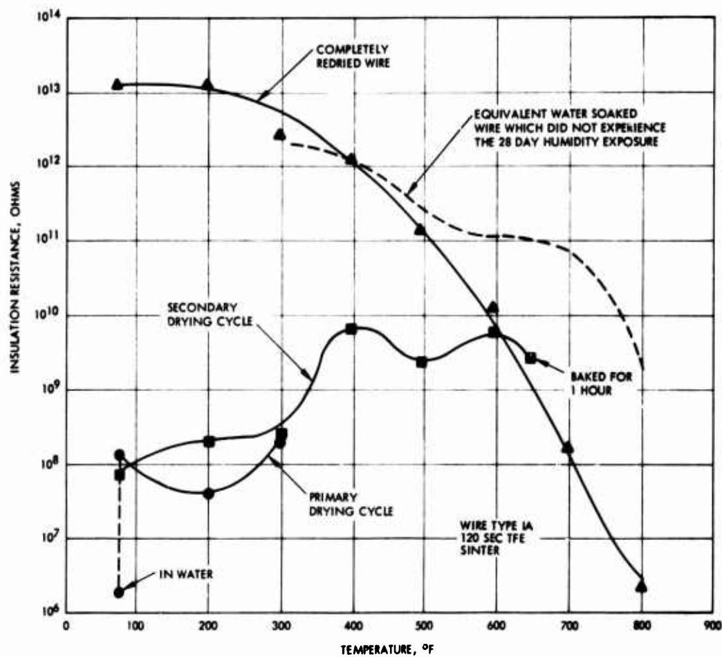
Figure 54. Insulation resistance of Teflon TFE overwrapped "pyrrone"-Kapton insulated wire after 28 days at 95 percent relative humidity (single wrap - 120 sec TFE sinter)
