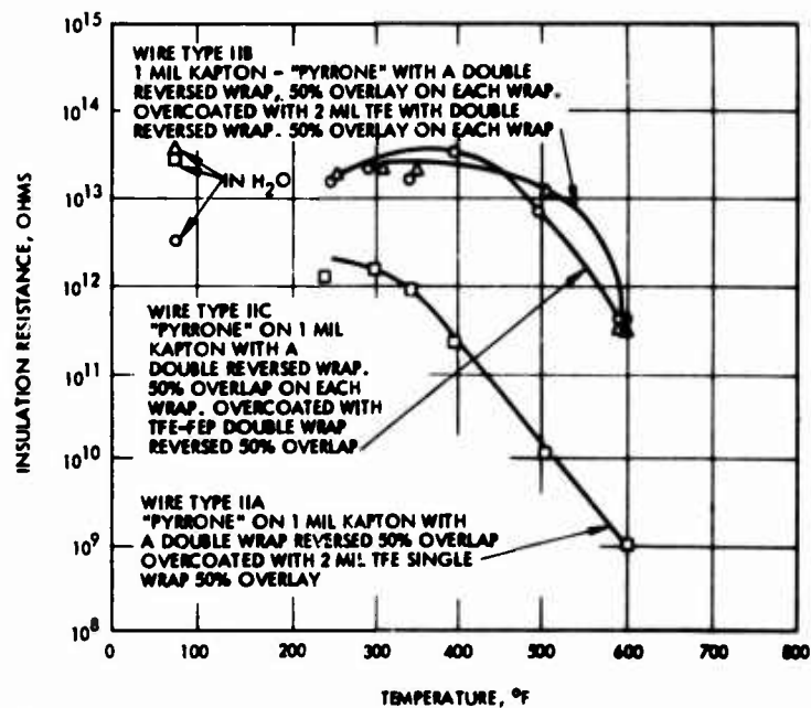
Figure 16. Insulation resistance of Teflon overcoated "pyrrone"-Kapton insulated wires as a function of temperature
