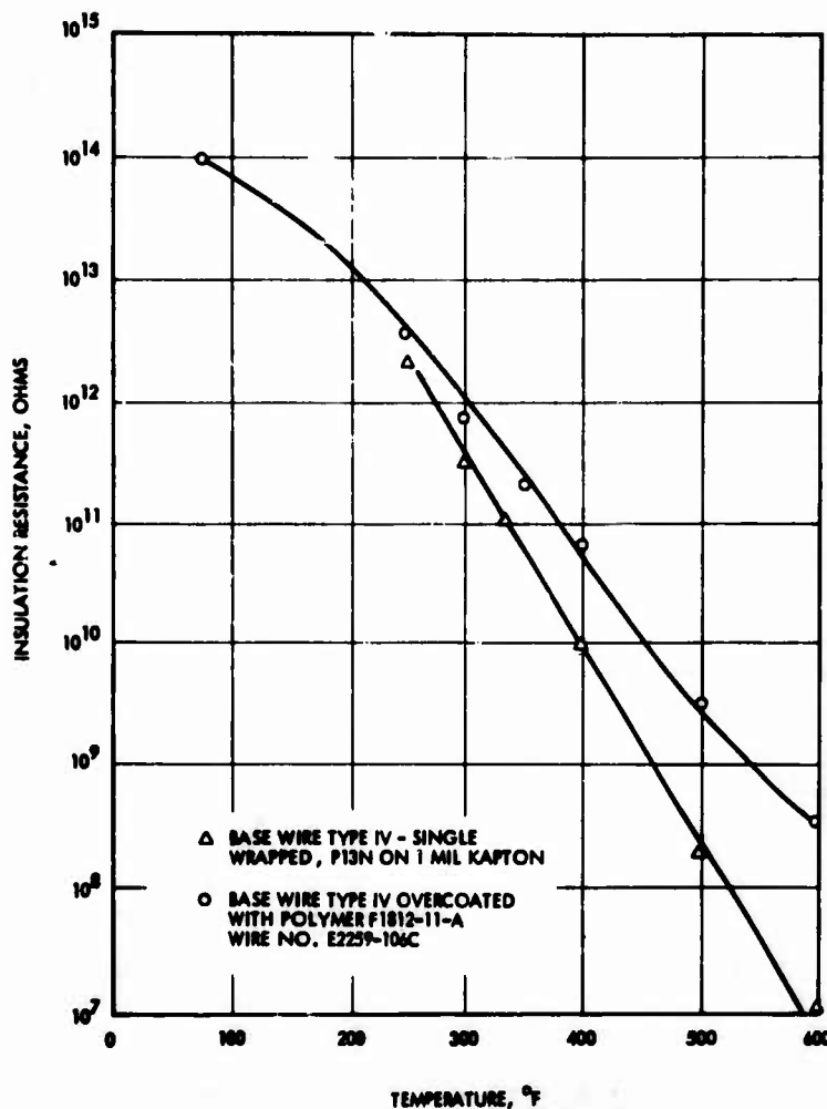
Figure 24. Insulation resistance versus temperature, Type IV wire overcoated with 1,3-bis(p-aminophenoxy) benzene based polyimide
