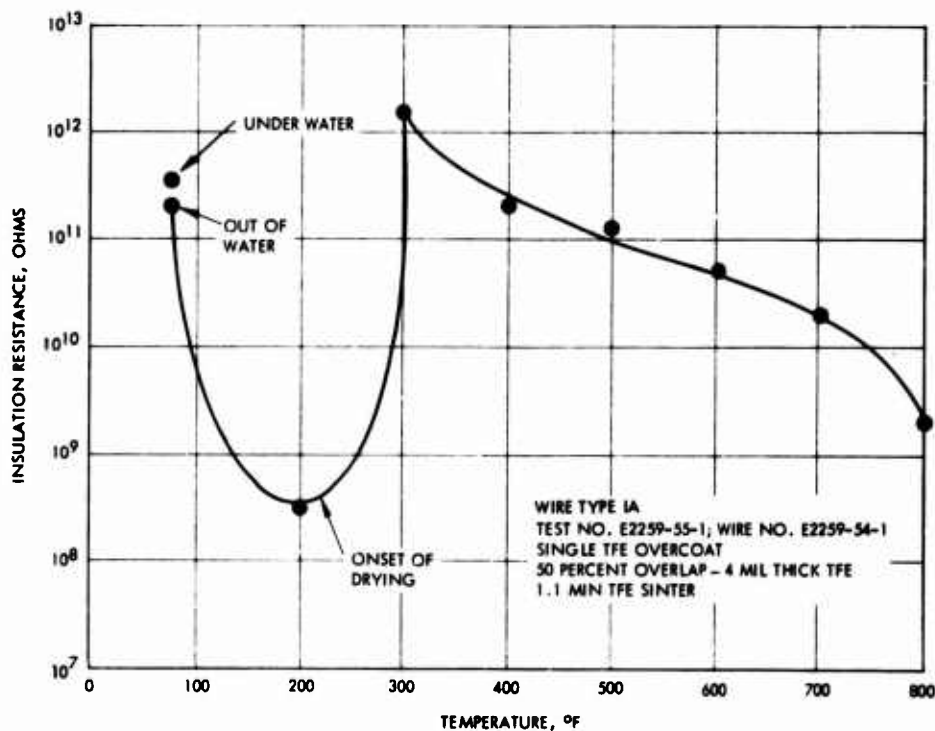
Figure 8. Insulation resistance of water-soaked Teflon TFE overcoated "pyrrone"-Kapton insulated wire - single overcoat - 1 minute sinter
