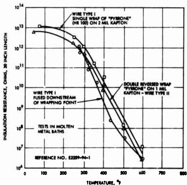
Figure 13. Insulation resistance of several "pyrrone"-Kapton insulated wires
