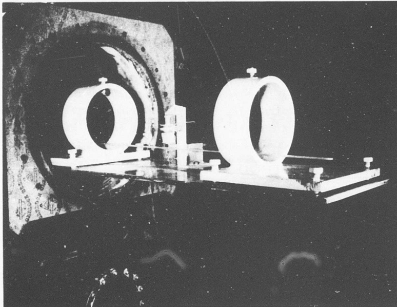
Figure 1. Free-Free Test Apparatus.
