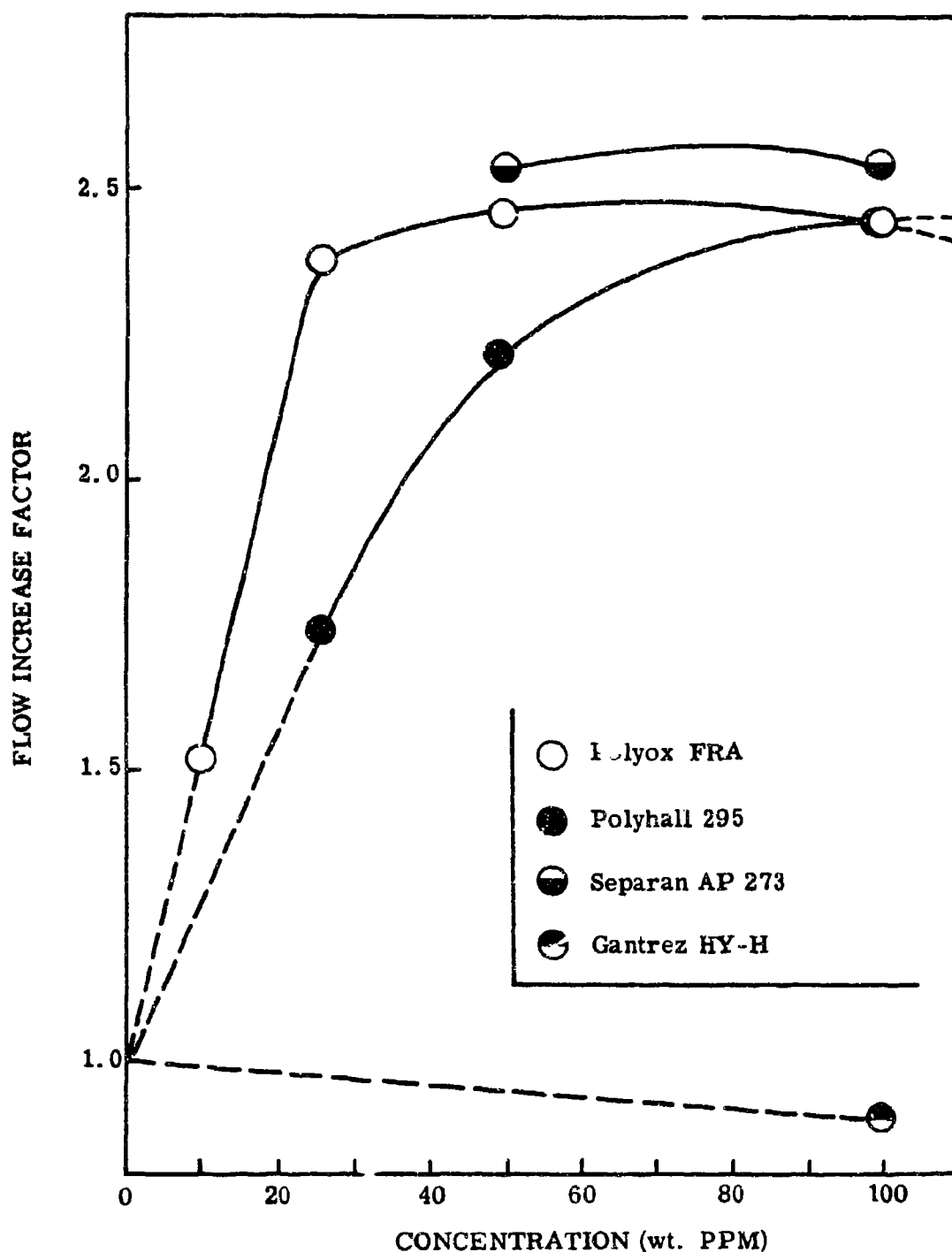
Figure 4 Concentration vs. Flow Increase Factor for Polyox FRA, Polyhall 295, Separan AP 273, and Gantrez HY-H. Differential pressure maintained at 12.6 \pm 1.0 in. of mercury, \Delta L = 20 ft., I.D. = 0.622 in., N_r = 3.2 - 8.1 \times 10^4 (Dashed lines are extrapolations)
