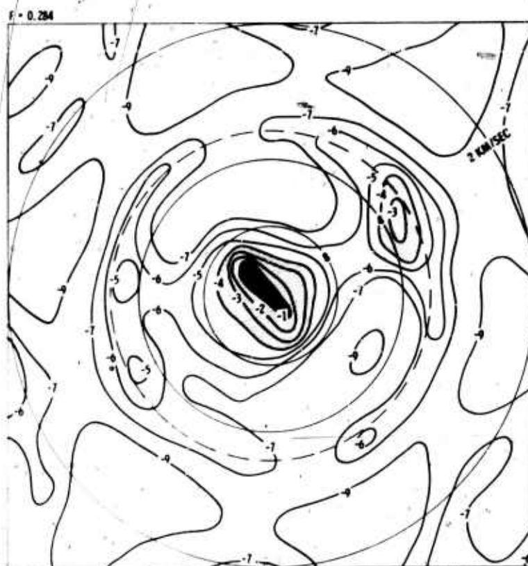
Figure IV-12. High Resolution Wavenumber Spectra of .244 and .284 Hz 'winter' Noise
