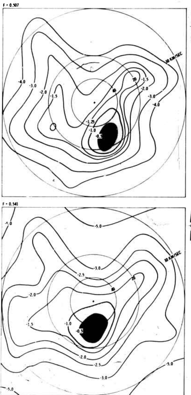
Figure IV-8. High Resolution Wavenumber Spectra of 'summer' P-Wave Noise at .507 and .541 Hz
