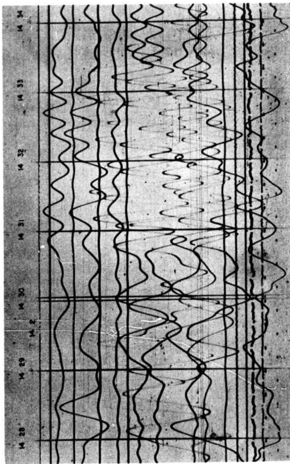
Figure 15. Reproduction of a 16 mm film recording of a Rayleigh wave train from an earthquake off the coast of Ecuador. \theta = 1408:54 , 2.5N , 83.0W , h = ? , m_b = 4.4 , \Delta = 42 deg, azimuth \approx 135 deg.
