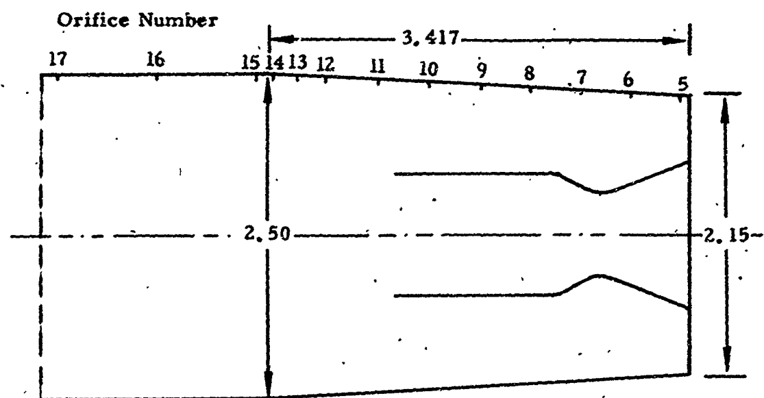
Conical Nozzle 2.7-20-.45 With Boattail Afterbody
