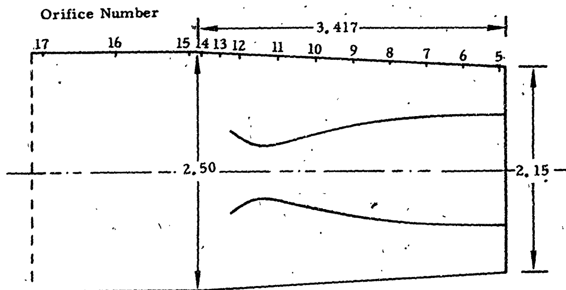
Contour Nozzle 3.0-0-.456 With Boattail Afterbody
