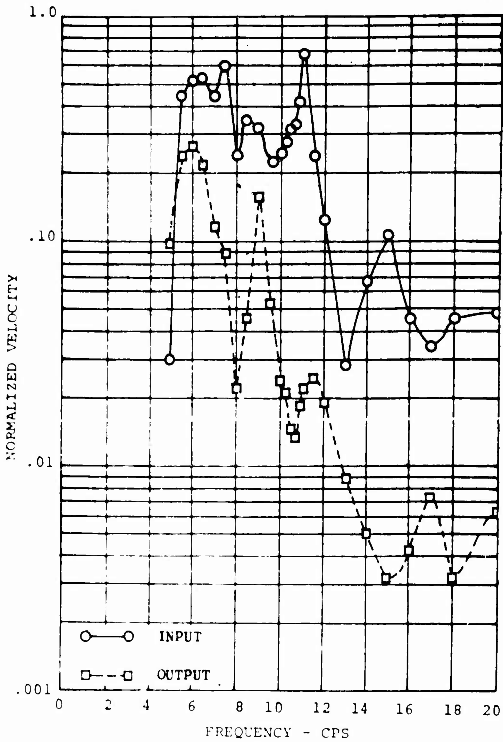
Figure 38. Normalized Longitudinal Velocity of the 160-Pound Three-Dimensional DAV 1 Platform for a Non-Orthogonal Excitation.
