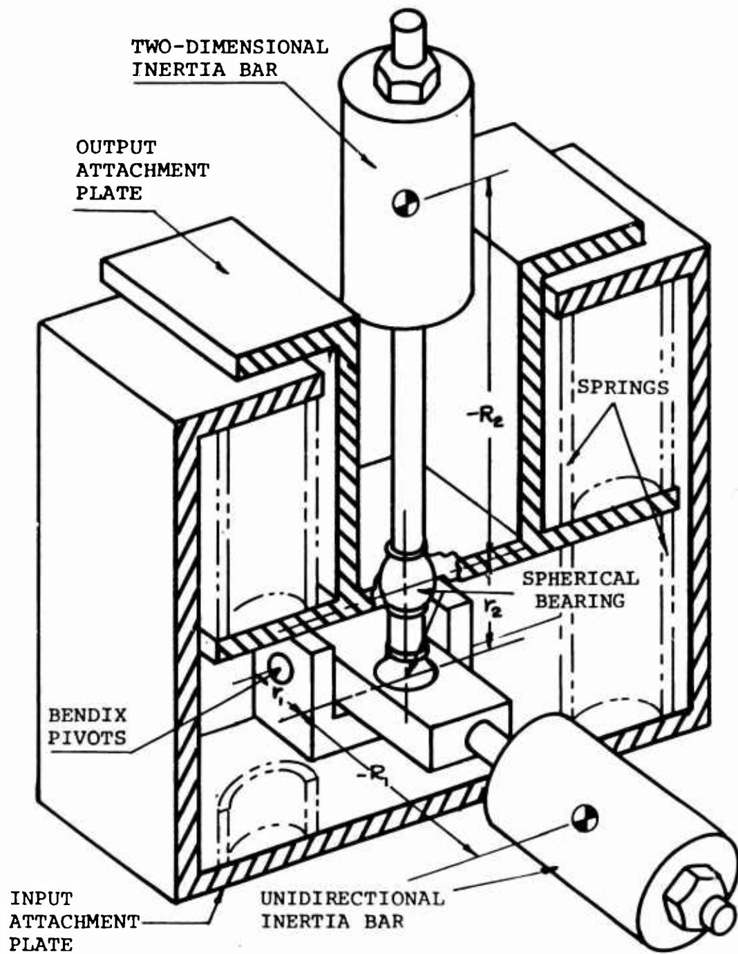
Figure 6. Schematic of the Improved Three-Dimensional DAVI Model.
