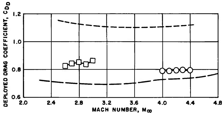
Fig. 6 Effect of Free-Stream Mach Number on the AID Drag Coefficient; \alpha = 0
