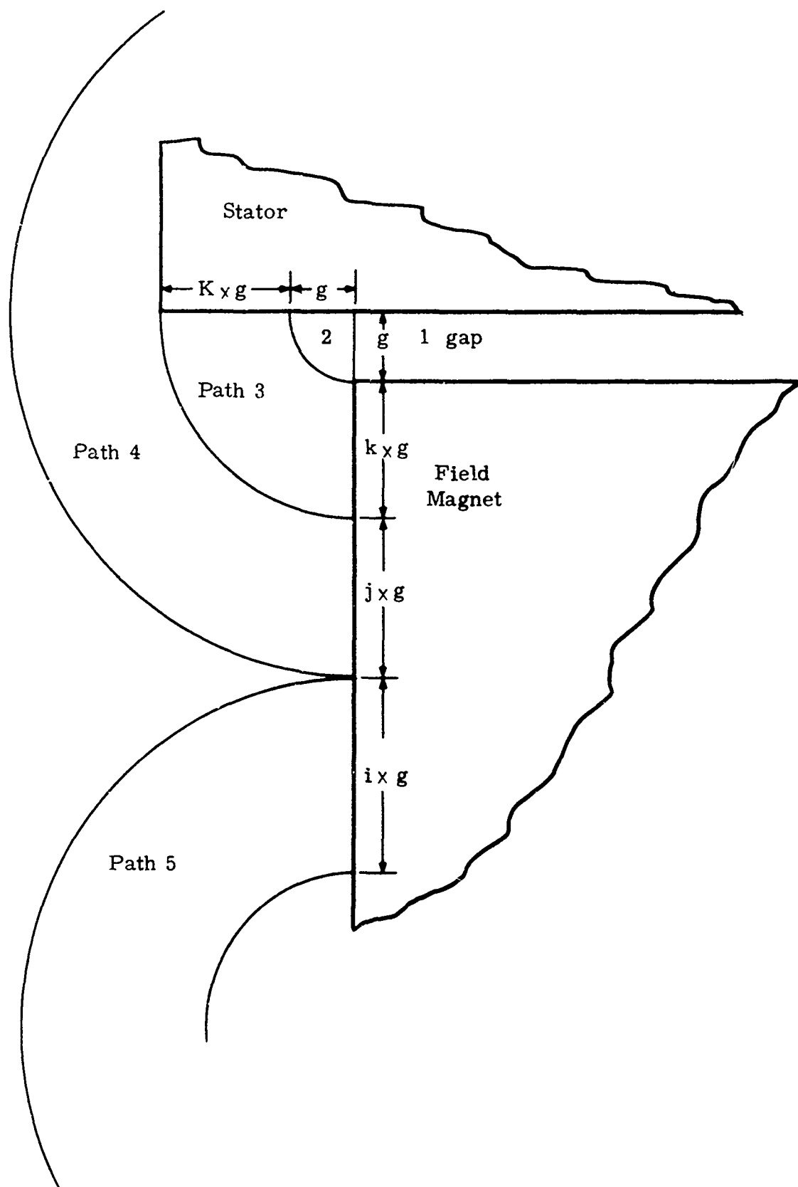
Figure 2.1.1.1-2. Permeance Paths
