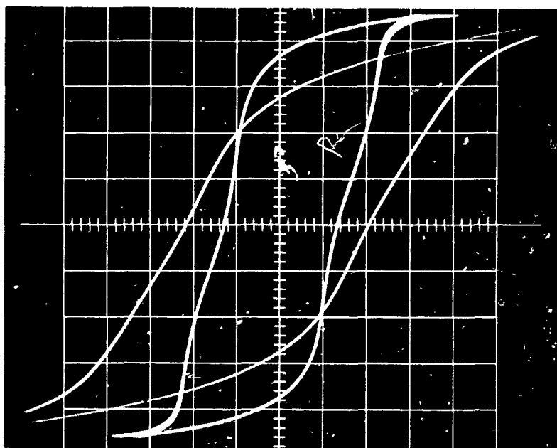
Figure 2.1.1.14.4-7. Outer Loops of Figures 2.1.1.14.4-5 and 2.1.1.14.4-6 Superimposed
