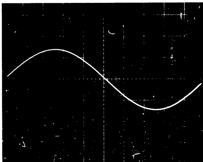
Figure 4.1.4.2-8. Black Lead, Voltage Waveform across 2985-ohm Resistor, 66.9 Watts, Room Temperature, 180,120 Rpm, Oscilloscope Sensitivity 50 Volts per Centimeter
