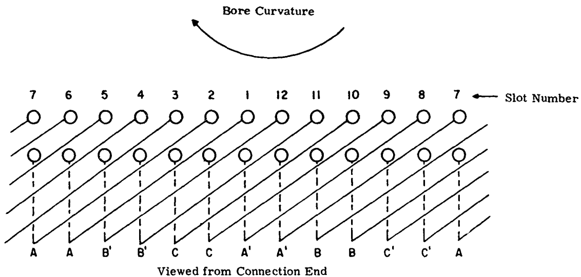
Figure 3.2-4. Five-sixth Pitch -- Twelve Coils
