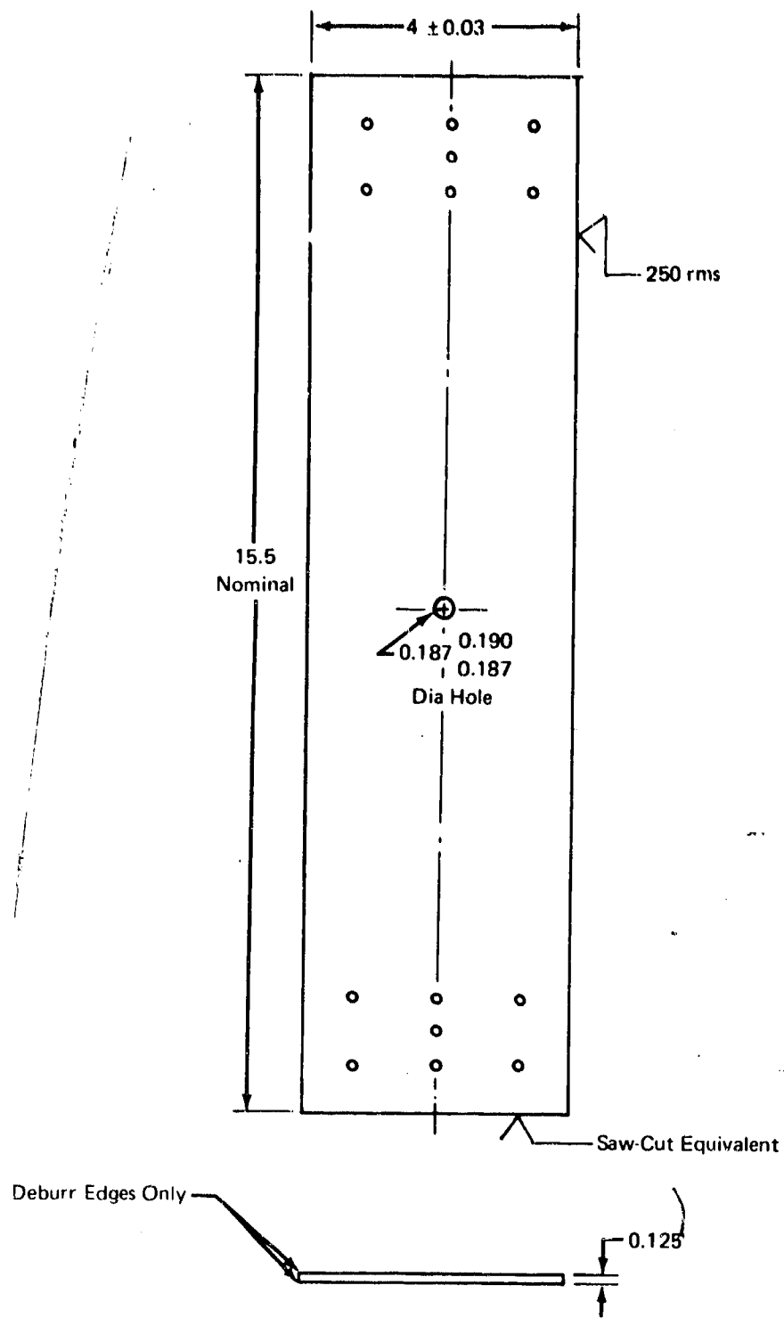
Figure 8. Single-Hole Specimen
