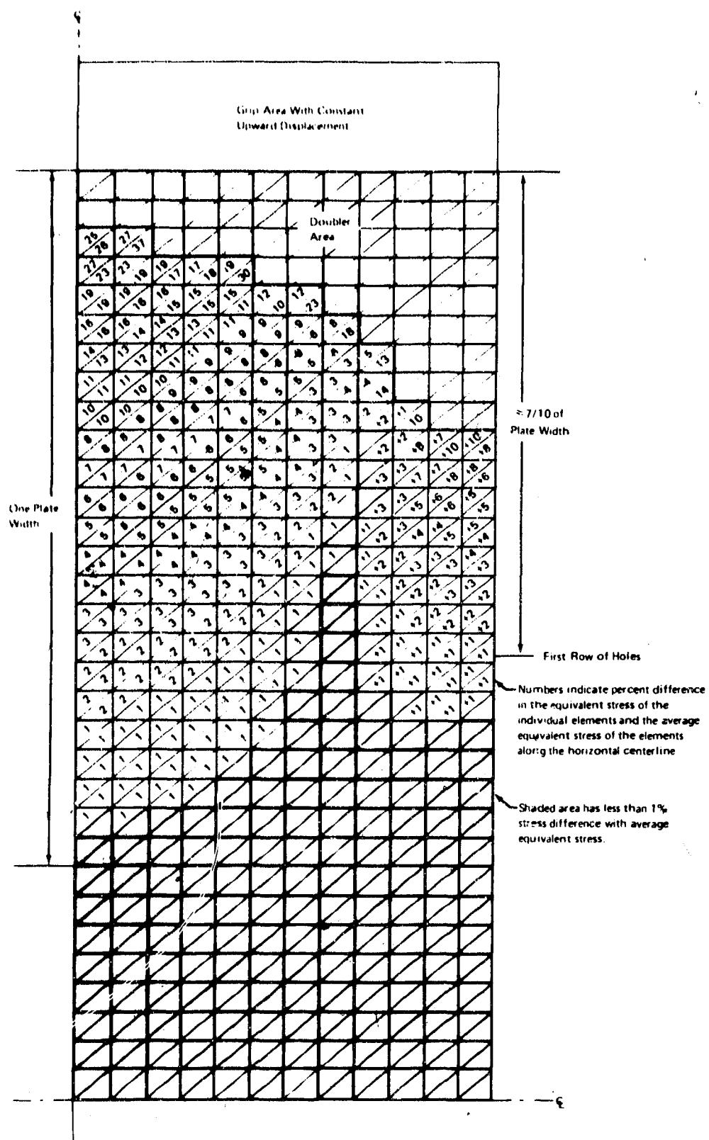
Figure 12. Computed Stress Variations for Panel With U-Shaped Doublers (Final Configuration)
