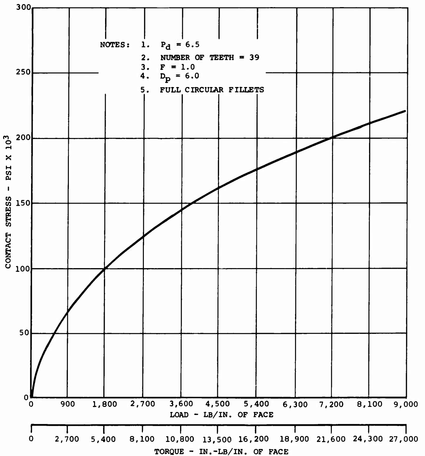
Figure 28. Contact Stress of Baseline Standard Involute Helical Gears
