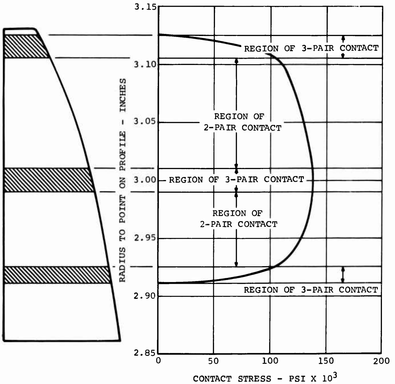
Figure 61. Contact Stress Distribution of 9-Pitch, High-Contact-Ratio Spur Gears
