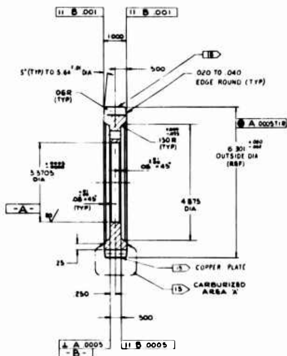
DETAIL 'M'
