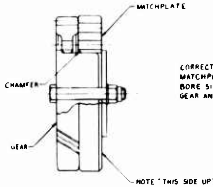
DETAIL 'M'
