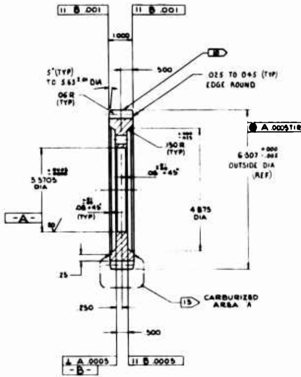
DETAIL 'M'
