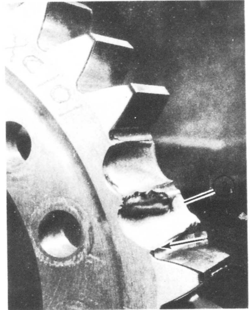
Figure 38. Fracture Surface of Second Tooth Failure. Arrow Indicates Origin Location in Drive Root Fillet Area.
