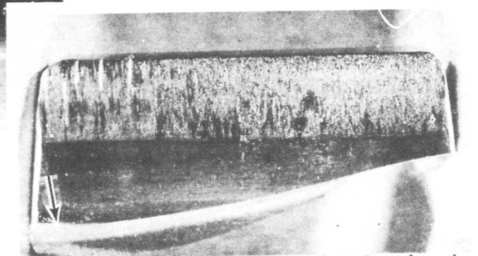
Figure 41. Contact Pattern of Second Failed Tooth Showing Addendum Scuffing
