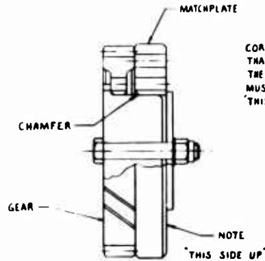
DETAIL M
