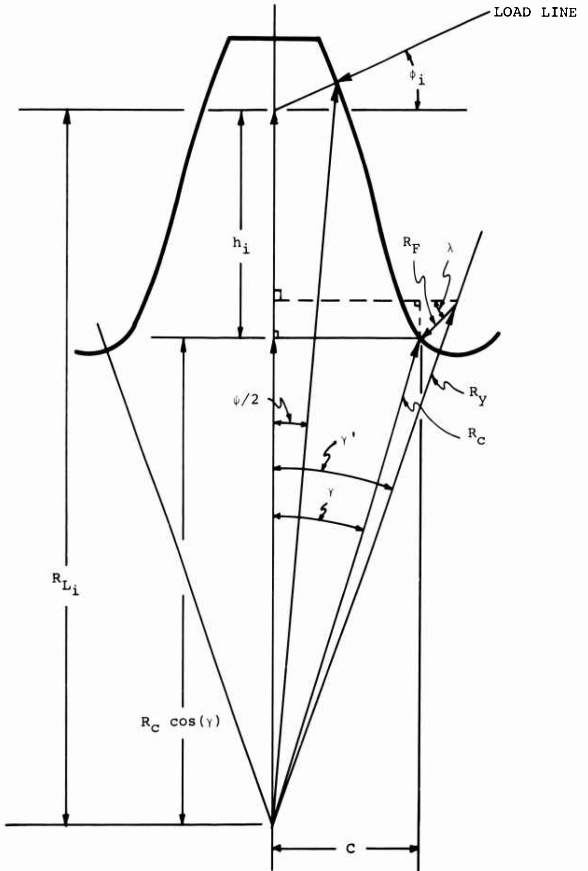
Figure 62. Schematic Diagram for Gear Tooth Calculations
