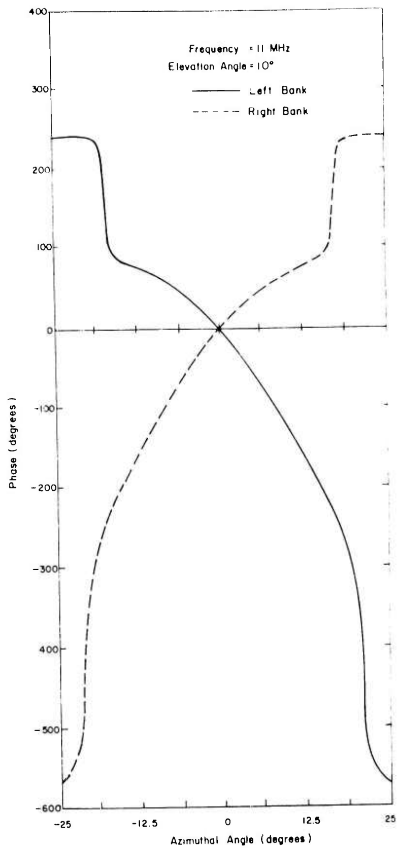
Figure 9. Phase pattern, single wave case.
