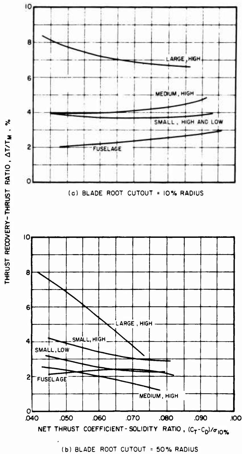
Figure 12. Variation of Thrust Recovery-Thrust Ratio With Net Thrust.
