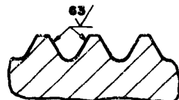
SECTION THRU THREAD PROFILE
