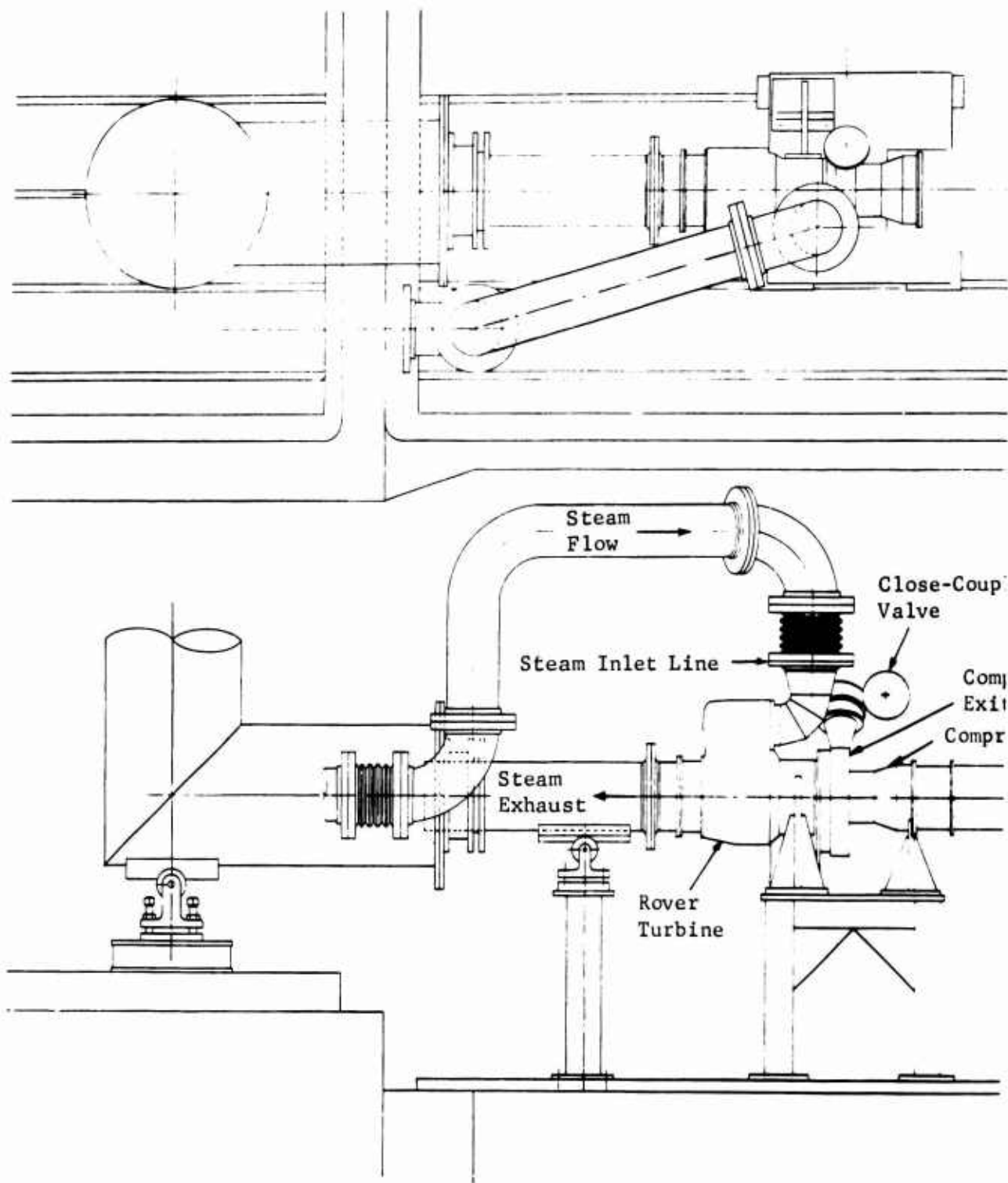
Figure 38. Compressor Test Rig Installation.
