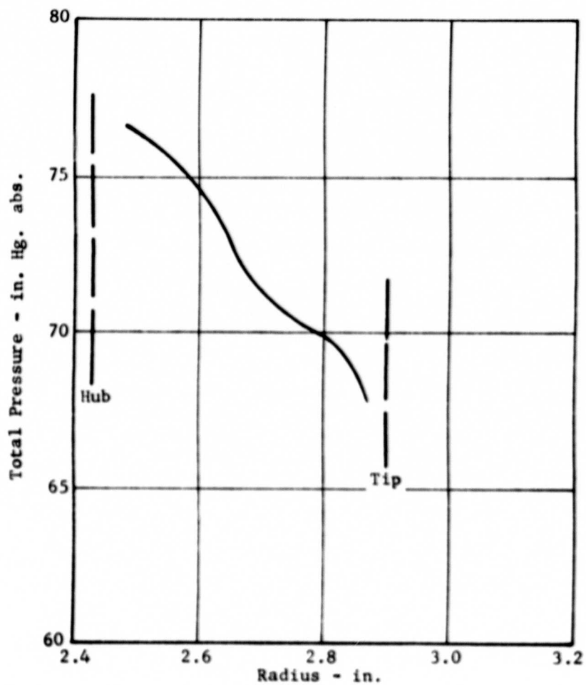
Figure 32. Build 20 Rotor Exit Pressure Traverse Data for N/\sqrt{r} = 90 Percent, (W\sqrt{r})/8 = 3.49 lb/sec, and P_T/P_T = 2.31 .
