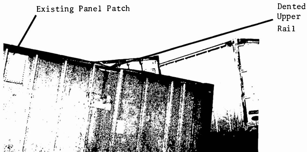
Figure 5-7. Typical Top Rail Damage
