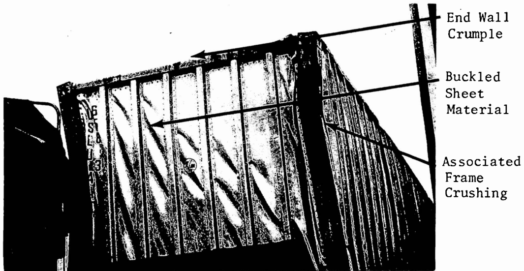
Figure 5-13. Typical Major Panel Damage
