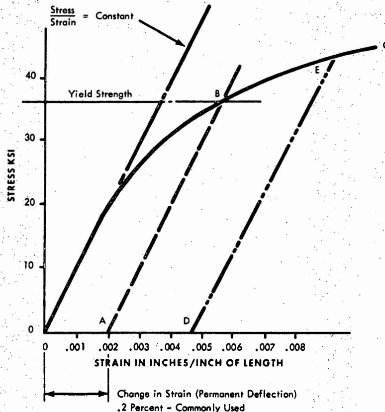
Figure 6-3. Stress-Strain Curve
