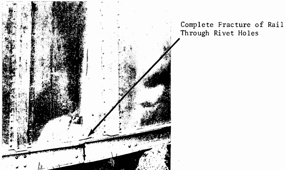
Figure 5-4. Typical Bottom Rail Damage
