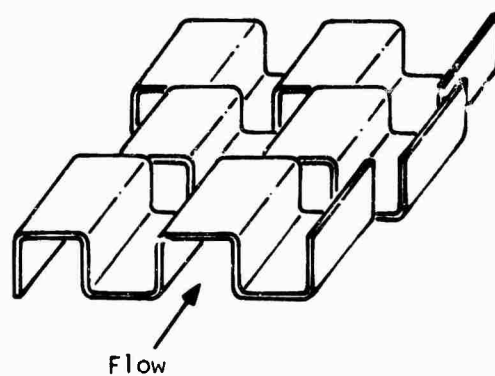
c) Enlarged view of a typical rectangular offset-fin heat transfer surface
