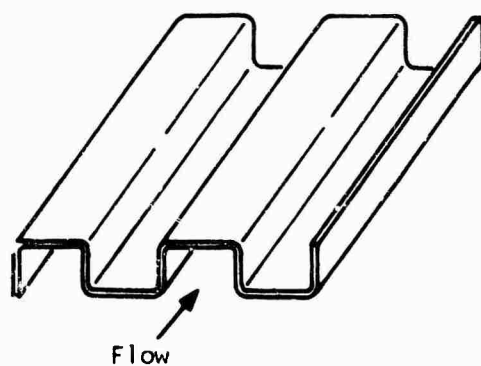
b) Enlarged view of typical plain rectangular fin heat transfer surface
