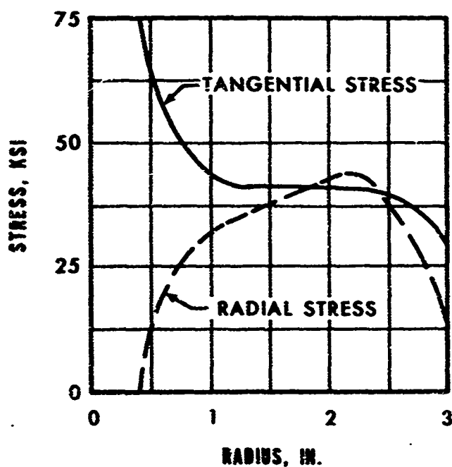
Figure 11. Preliminary Disk Shape and Calculated Centrifugal Stresses of First-Stage Turbine.
