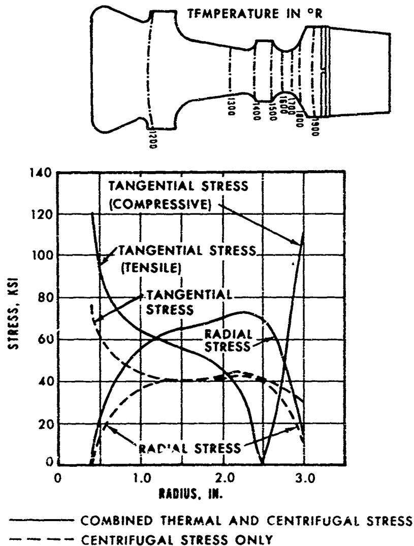
Figure 17. Preliminary Centrifugal- and Thermal-Stress Distributions of First-Stage Rotor Disk.
