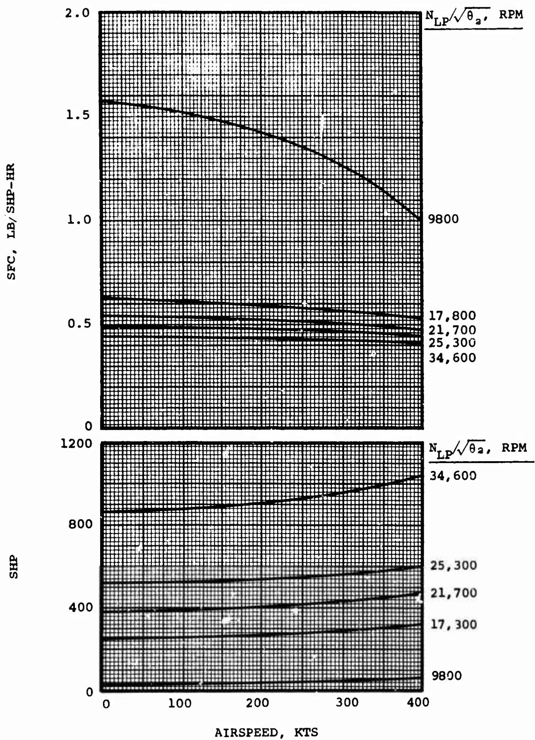
Figure 89. Shaft Horsepower and SFC Versus Airspeed for 3S-RF-TSE at 6000 Feet, Standard-Day Conditions.
