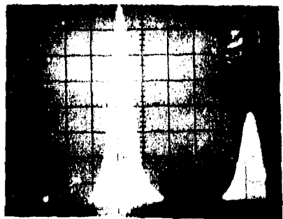
Spectrum in Gate D Linear Scale 6 MHz Center Frequency 300 KHz Bandwidth 1 MHz/div
