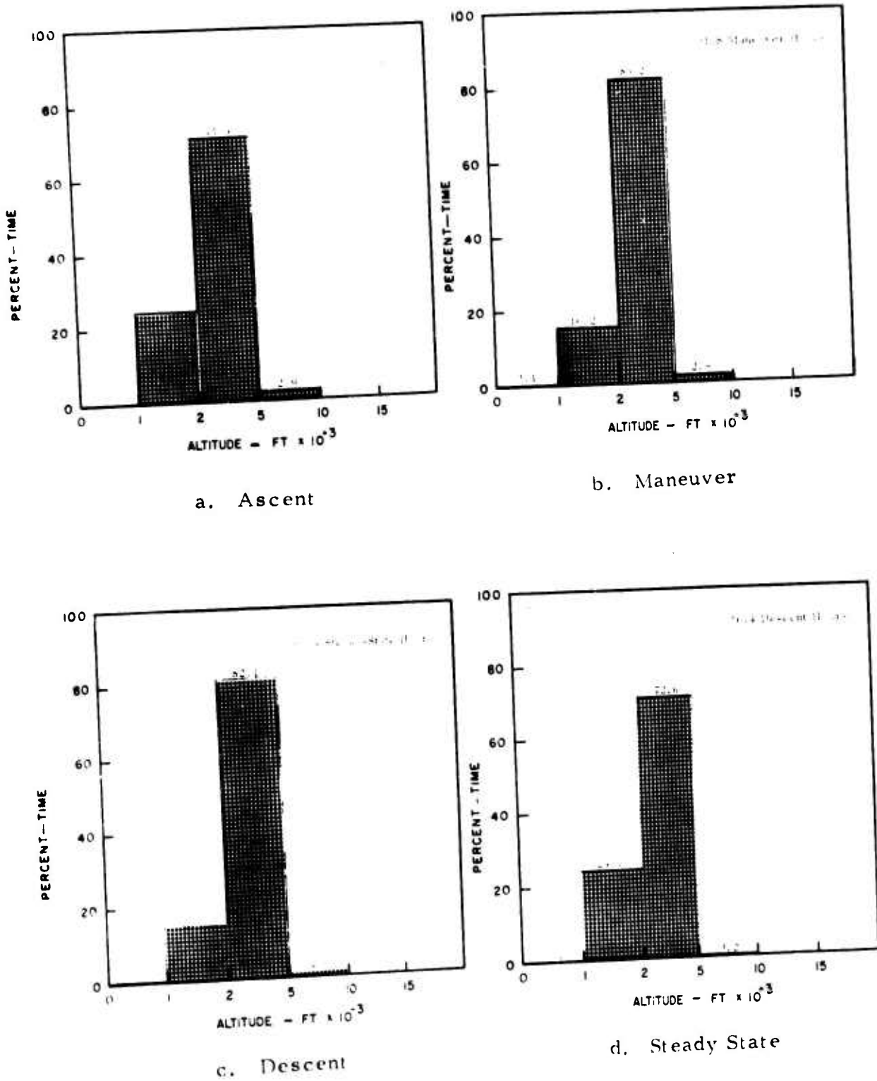
Figure 12. Flight Time in Each Mission Segment Broken Down by Percentage of Time in Each Altitude Range (Sample II).
