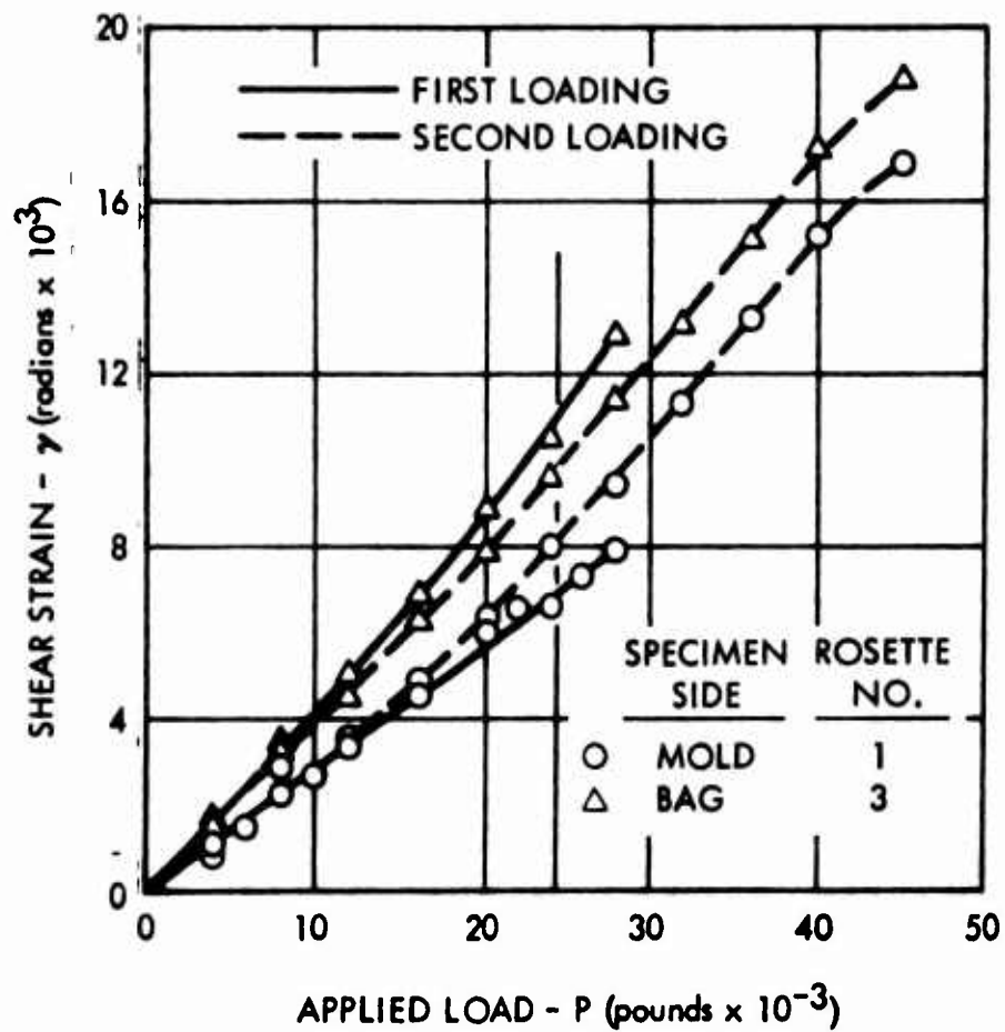
Figure 15. Shear Strains in Constant-Thickness Sandwich Specimen 132 - Seven Inches From Mid-Span.
