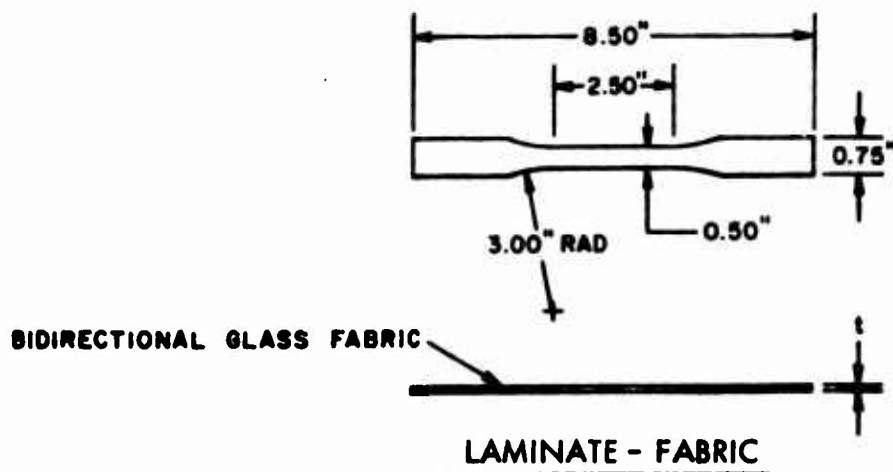
Figure 1. Laminate Tensile Specimens.
