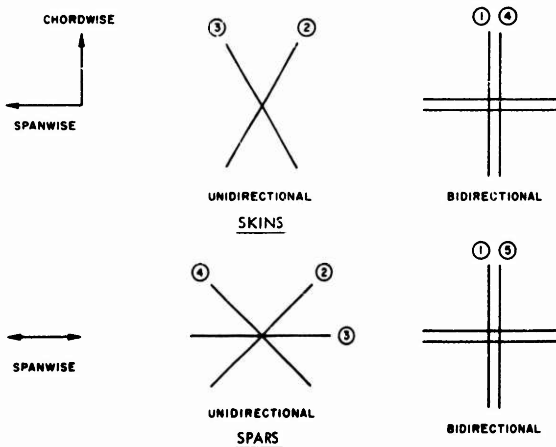
Figure 25. Test Section Ply Orientations.
