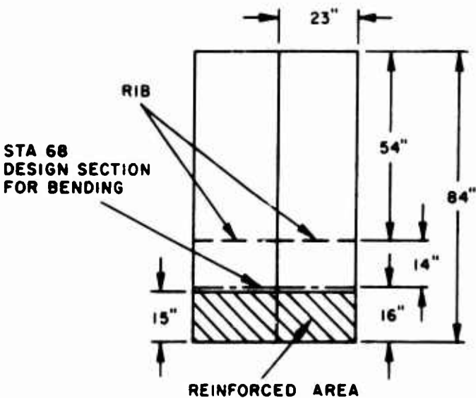
Figure 56. Rib Location.
