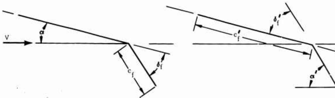
Geometry for Airfoil With a Trailing Edge Flap
