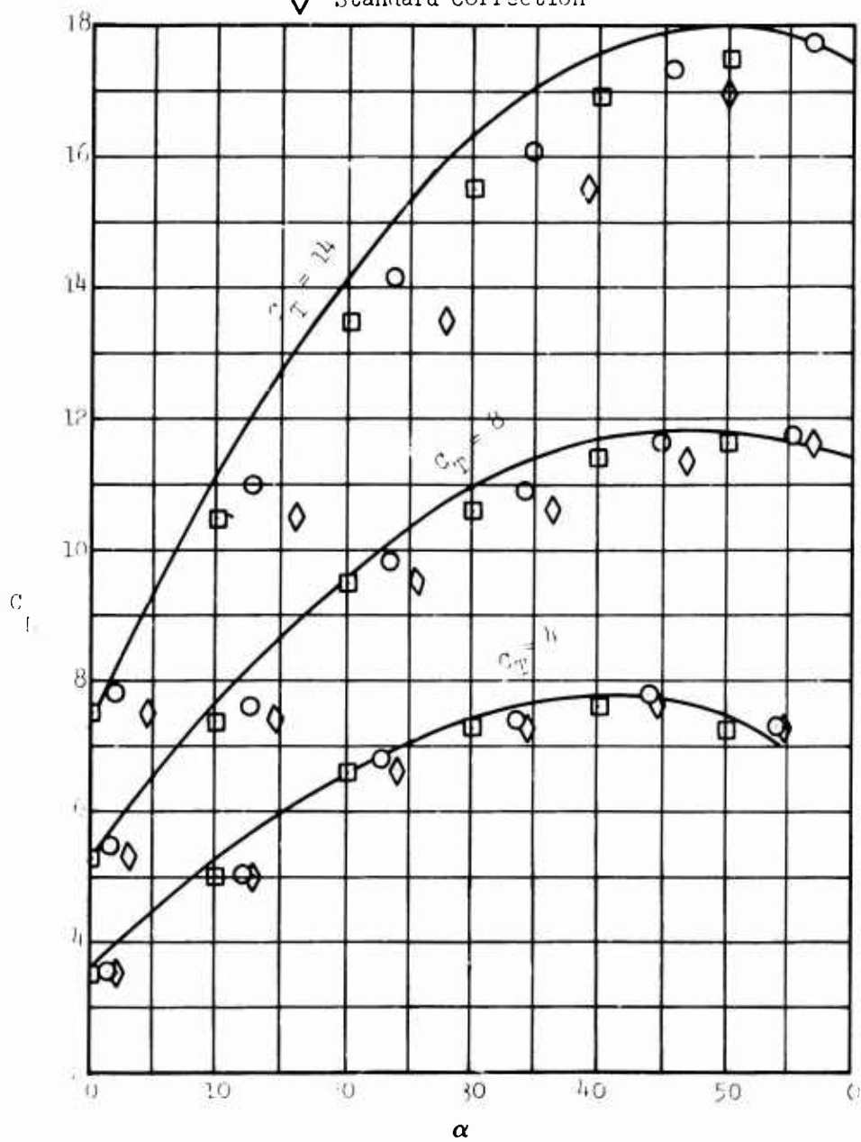
Figure 40. The Effect of Wind Tunnel Wall Corrections to Lift Coefficient Data From Reference 56.
