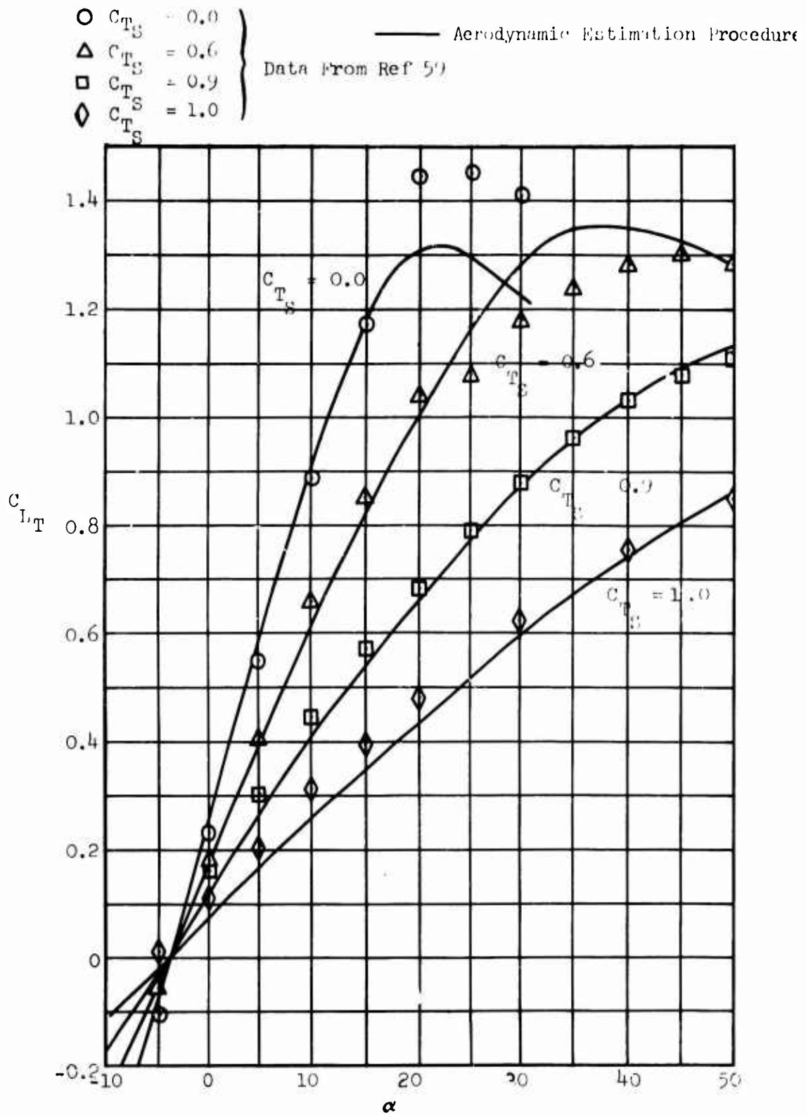
Figure 46. Total Lift Coefficient Versus Wing Angle of Attack, \delta_f = 0^\circ .
