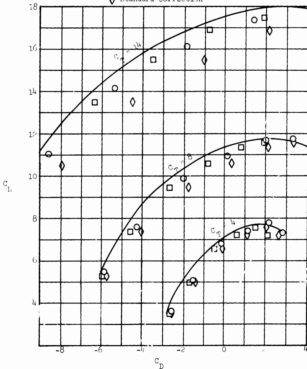
Figure 41. The Effect of Wind Tunnel Wall Corrections to Drag Coefficient Data From Reference 56.
