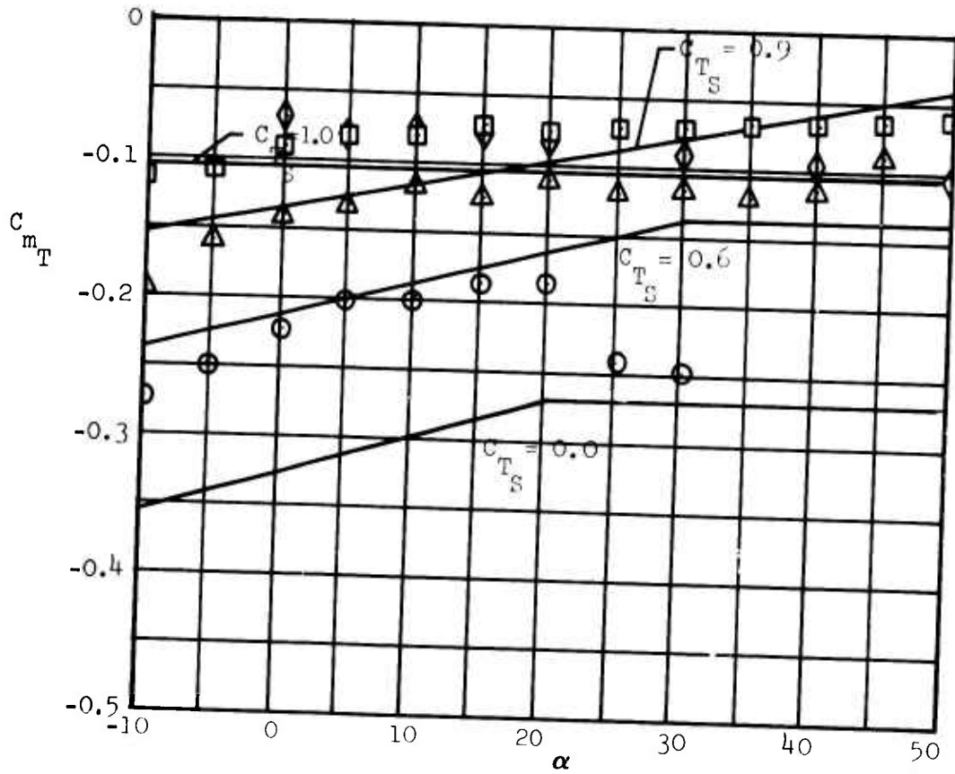
Figure 51. Total Pitching Moment Versus Wing Angle of Attack, \delta_f = 20^\circ .
