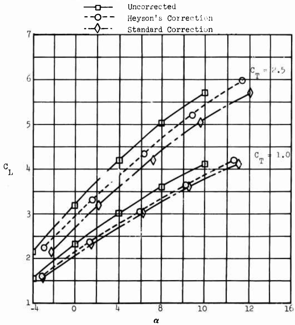
Figure 42. The Effect of Wind Tunnel Wall Corrections to Lift Coefficient Data From Reference 57.
