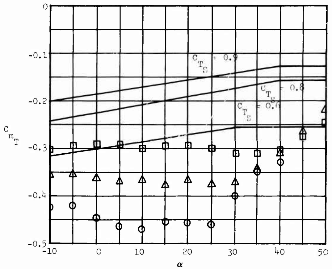
Figure 57. Total Pitching Moment Versus Wing Angle of Attack, \delta_f = 40^\circ .
