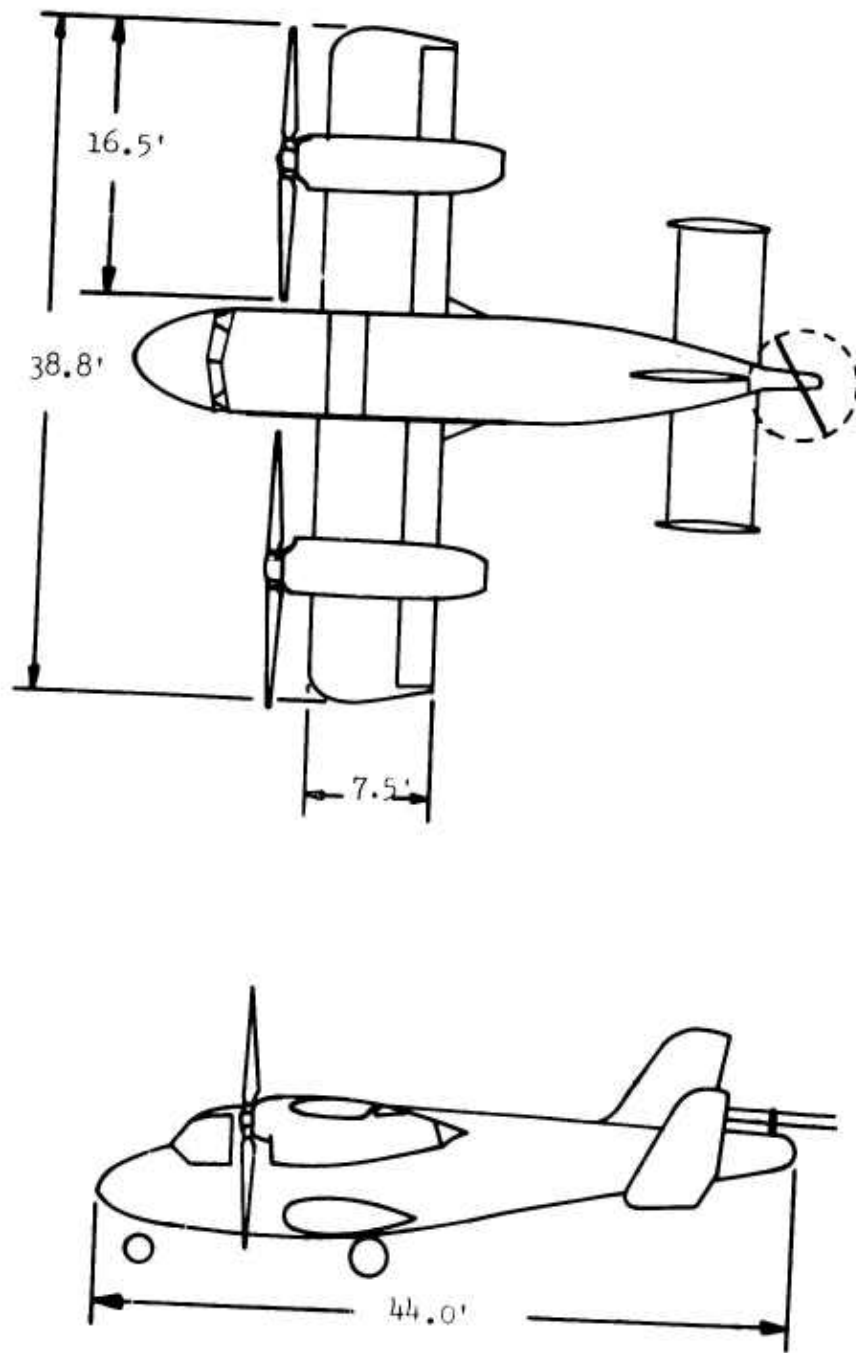
Figure 68. General Arrangement of Tilt-Wing Aircraft.
