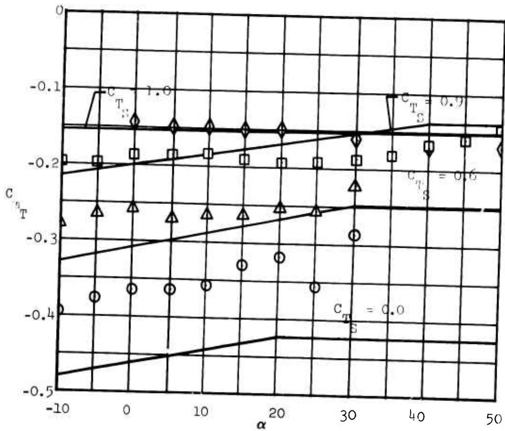
Figure 54. Total Pitching Moment Versus Wing Angle of Attack, \delta_f = 50^\circ .
