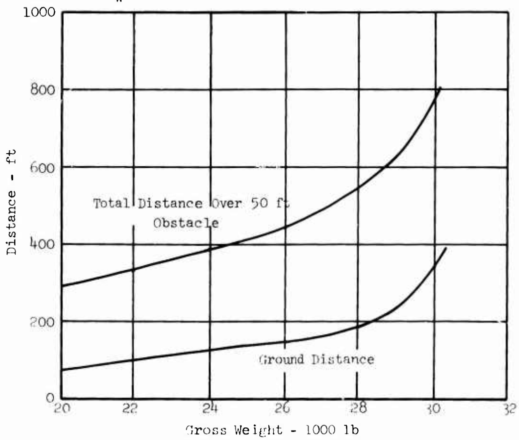
Figure 75. Deflected-Slipstream Takeoff Distance Versus Gross Weight.
