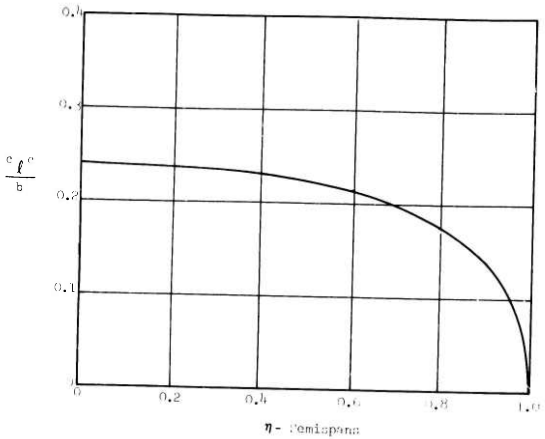
Figure 36. Span Load Distributions and Downwash for Model.
