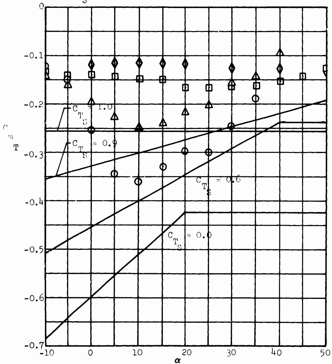
Figure 60. Total Pitching Moment Versus Wing Angle of Attack, \delta_f = 40^\circ , \delta_s = 20^\circ .
