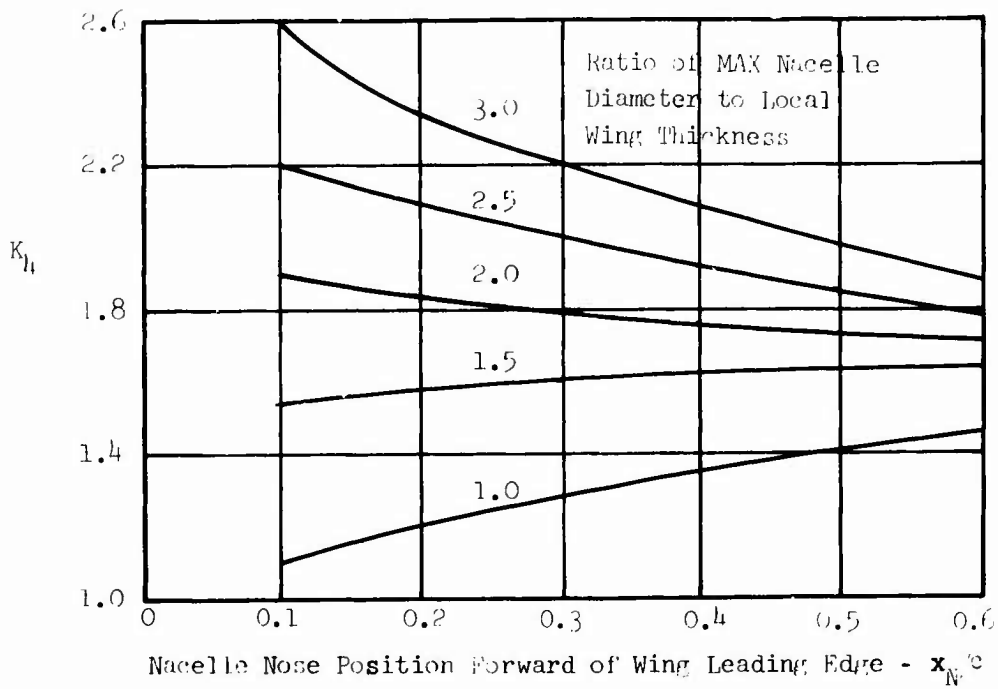
Figure 25. Nacelle-Wing Interference Drag Factors.
