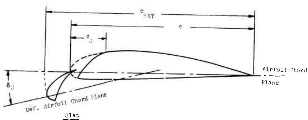
Figure 18. Geometry for Leading Edge Devices.
