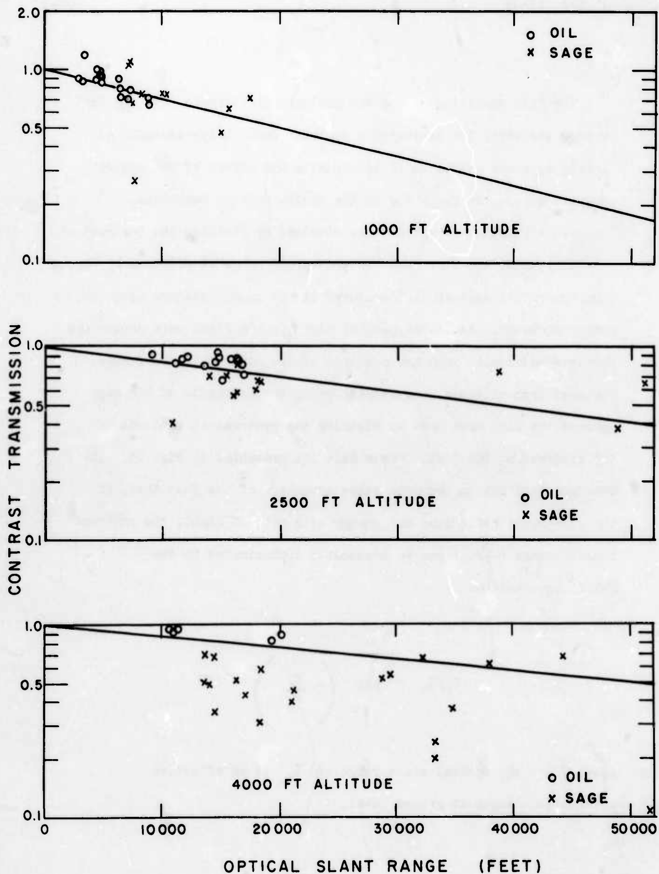
FIGURE 25 - CONTRAST TRANSMISSION OF THE ATMOSPHERE
