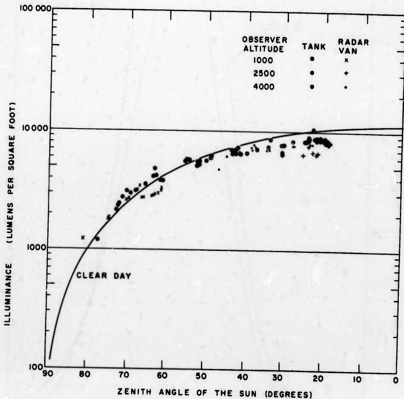
FIGURE 20 - ILLUMINATION DURING SIGHTINGS
