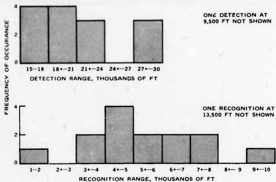
FIG. 2. Distribution of Scores for Flights Against a Radar Van.
