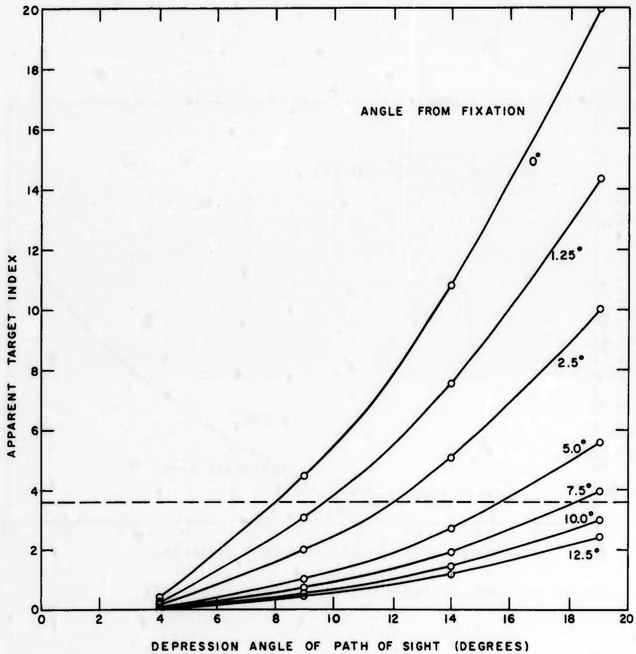
FIGURE 28 - PREDICTIONS OF VISUAL RESPONSE TO THE RADAR VAN FOR THE OBSERVER AT AN ALTITUDE OF 4000 FEET
