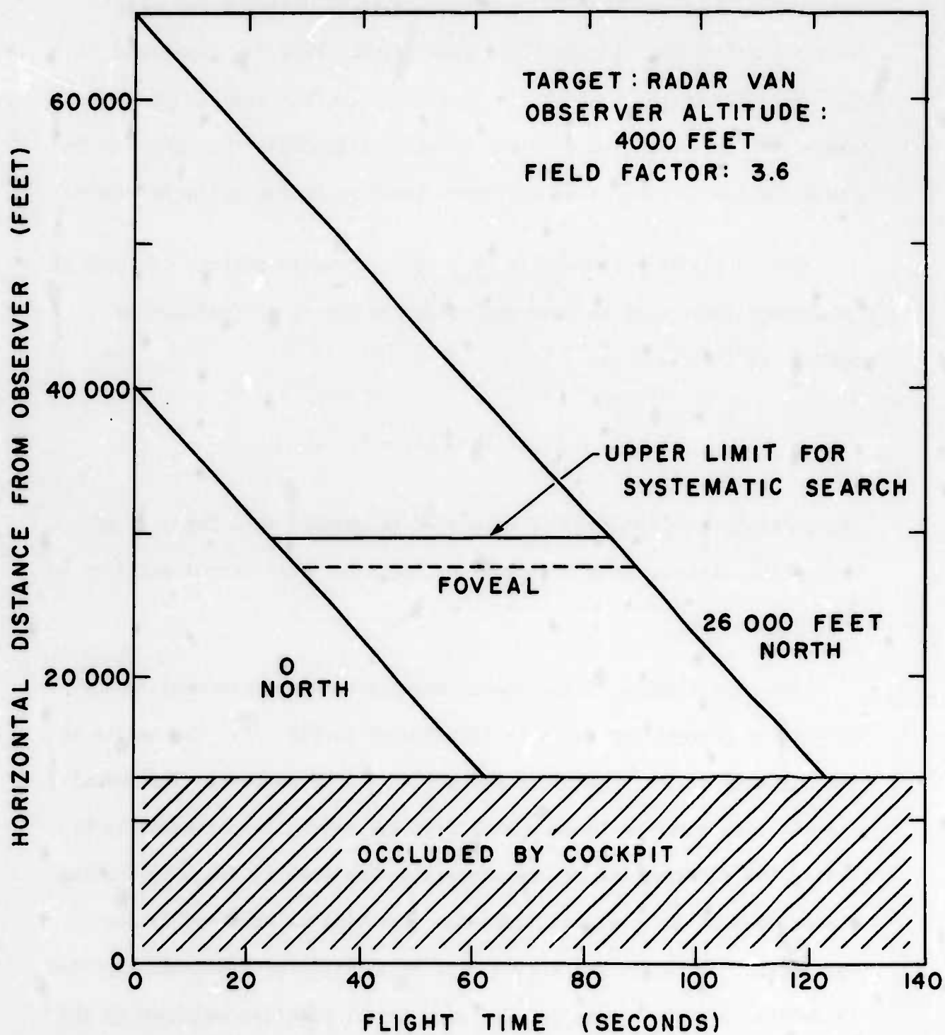
FIGURE 32-LINEAR REPRESENTATION OF THE FIELD OF VIEW AS A FUNCTION OF FLIGHT TIME
