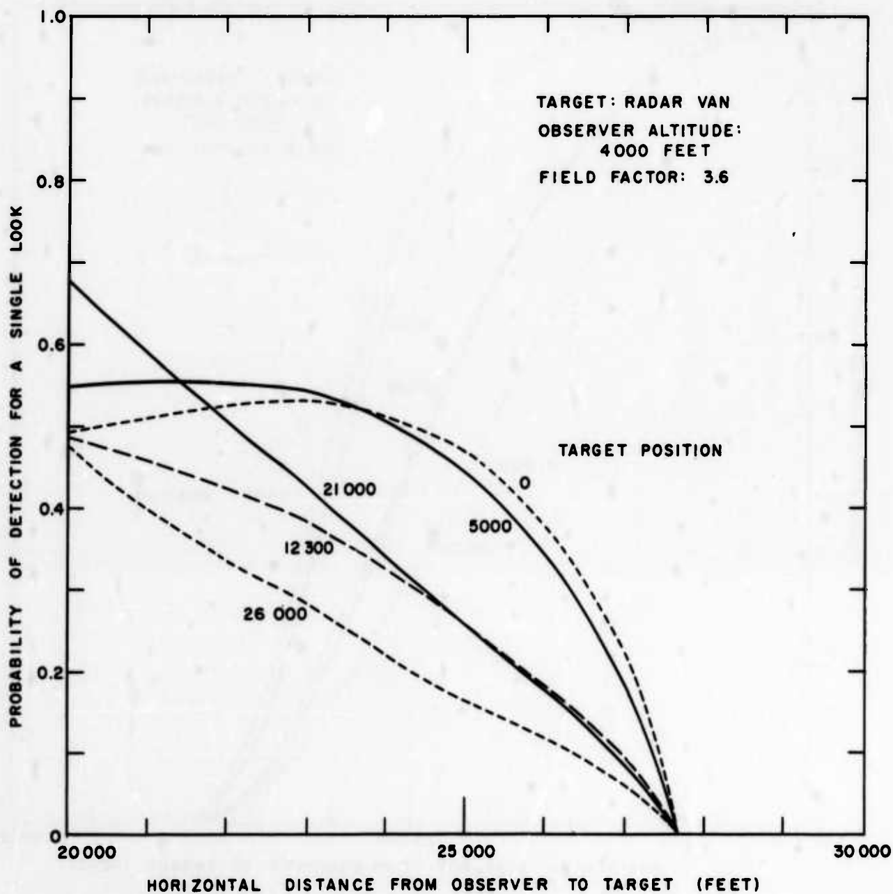
FIGURE 33 - PROBABILITIES FOR ONE LOOK FOR SYSTEMATIC SEARCH AS A FUNCTION OF OBSERVER-TO-TARGET DISTANCE AND TARGET POSITION
