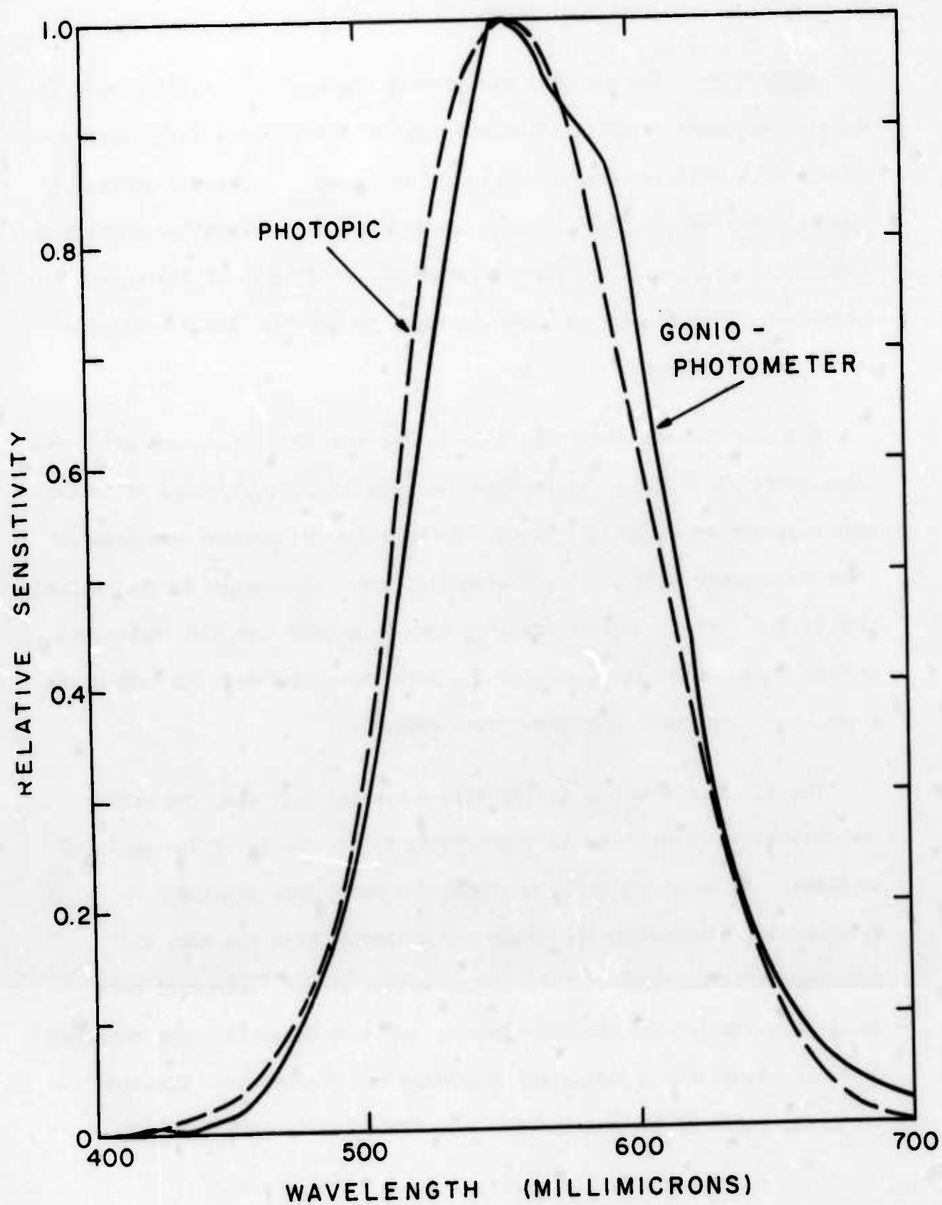
FIGURE 18- RELATIVE SPECTRAL SENSITIVITY OF GONIOPHOTOMETER
