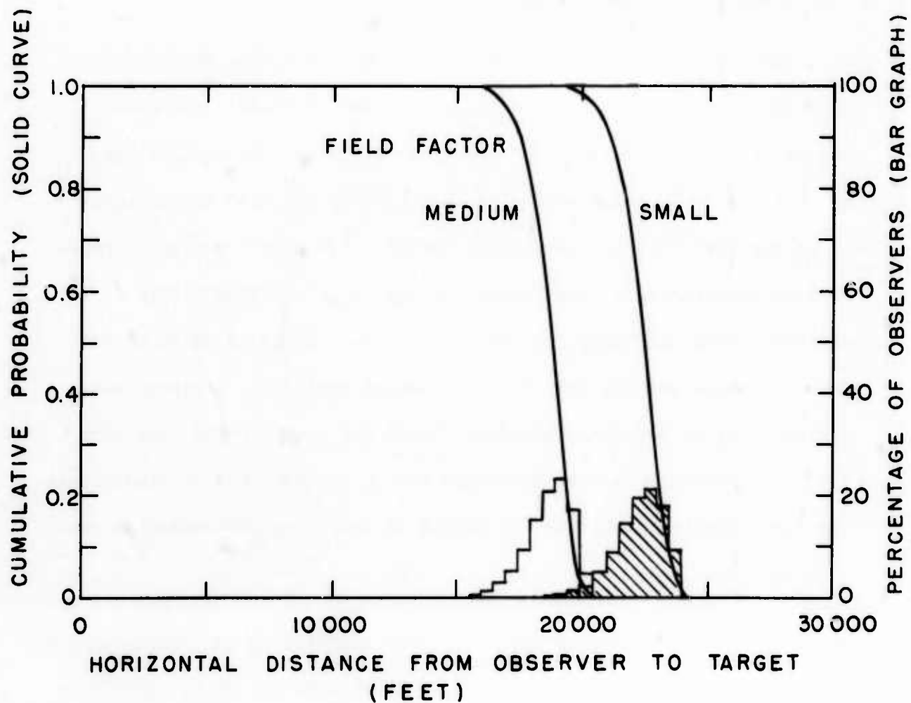
FIGURE 14-CUMULATIVE PROBABILITY CURVES AND NORMAL DISTRIBUTION BAR GRAPHS FOR SIGHTINGS OF THE RADAR VAN BY THE OBSERVER AT AN ALTITUDE OF 1000 FEET
