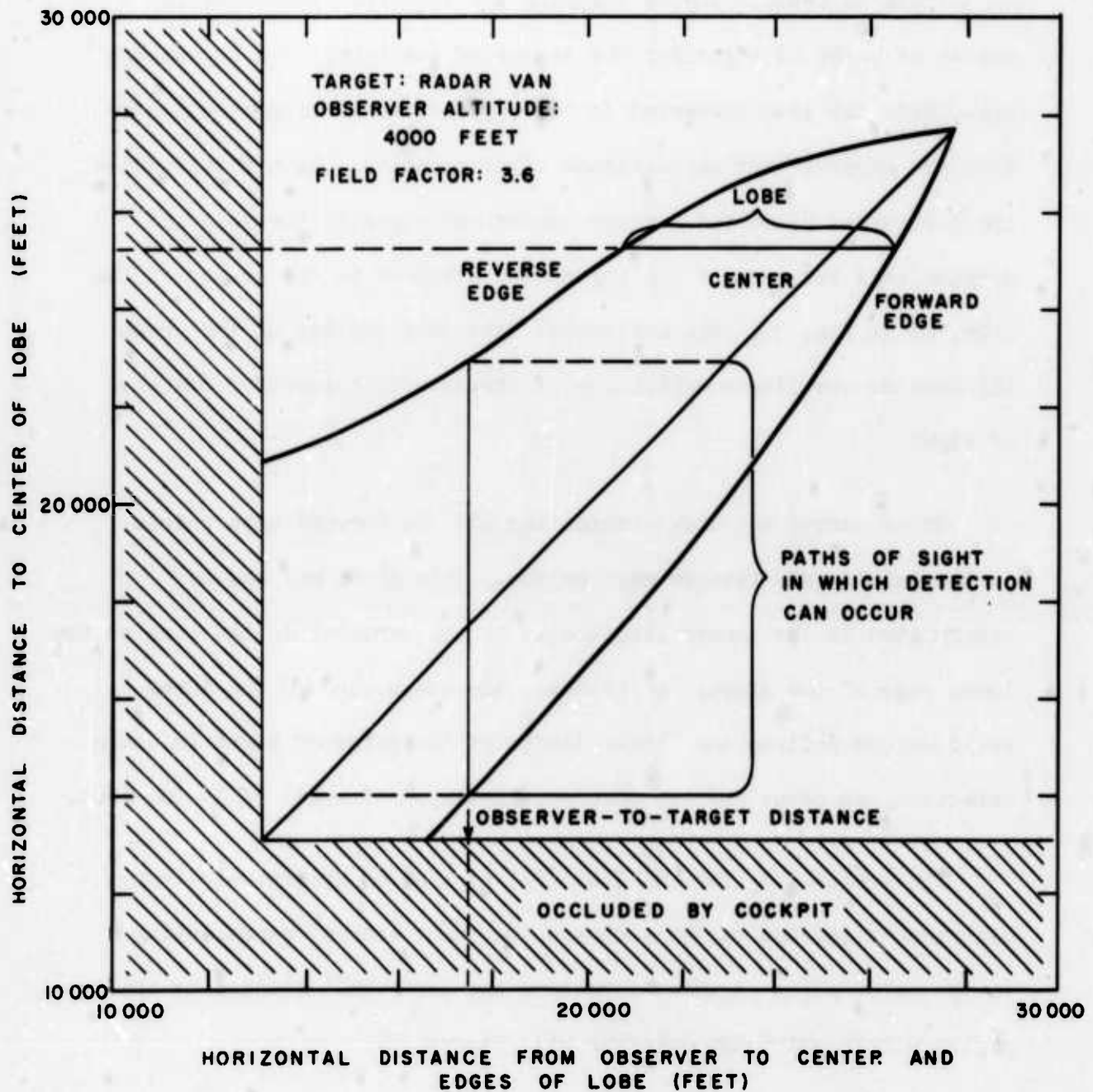
FIGURE 30 - LINEAR DEFINITION OF THE DETECTION LOBE, AND THE PATHS OF SIGHT APPROPRIATE TO DETECTION AT A GIVEN OBSERVER-TO-TARGET DISTANCE
