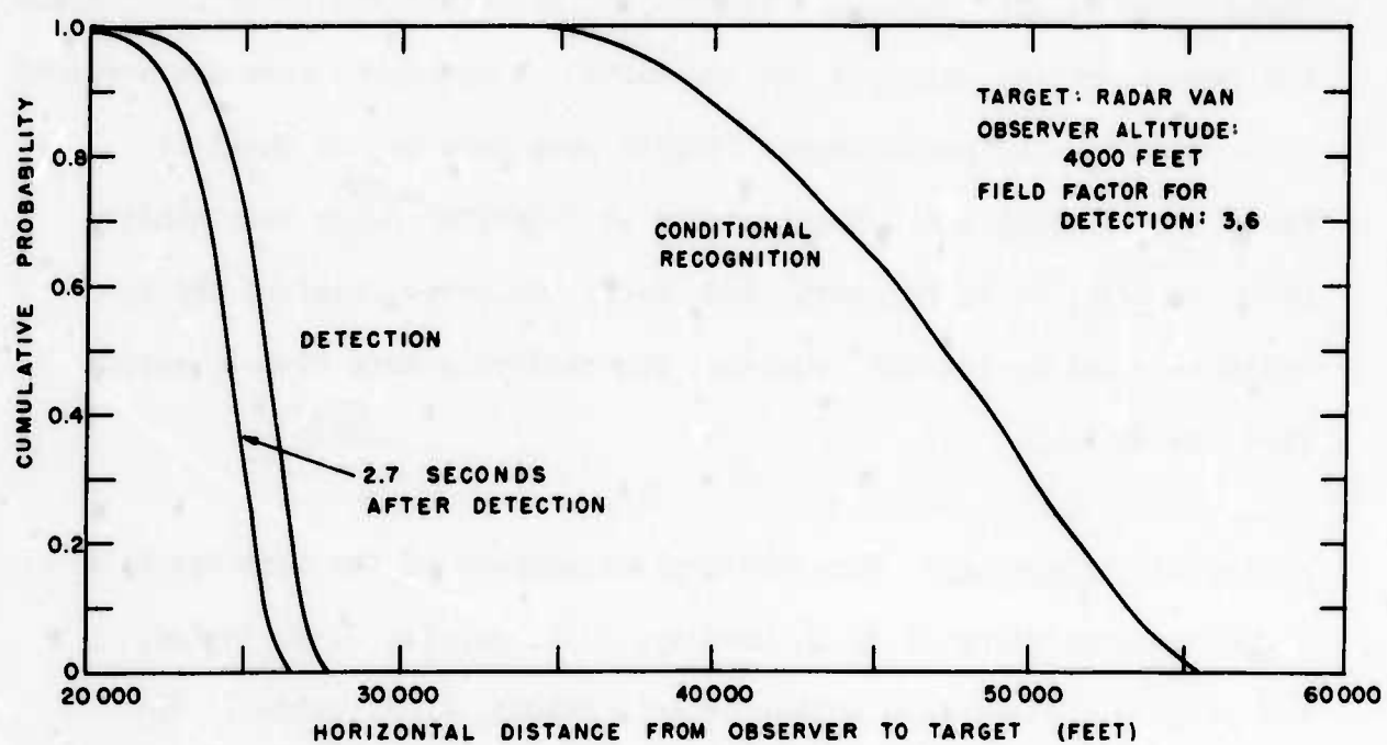
FIGURE 37 - TYPICAL RELATIONSHIP BETWEEN PROBABILITIES OF DETECTION AND CONDITIONAL RECOGNITION
