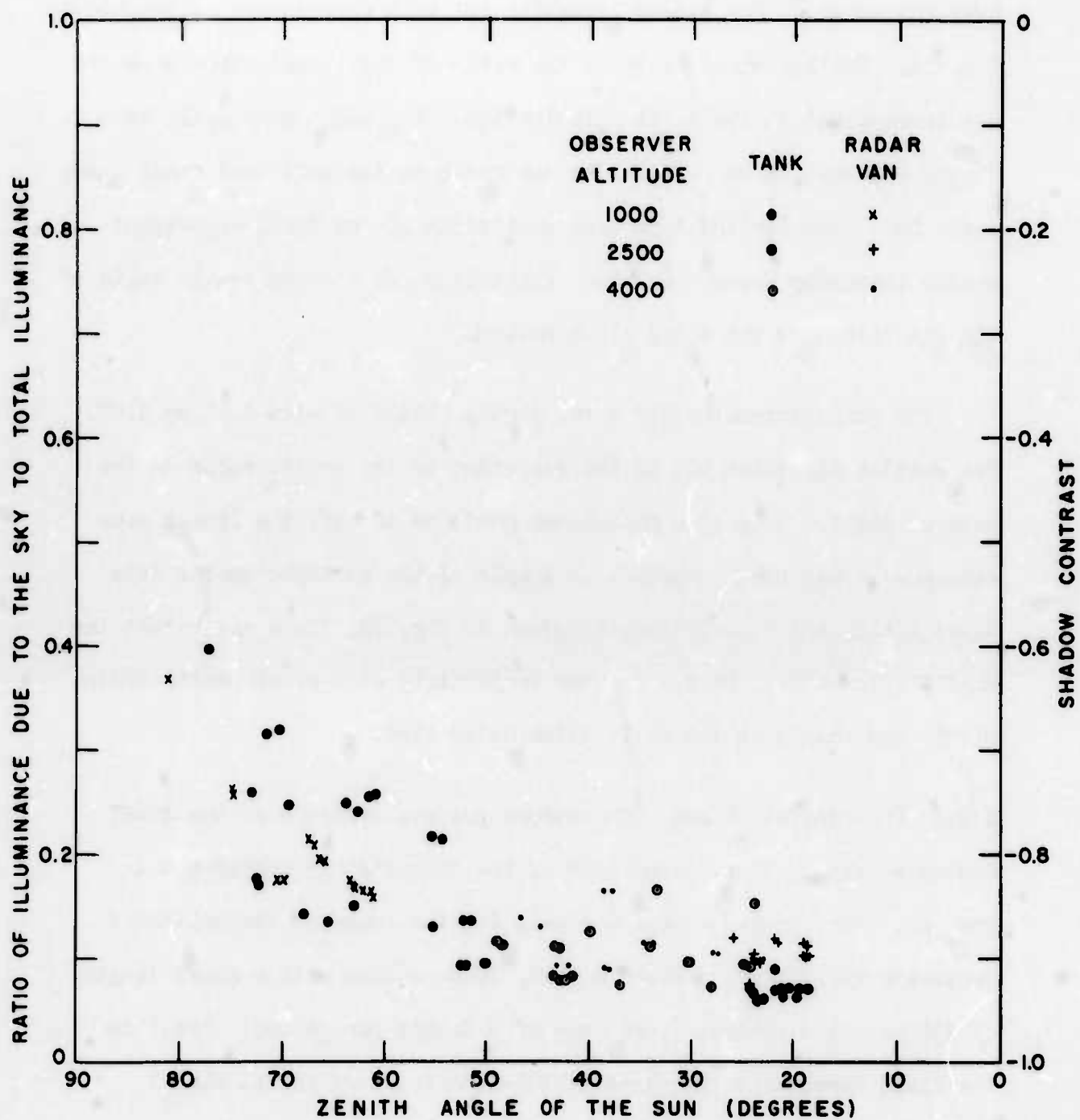
FIGURE 21 -- SHADOW INTENSITY DURING SIGHTINGS
