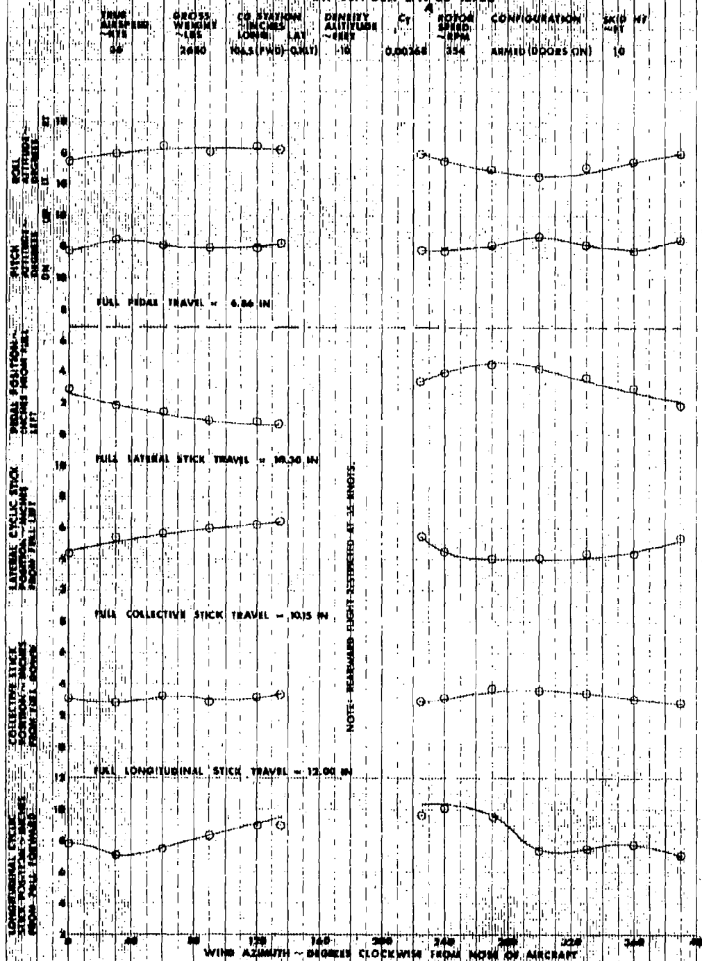
FIGURE 49 CONTROL POSITIONS VERSUS RELATIVE WIND AZIMUTH OH-13A USA S/N 68-16786
