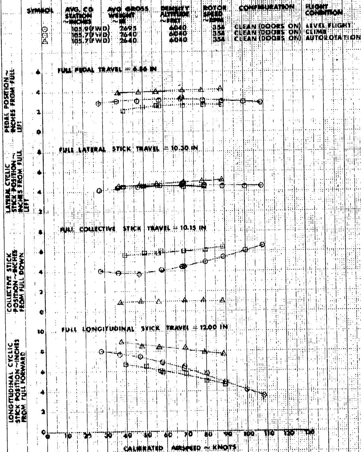
FIGURE 18 CONTROL POSITIONS IN FORWARD FLIGHT OH-5A USA S/N 68-16704
