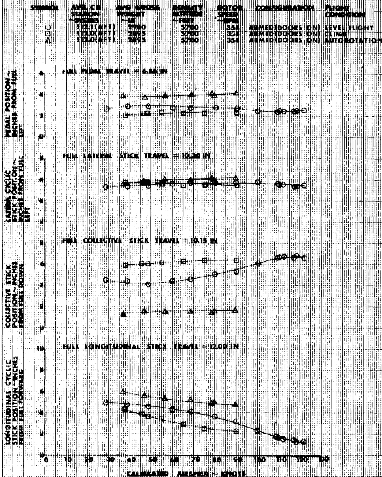
FIGURE 12 CONTROL POSITIONS IN POWERED FLIGHT G4-58A USA 574 68-16766
