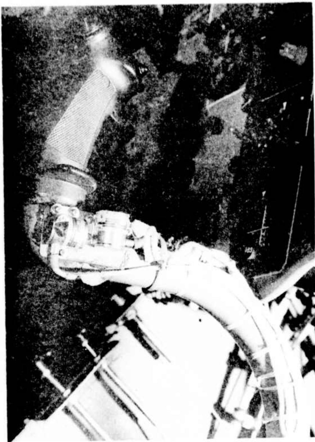
Photo 9. Vertical and Longitudinal Accelerometer Installation - Pilot's Cyclic
