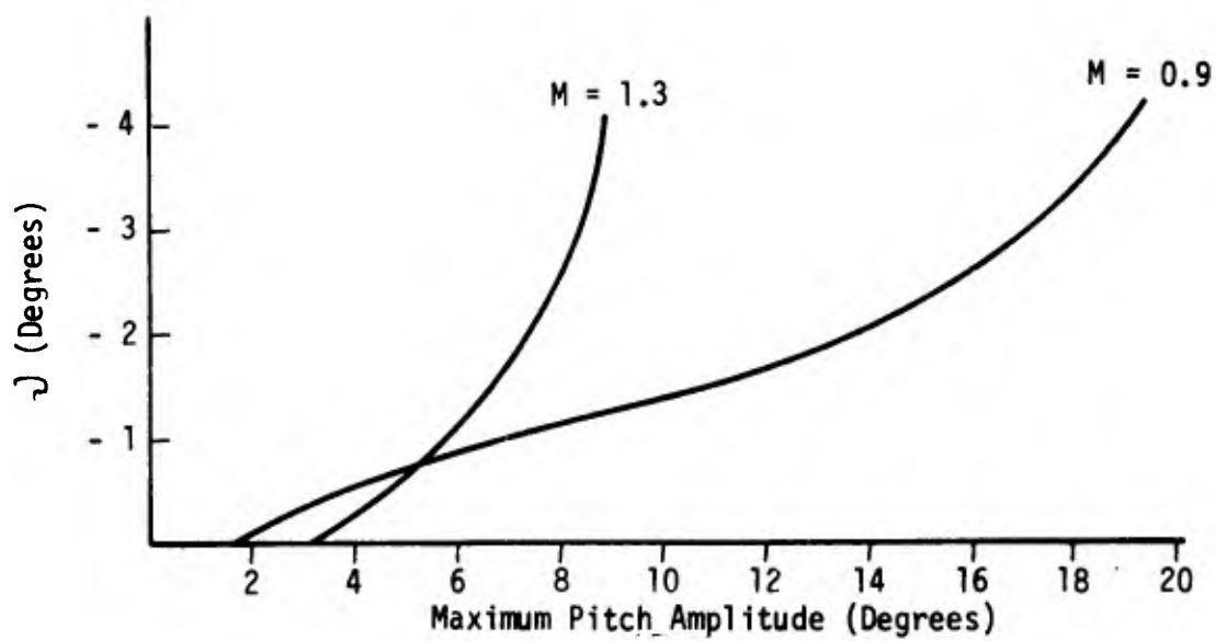
Figure 9. \delta Versus Maximum Pitch Amplitude (Nominal X_{cg} Position)
