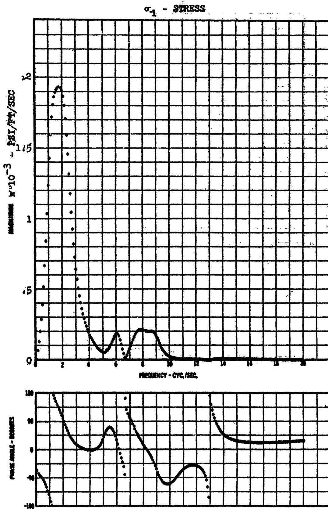
Figure B-4. Illustrative Frequency Response Function for B-57 Airplane (from reference 6)
