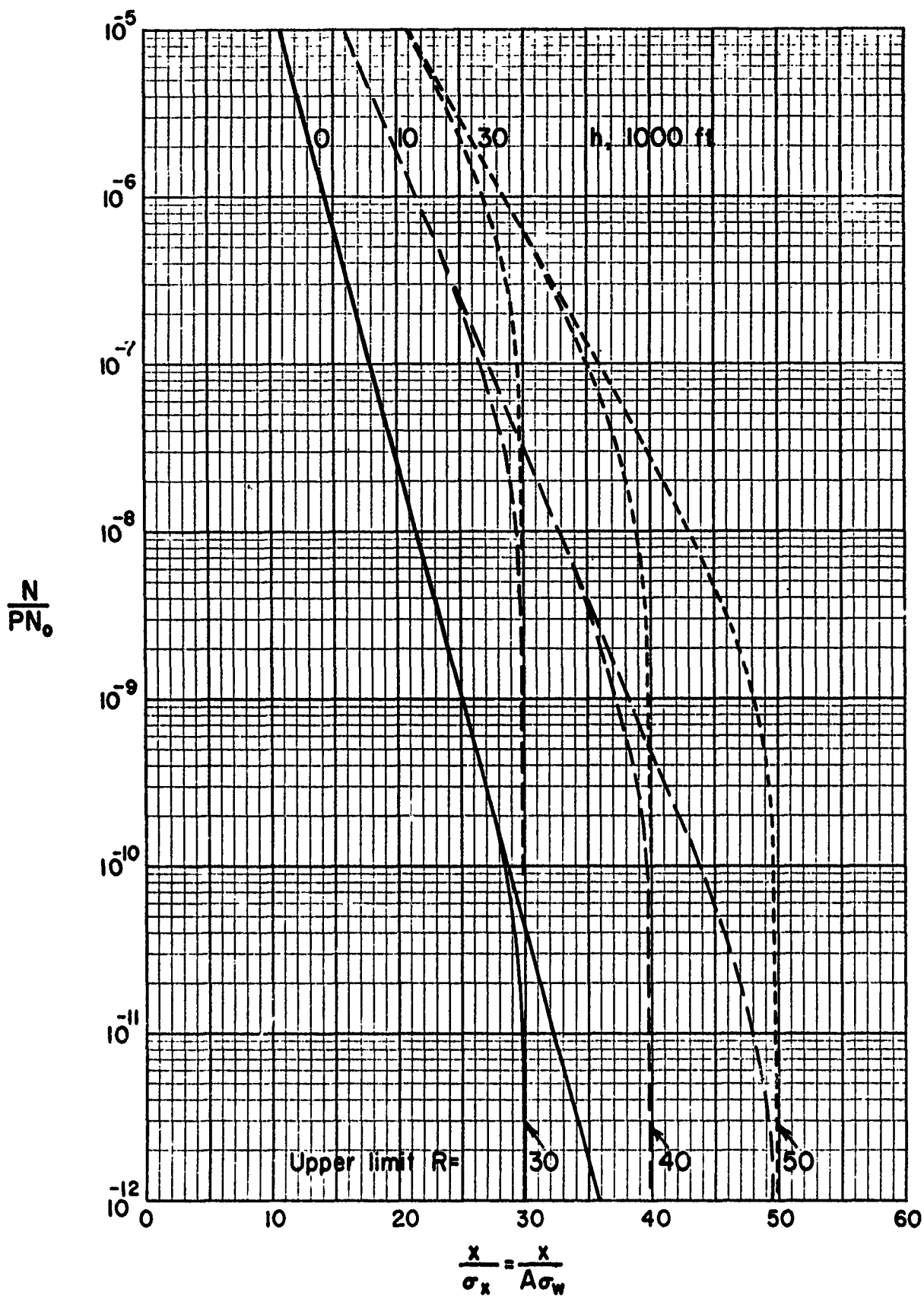
Figure 42. Effect of Bounded Joint Distribution on Exceedance Curves
