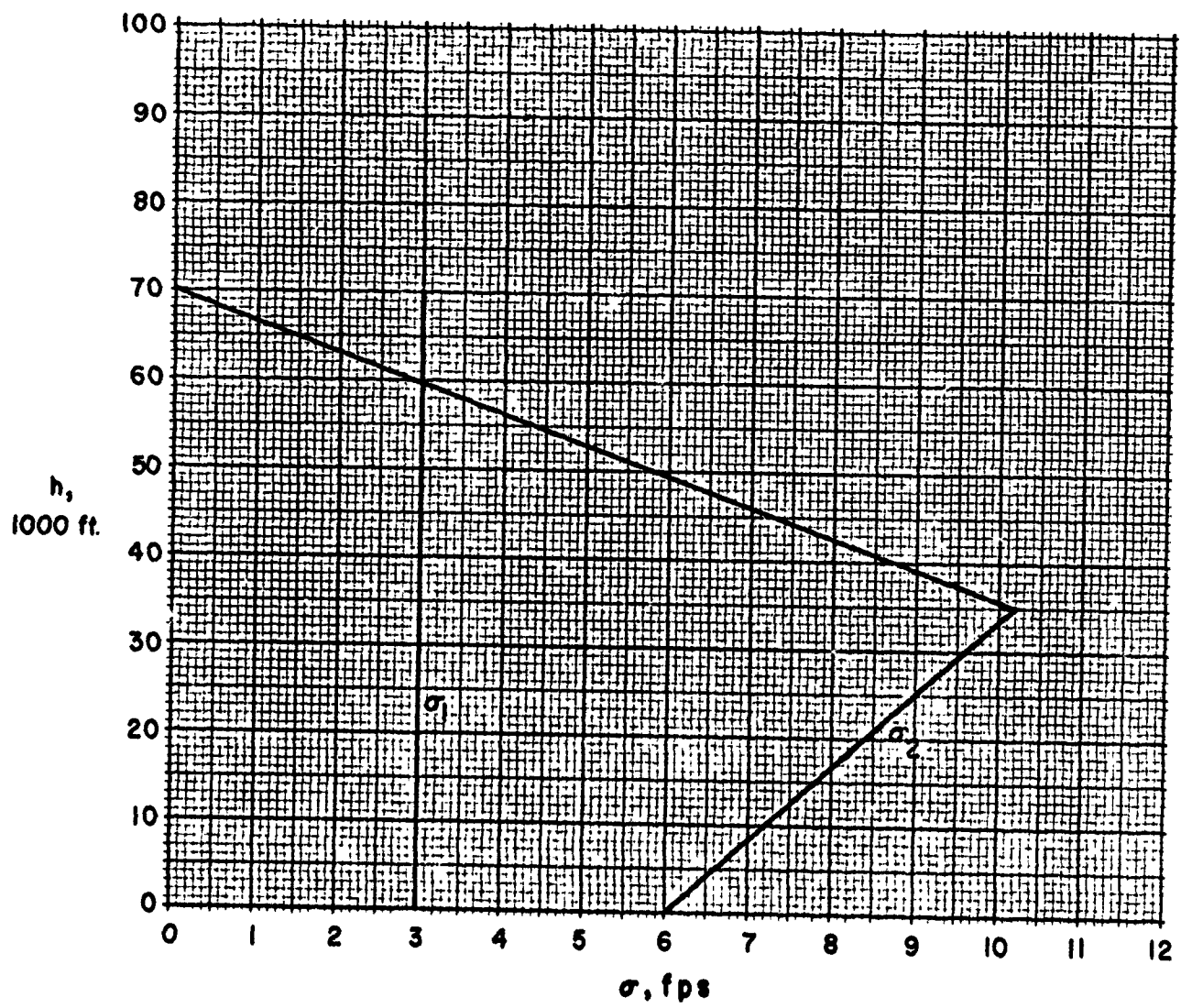
Figure 34. \sigma Values for Case (b)
