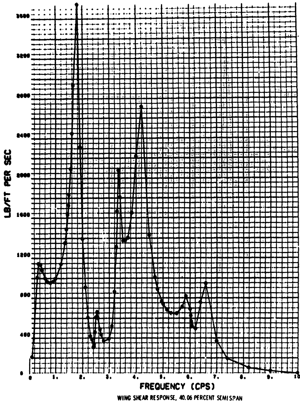
Figure B-2. Illustrative Frequency Response Function for Wing Shear for KC-135 Airplane (from reference 7)
