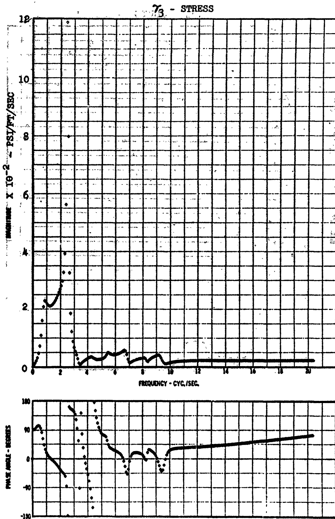
Figure B-3. Illustrative Frequency Response Function for B-58 Airplane (from reference 6)
