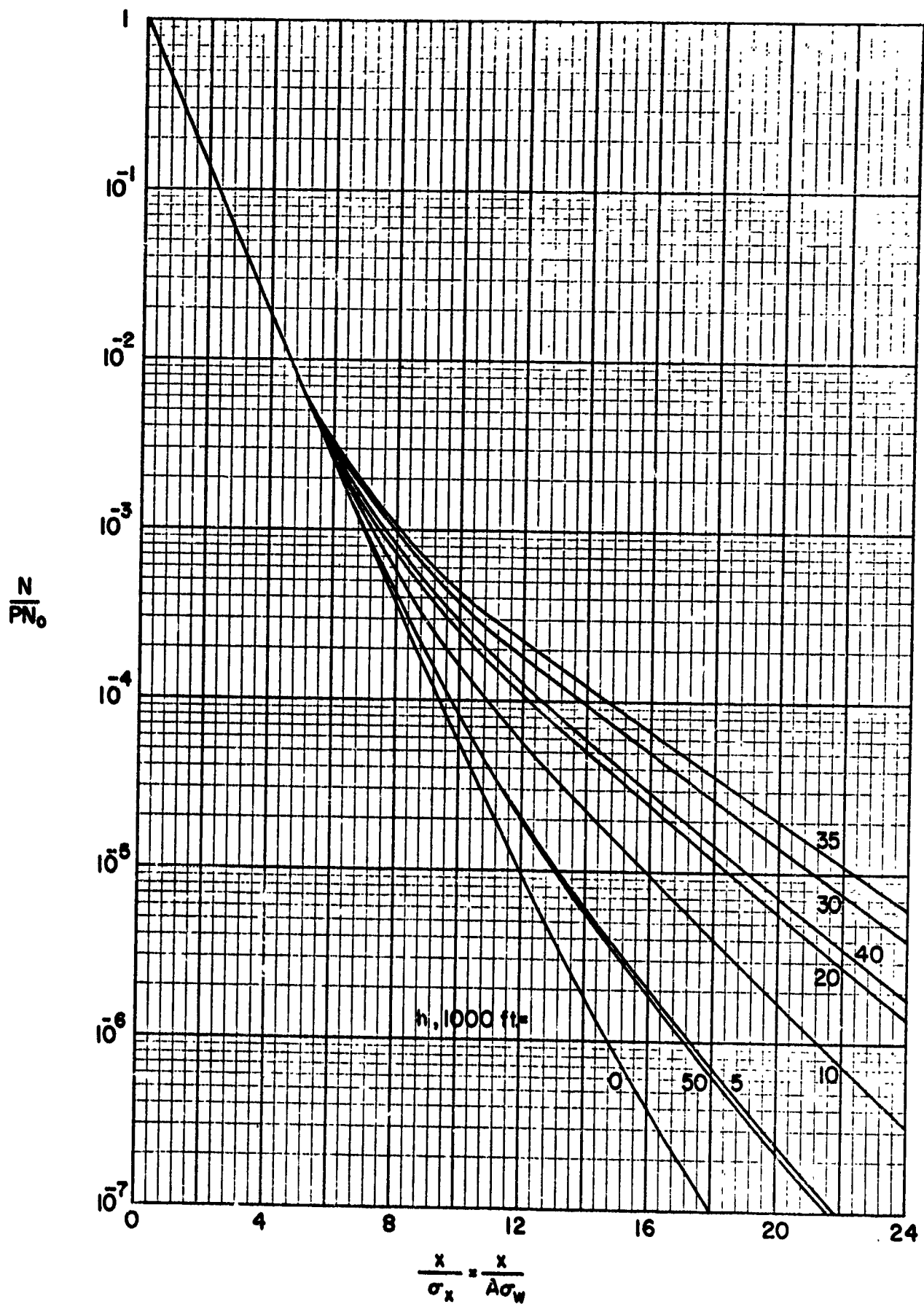
Figure 30. Generalized Exceedance Curves for Case (a)
