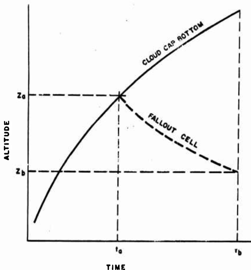
Figure 3.1 Time-Altitude Relationship of the Cloud Cap Bottom and a Fallout Parcel Trajectory
