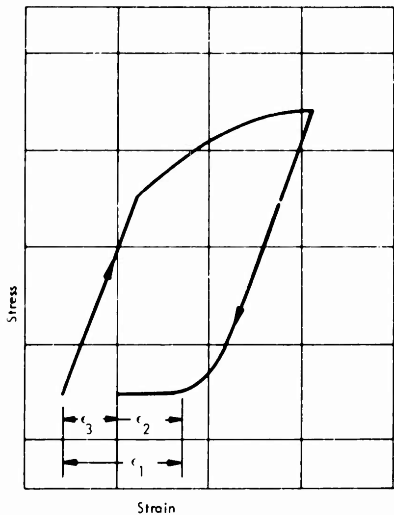
Figure 7. Viscoelastic Strain Parameters.
