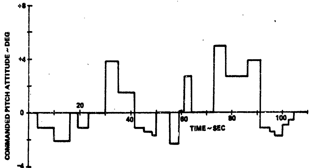
Figure 12. Discrete-Error Pitch-Attitude Command Signal
