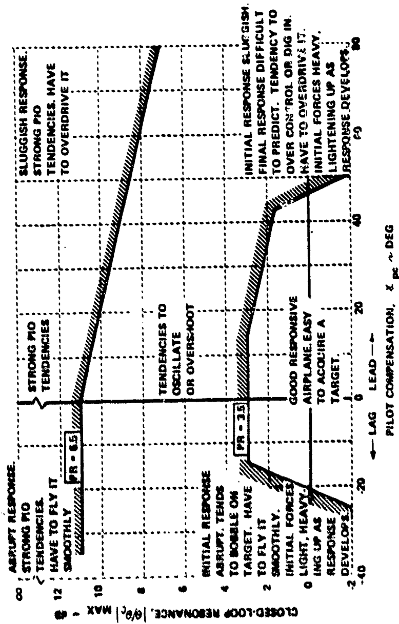
Figure 50. Proposed Criterion for Fighter Maneuvering Dynamics
