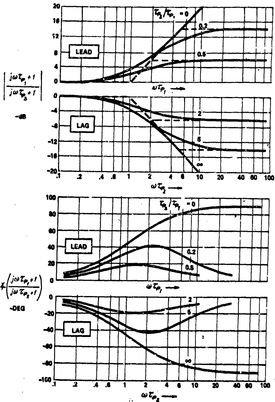
Figure 22. Amplitude and Phase Contributed by Pilot Compensation
