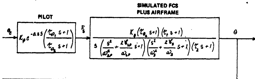
Figure 16. Mathematical Model of Pitch Attitude Tracking
