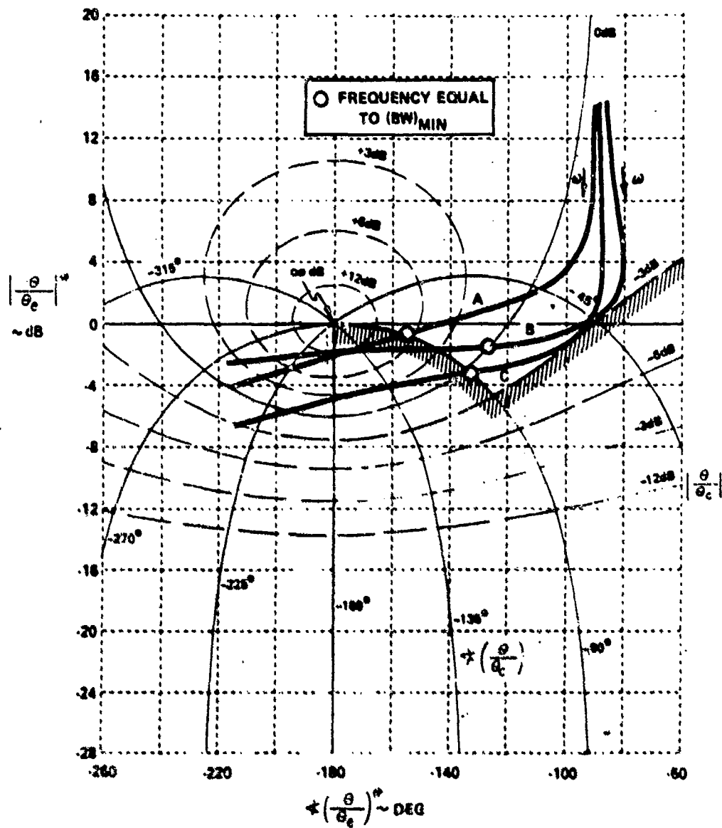
Figure 21. Typical Overlays of \left| \theta / \theta_c \right|^2 Versus \angle \left( \theta / \theta_c \right)^\circ on a Nichols Chart
