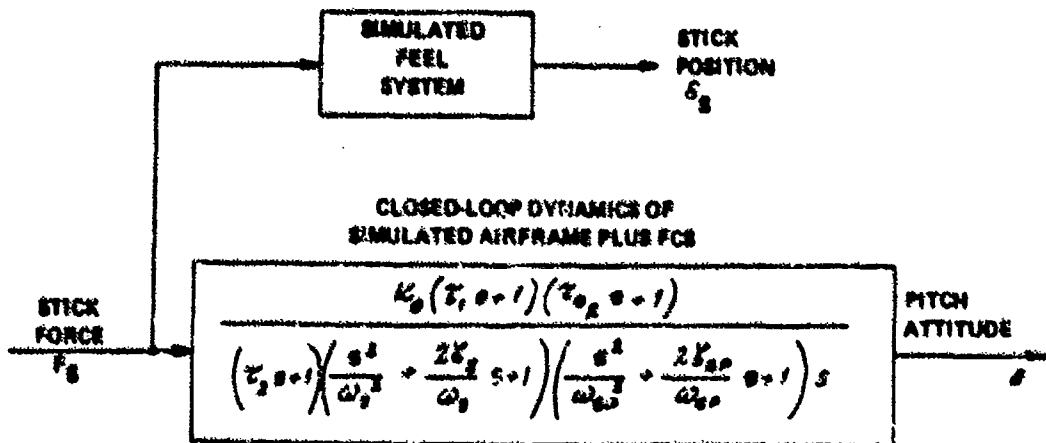
Figure 3. Block Diagram for Basic Configurations Simulated
