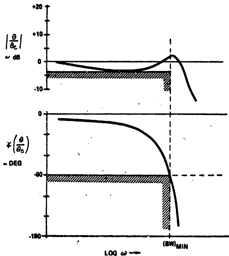
Figure 19. Tracking Performance Standards Used in the Analysis.
