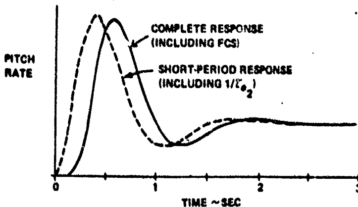
Figure 2. Pitch-Rate Response to a Step Stick-Force Input for HOS Configuration of Figure 1.
