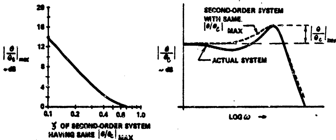
Figure 37. Damping Ratio of Simple Second-Order System as a Function of \left| \theta / \theta_c \right|_{\max}
