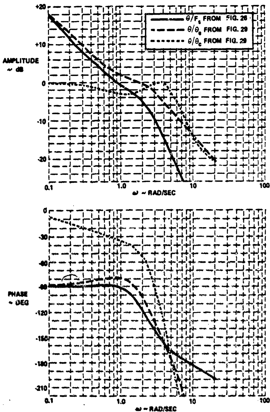
Figure 30. Open-Loop and Closed-Loop Bode Plots for Configuration with Low \omega_{np}
