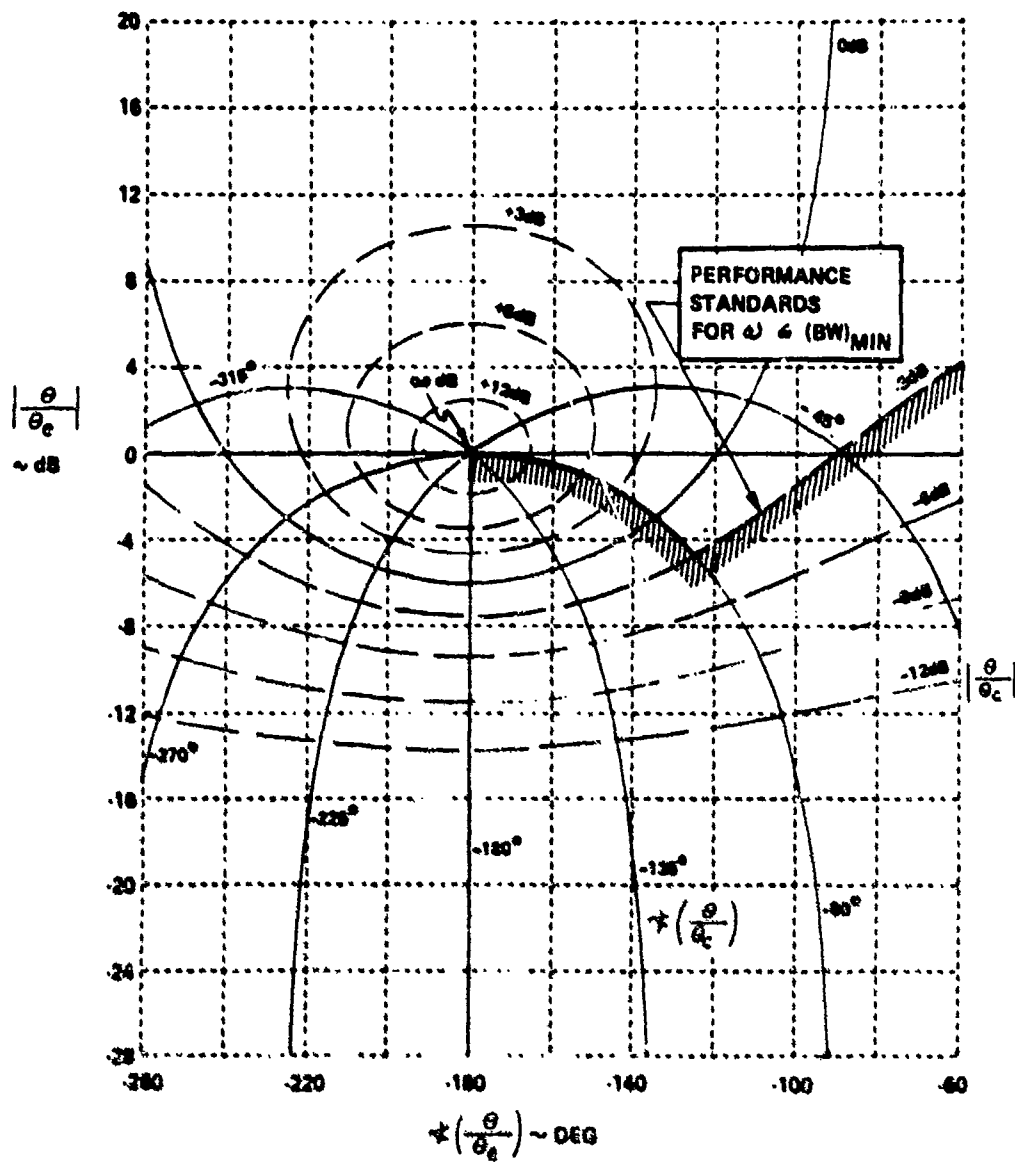
Figure 20. Nichols Chart Showing Performance Standards Used in the Analysis
