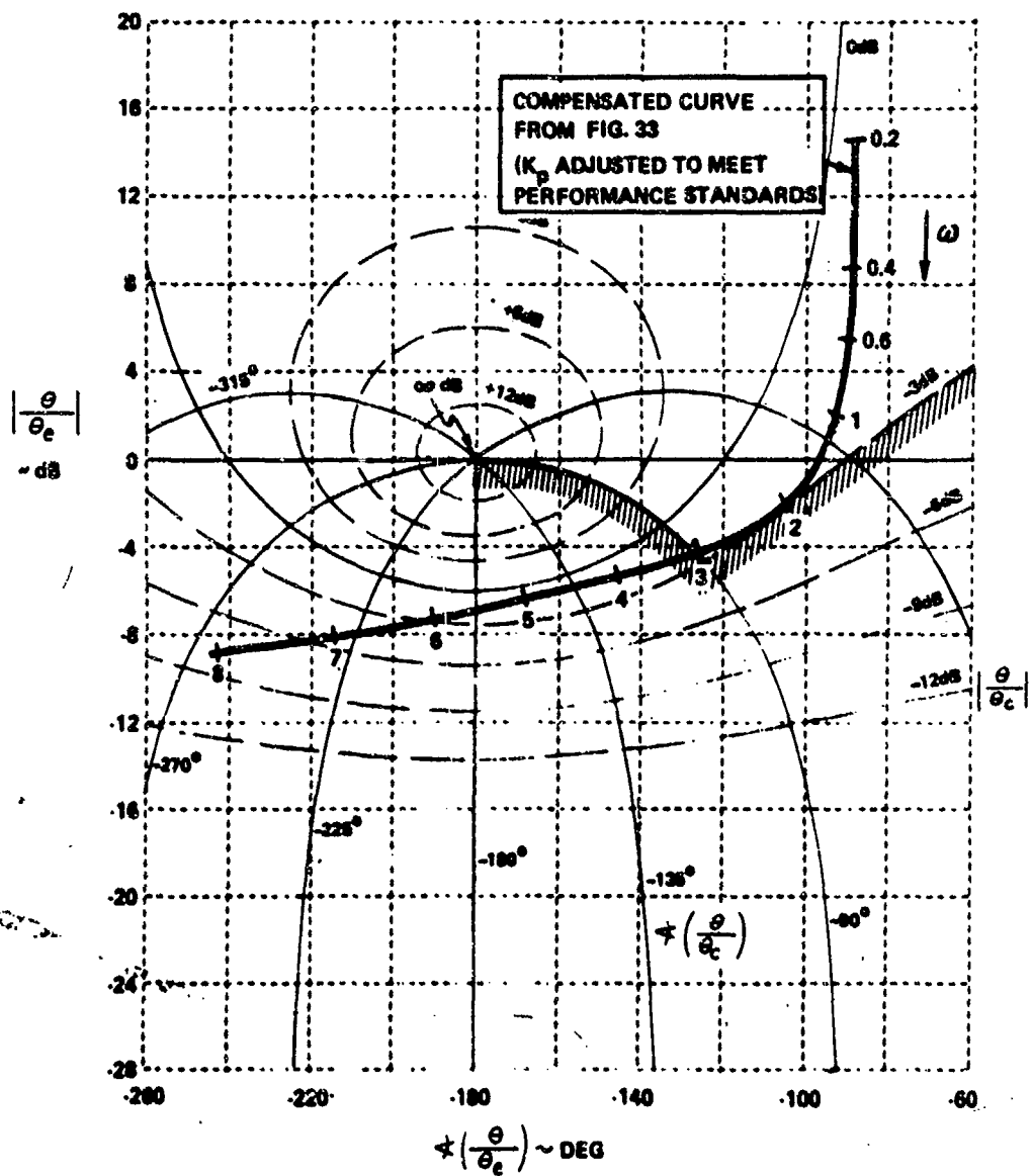
Figure 34. Lag-Compensated Amplitude-Phase Curve Overlayed on a Nichols Chart (Configuration with High \omega_{sp} )
