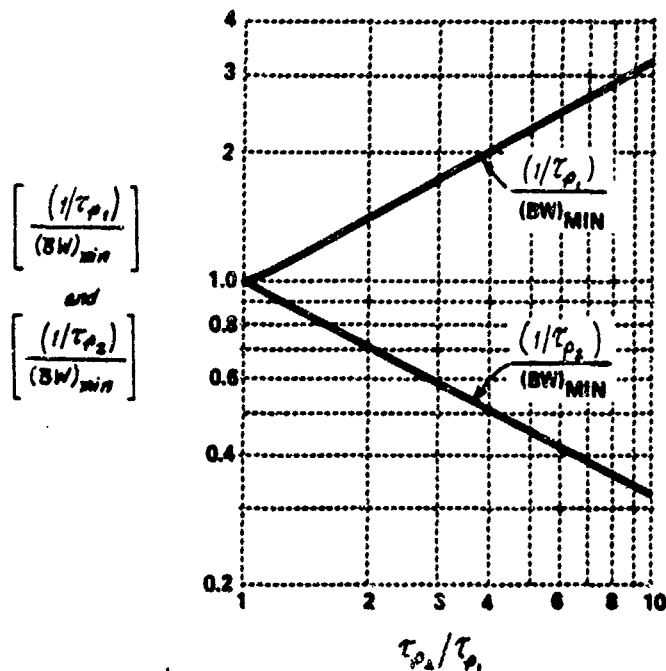
Figure 24. "Optimum" Lag Compensation
