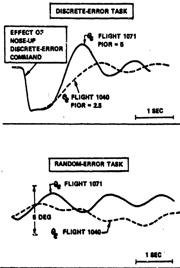
Figure 36. Typical IFR Tracking Records for Configuration 6E
