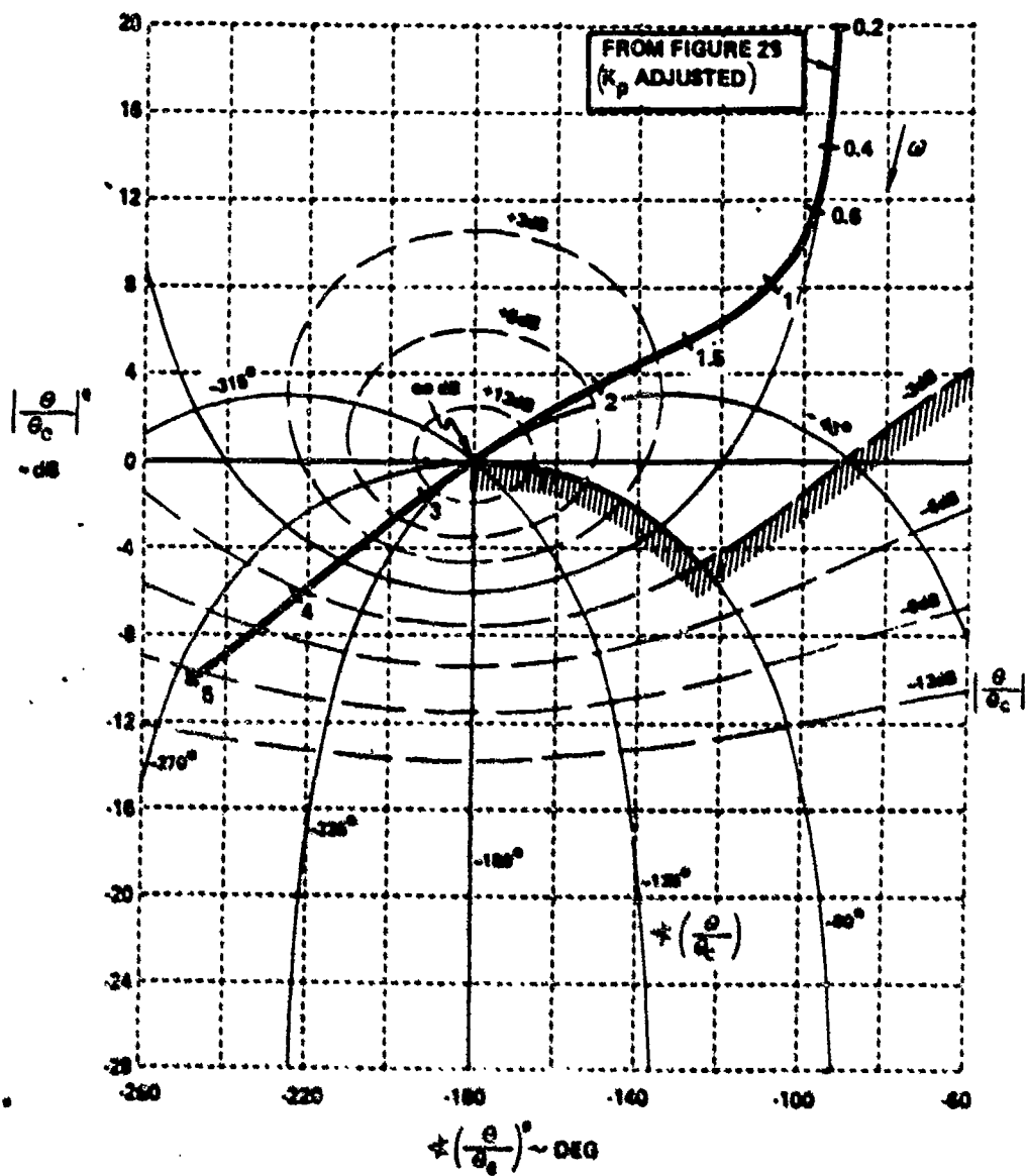
Figure 27. Overlay of |\theta/\theta_c|^2 Versus \angle(\theta/\theta_c)^\circ on a Nichols Chart (Configuration with Low \omega_{zp} )
