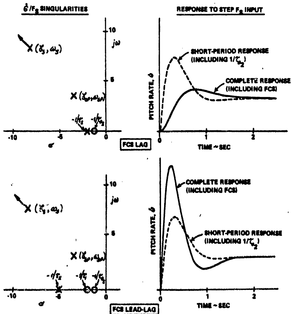
Figure 6. Typical s-Plane Plots and Time Histories for Present Experiment
