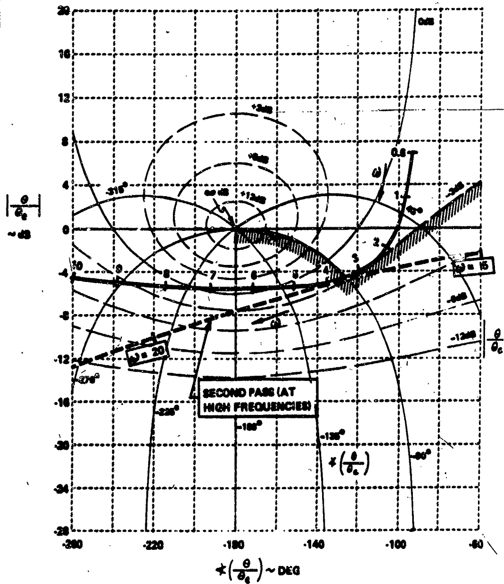
Figure 42. Compensated Amplitude-Phase Plot for Configuration 14, Showing the Cause of the High Frequency Resonance
