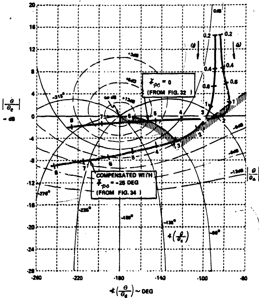
Figure 39. Effects of Removing Pilot Lag Compensation for Configuration 3A (at Constant K_p )
