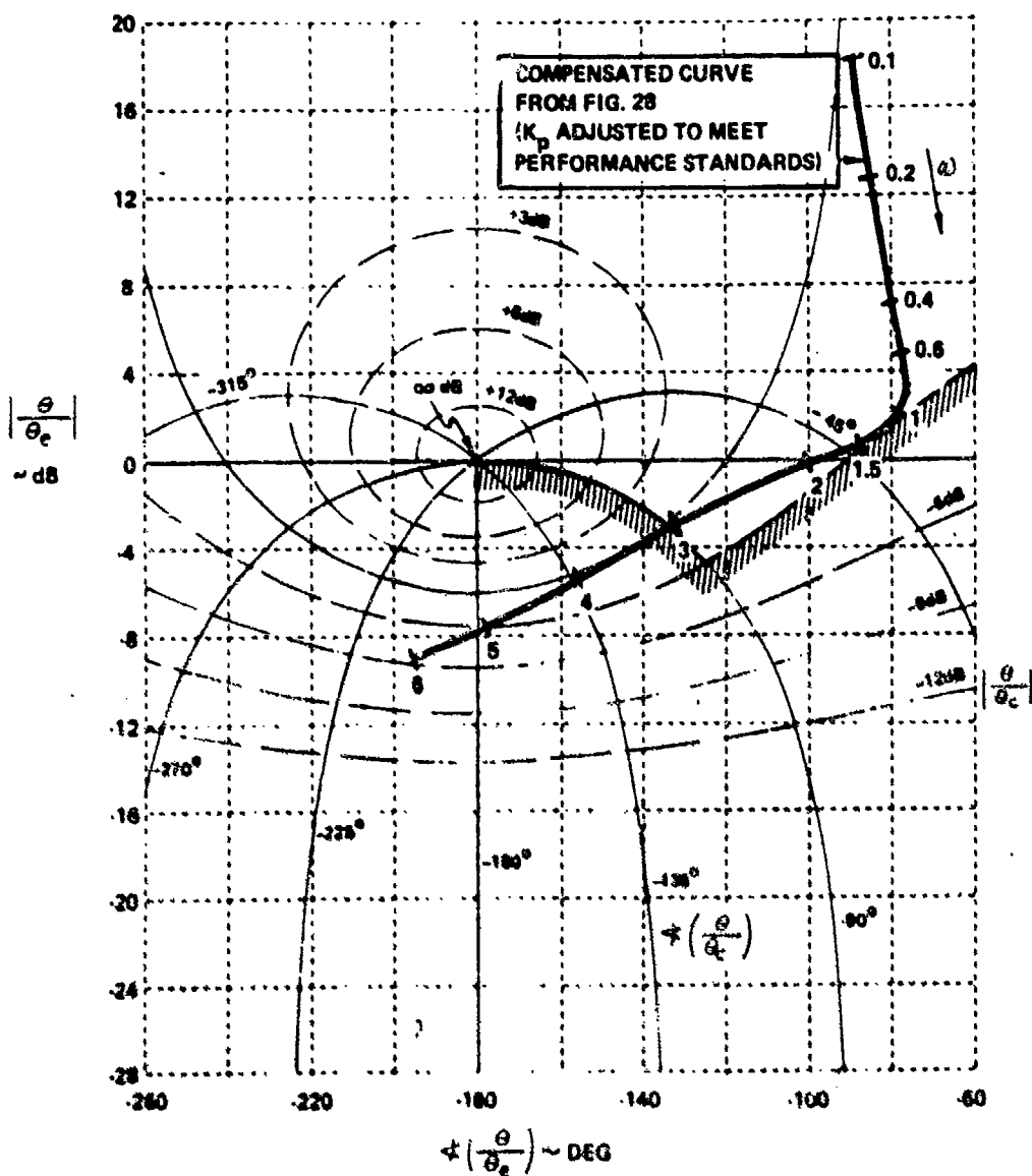
Figure 29. Lead-Compensated Amplitude-Phase Curve Overlaid on a Nichols Chart (Configuration with Low \omega_{sp} )
