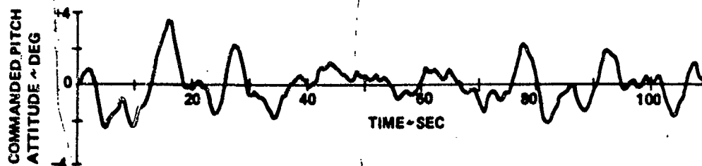
Figure 13. Random-Error Pitch-Attitude Command Signal
