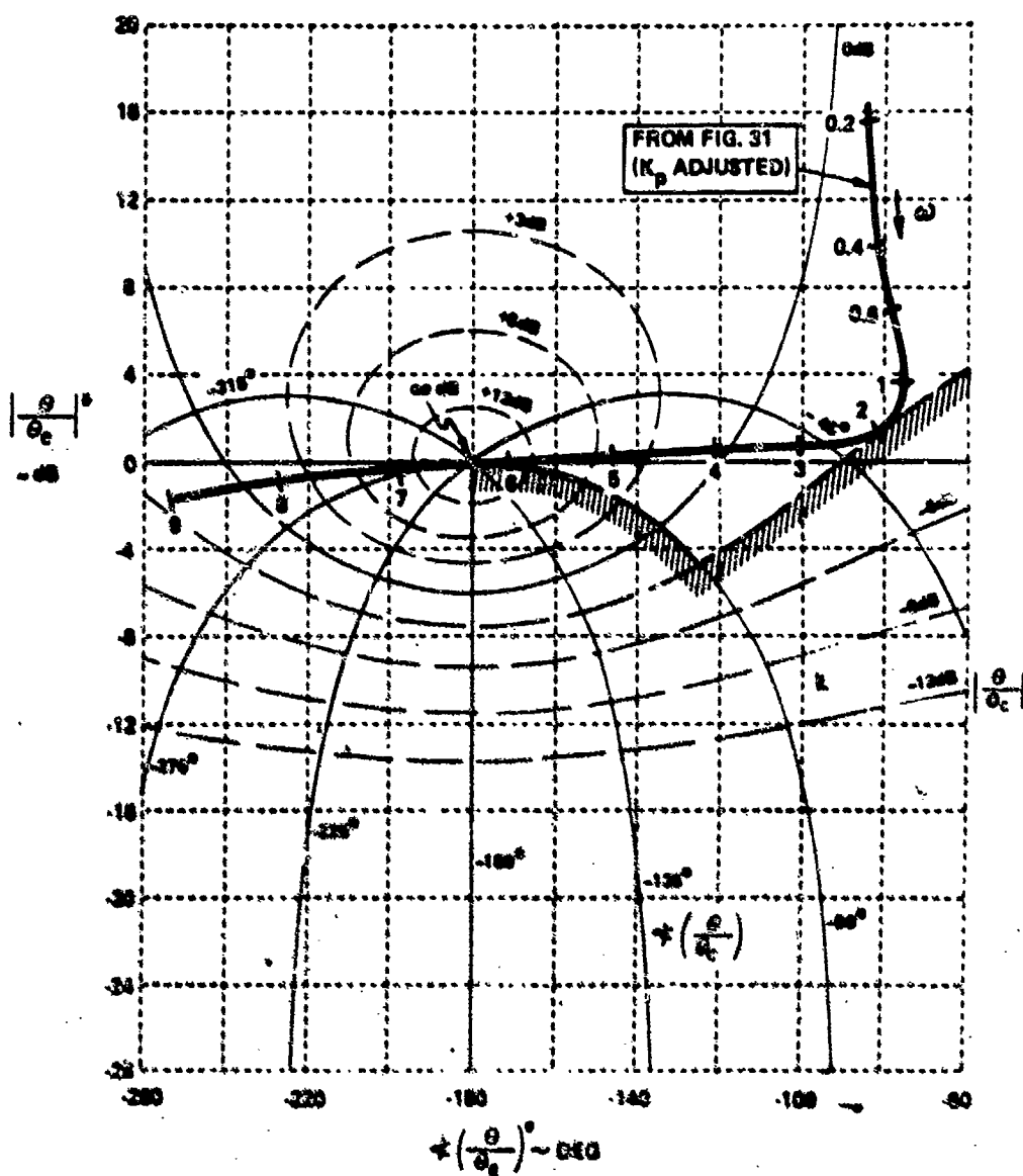
Figure 32. Overlay of \left| \theta / \theta_c \right|^2 Versus \angle \left( \theta / \theta_c \right)^\circ on a Nichols Chart (Configuration with High \omega_{3r} )
