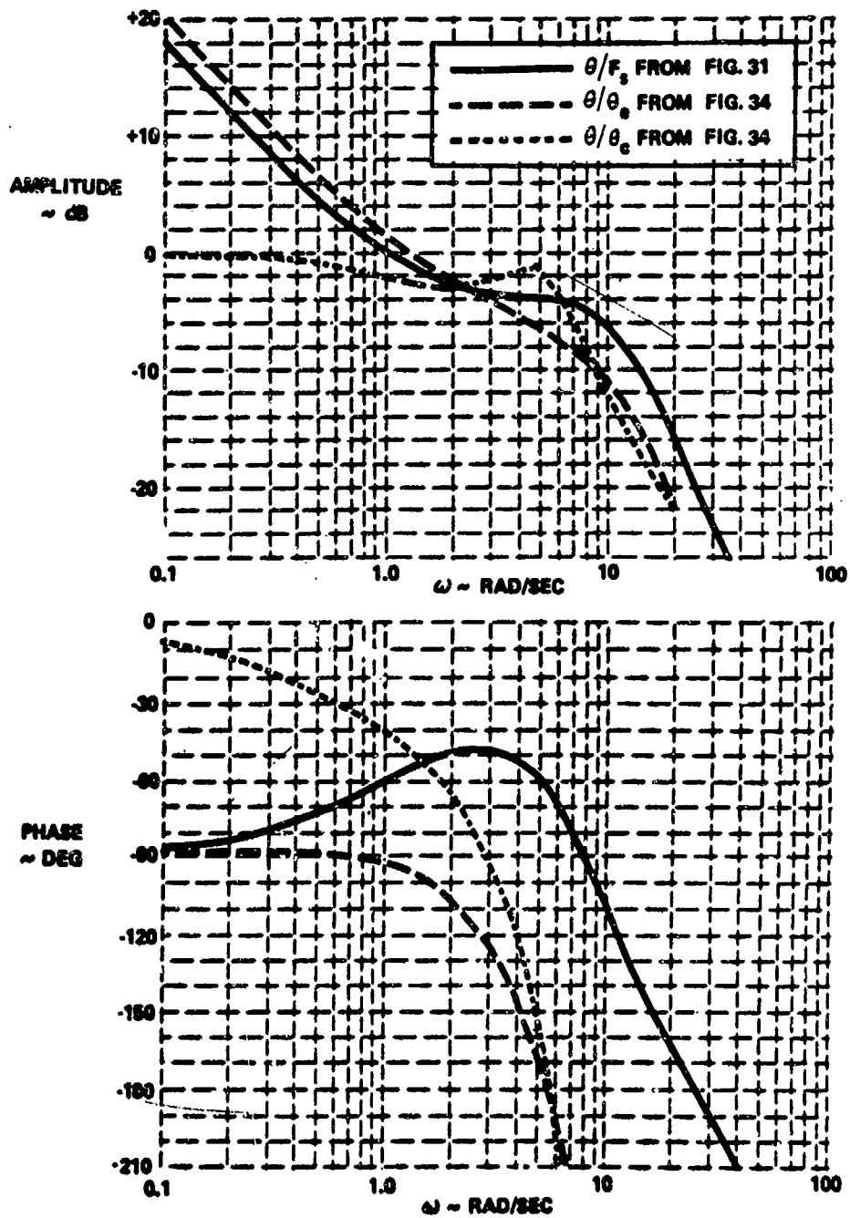
Figure 35. Open-Loop and Closed-Loop Bode Plots for Configuration with High \omega_{sp}
