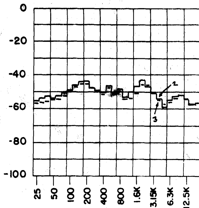
FIGURE 51. THIRD-OCTAVE-BAND SPECTRA — CAVITY WITH ONE STORE (1), WITH TWO STORES (2); M = 1.5 ; L/D = 5.7 ; P_0 = 10 psia; MICROPHONES #2, #3.
