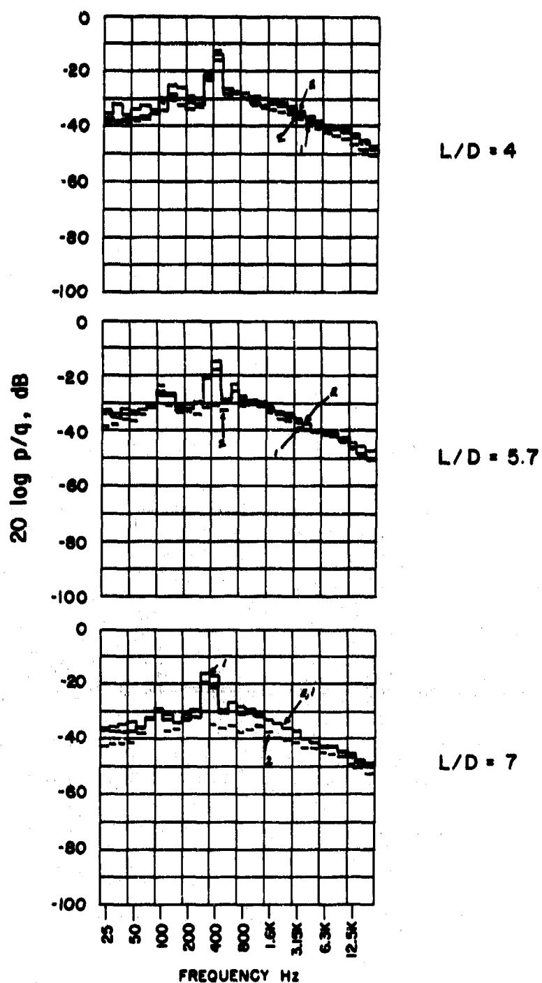
FIGURE 41. THIRD-OCTAVE-BAND SPECTRA — EMPTY CAVITY (E); CAVITY WITH ONE STORE (1), WITH TWO STORES (2); M = 0.8 ; P_0 = 10 psia; MICROPHONE #6.
