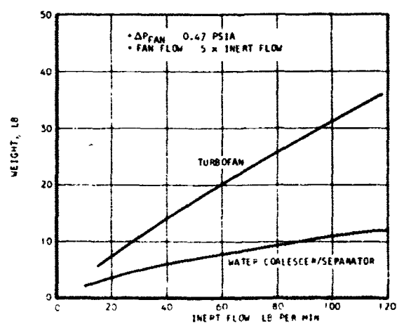
Figure 46. Turbofan and Water Separator Weight
