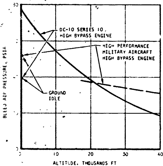
Figure 57. Typical High Bypass Engine Bleed Data
