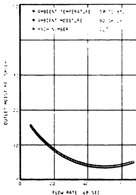
Figure 60. Inerting System Outlet Moisture Content Insensitivity to Ambient Humidity
