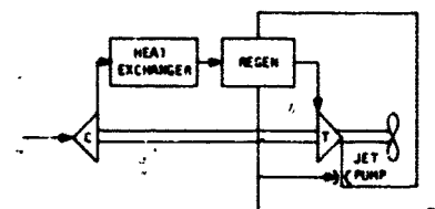
C. WITH REGENERATOR WITH RECIRCULATION LOOP
